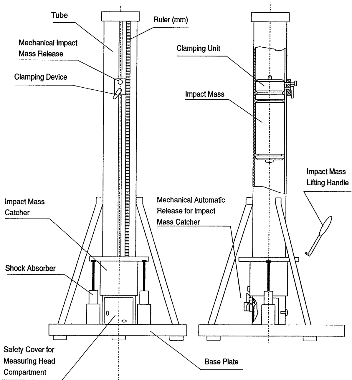
Figure 120. AVL calibrator.
