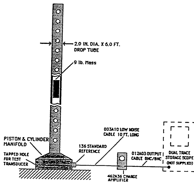
Figure 115. Modern drop-test calibrator.
