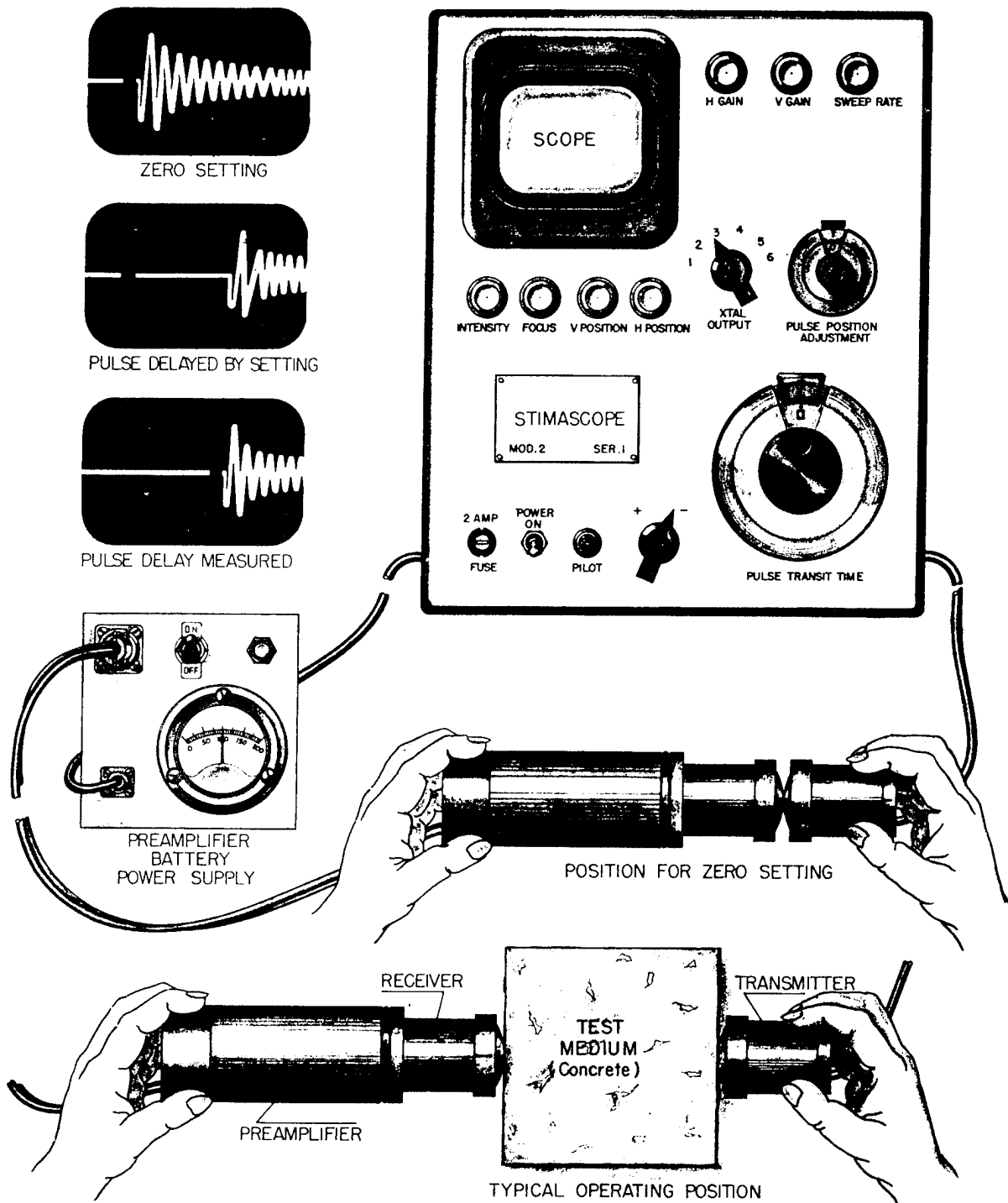
Figure 44. Use of Stimascope.
