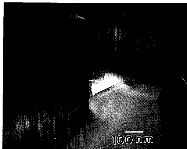
Fig. 10. Cavity formed at whisker/matrix boundary. Such a cavity will, under load, be propagated in an intergranular mode across the matrix.
