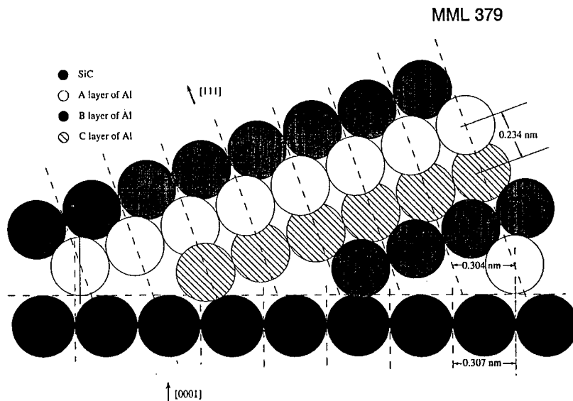
Figure 4. Schematic of the atomic packing at the (112)Al/(0001) SiC interface. The rotation of the (111)Al planes by 20° away from the interface may be necessary not only to reduce the interfacial strain but also to increase the atomic matching configuration.
