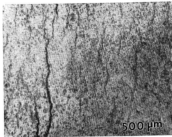
Fig. 20. Distribution of cracks on the tensile surface at 1300 °C. High stress regime. The cracks can be seen to be homogeneously distributed. There is a preponderance of small cracks.
