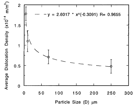
Figure 1 Average matrix dislocation density in annealed 20 V% SiC/Al composite as a function of particle size.
