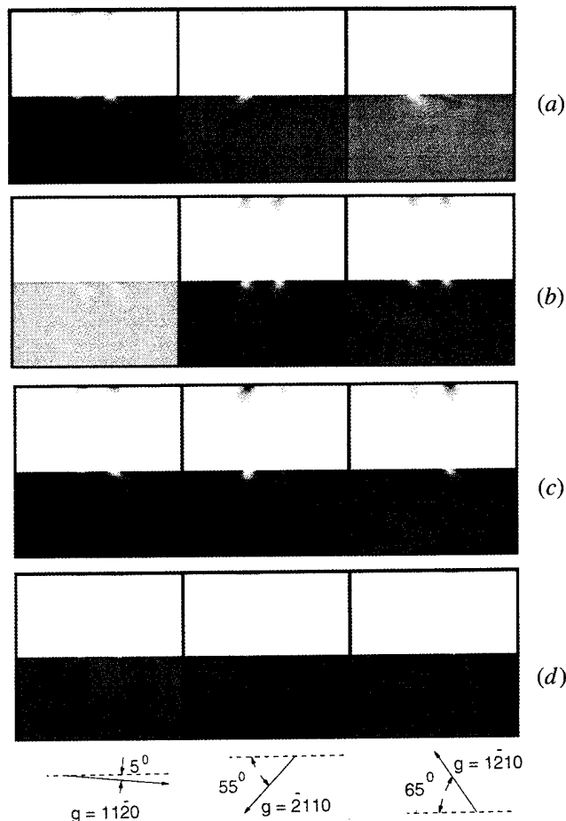
Fig. 7—Bright-field (top) and dark-field (bottom) diffraction contrast image simulations of the FEM model under different diffraction conditions, w = 1.0 and \tau = 1.3\xi_g : (a) concentrate shear load; (b) concentrate normal load; (c) both shear and normal; and (d) surface traction.
