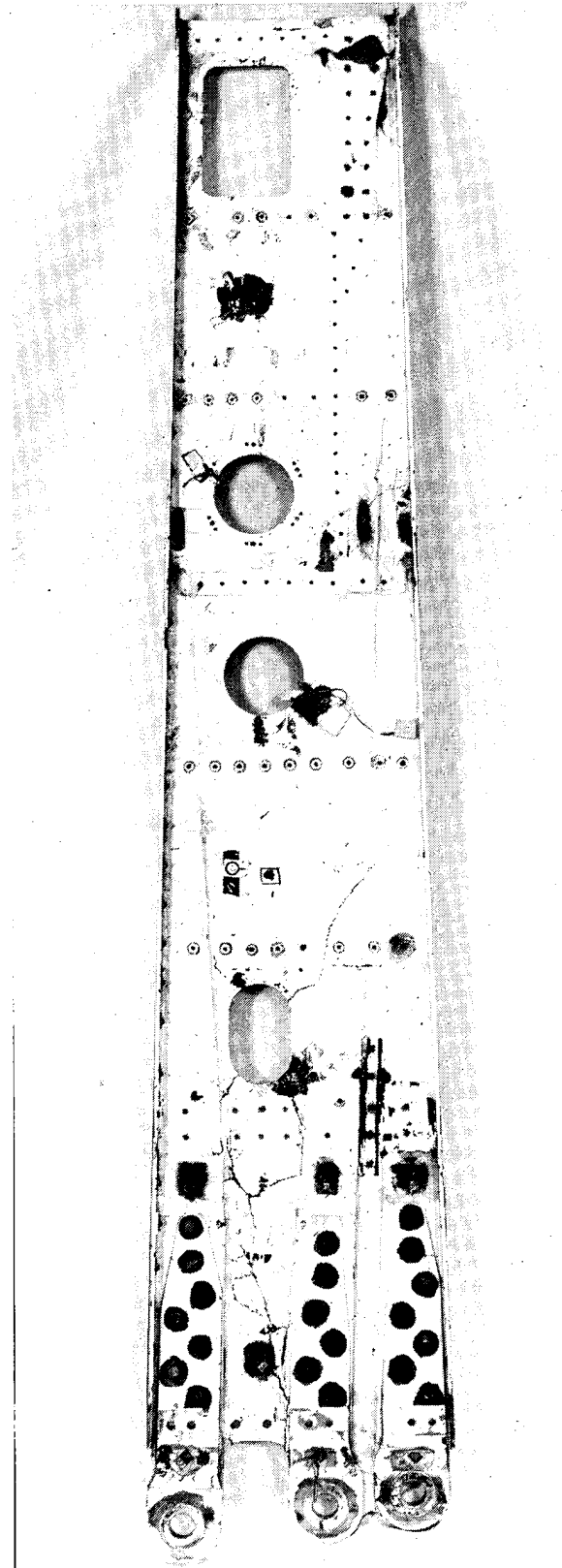
Figure 3. Rear-Spar Failure—Load Case 4010 With Upper Pin Removed
