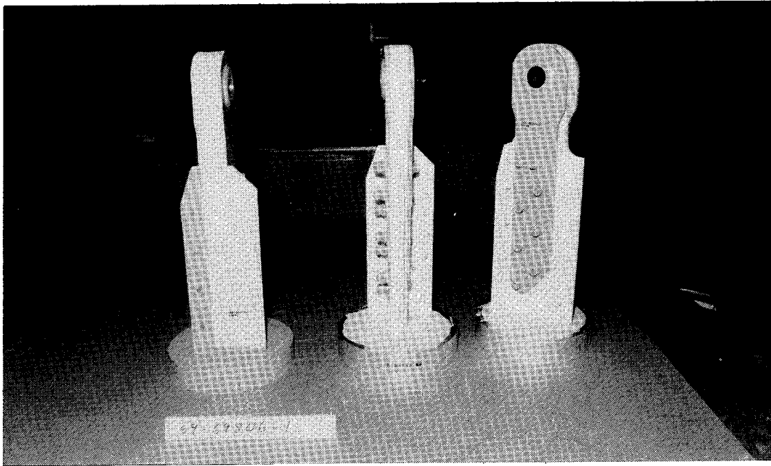
Figure 41. Spar Lug—Completed Compression Specimens
