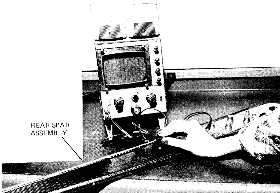
Figure 52. Sonicator Inspection of Rear-Spar Assembly
