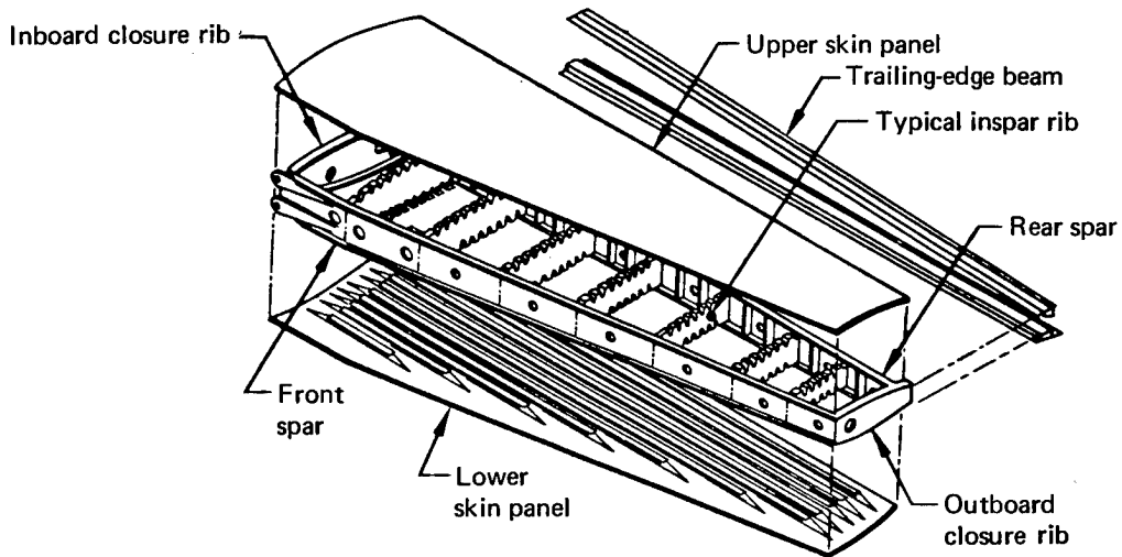
Figure 8. Stabilizer Inspar Structural Arrangement
