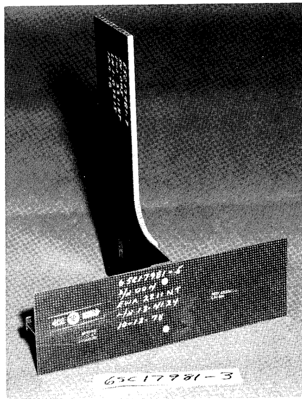
Figure 39. Panel-to-Rib Joint Test
