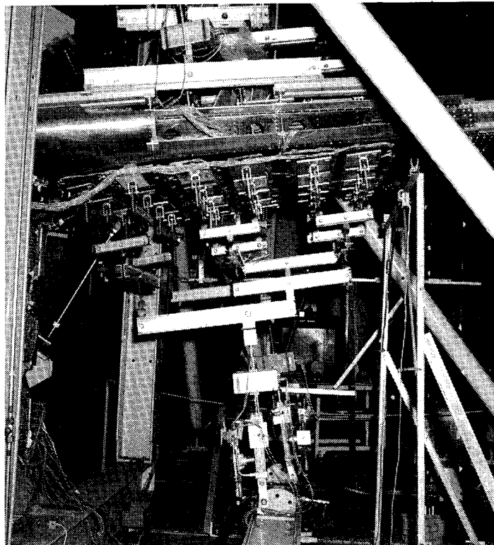
Figure 23. Stub Box Test Setup
