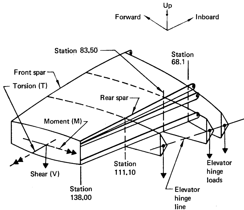
1778.0-mm (70-in) long inspar box test section
