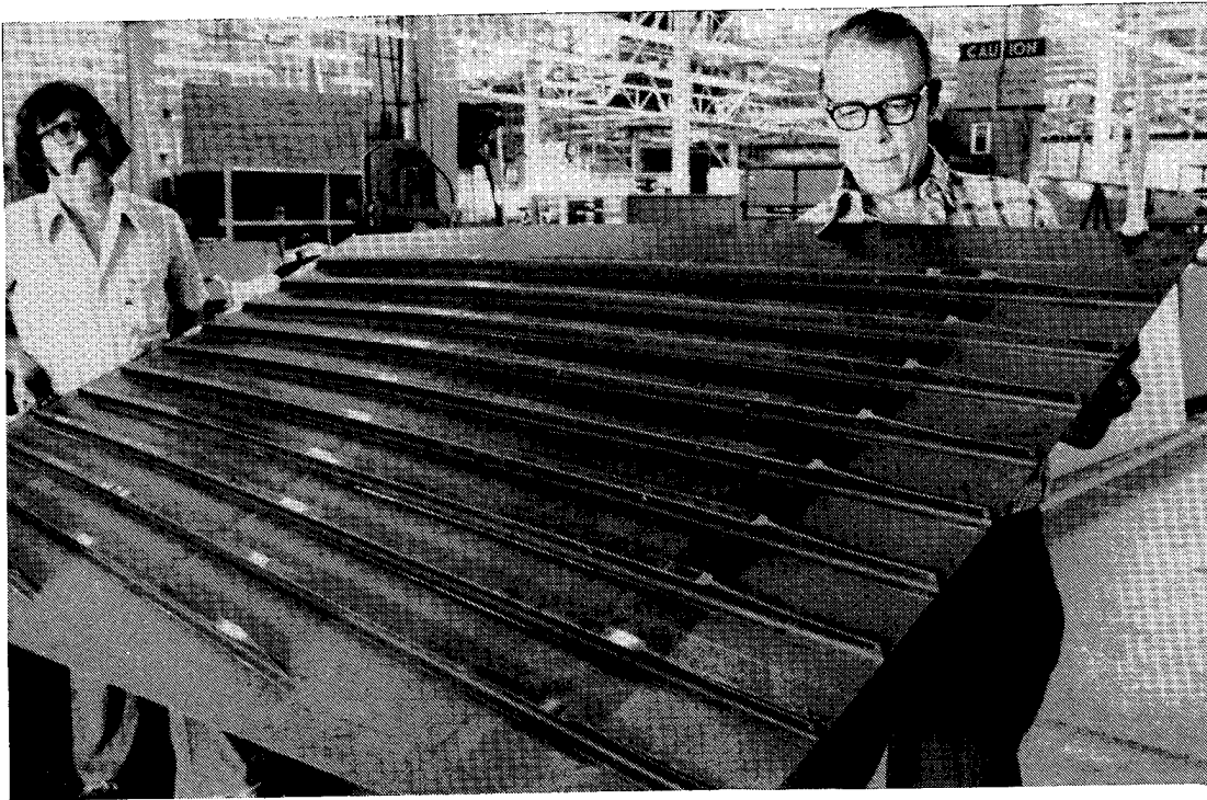
Figure 44. Stub Box I-Stiffened Skin Panel—Trimmed Part
