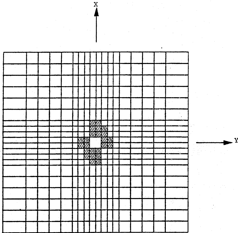
Figure 34. Elements with Ply Damage, T = 3.75 \times 10^{-5} sec., Stress Solution, Modified Model
