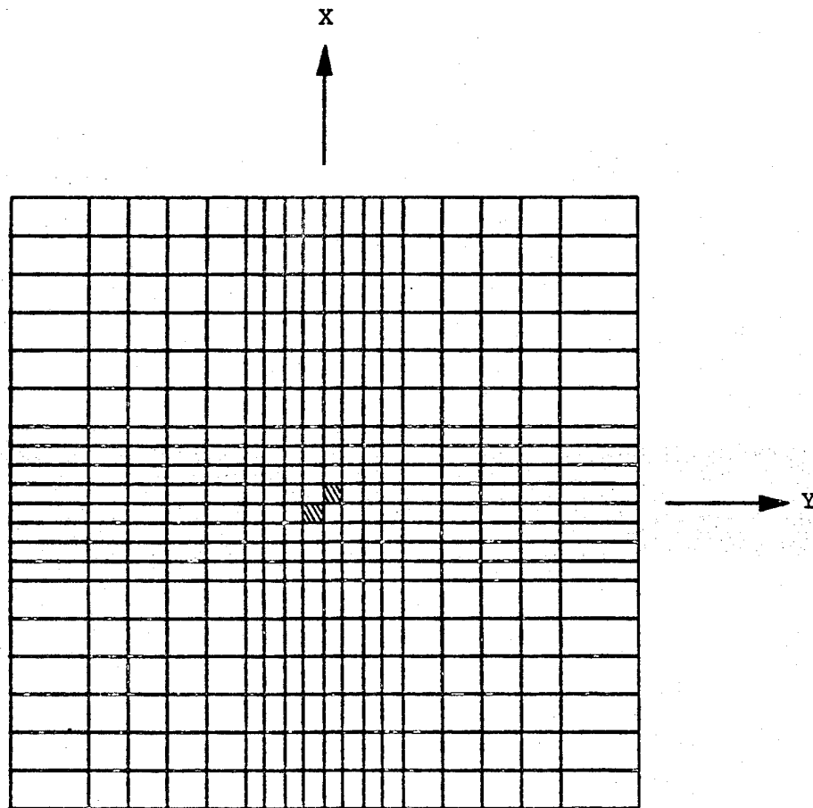
Figure 17. Elements with Top Ply Damage, T = 2.5 \times 10^{-5} sec., Stress Solution, Mass Lumped at One Node
