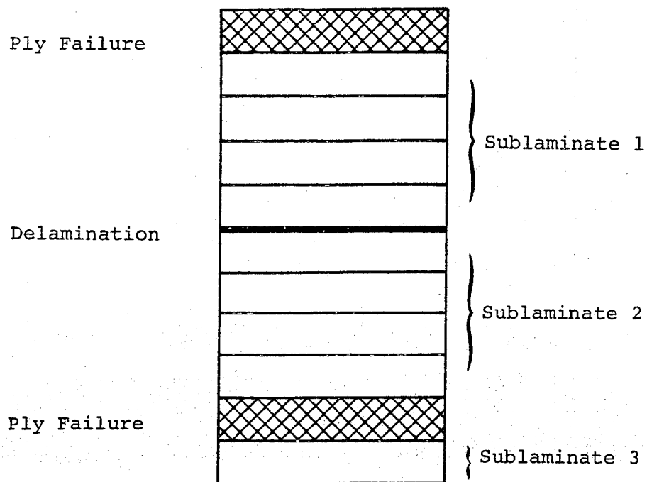
Figure B-4. Typical Failed Laminate
