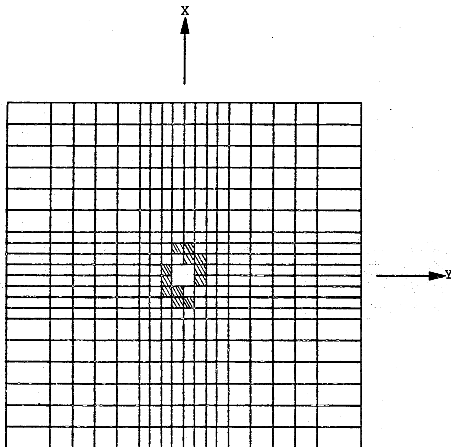
Figure 31. Elements with Ply Damage, T = 1.25 \times 10^{-5} sec., Stress Solution, Modified Model
