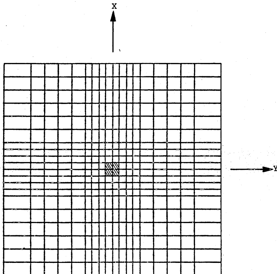
Figure 15. Elements with Interlaminar Damage, T = 1.25 \times 10^{-5} sec., Stress Solution, Mass Lumped at One Node
