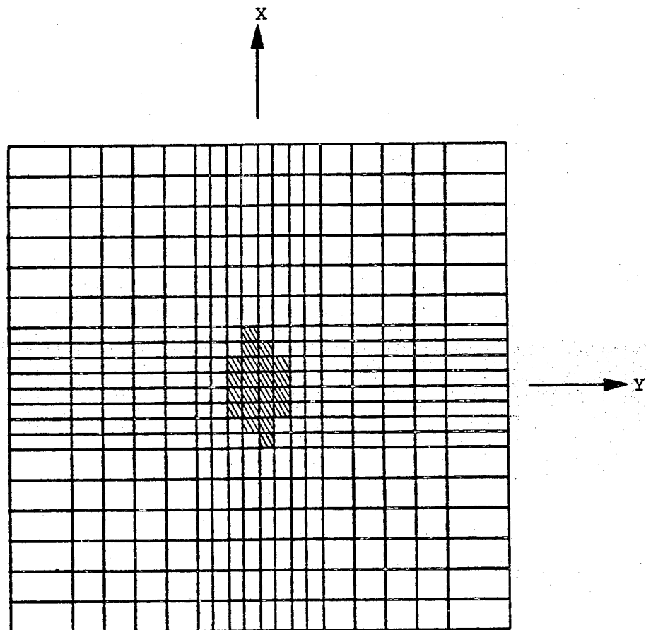
Figure 25. Elements with Ply Damage, T = 2.5 \times 10^{-5} sec., Stress Solution, Mass Distributed at 5 Nodes
