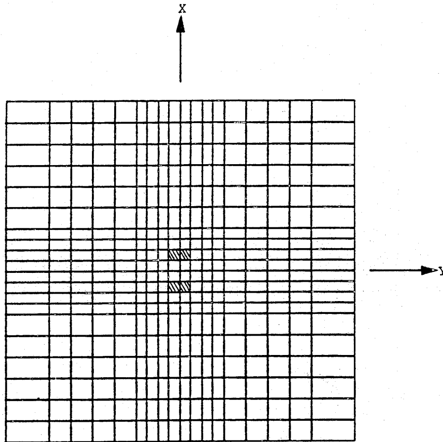
Figure 30. Elements with One Remaining Intact Ply Interface, T = 3.75 \times 10^{-5} sec., Stress Solution, Mass Distributed at 5 Nodes
