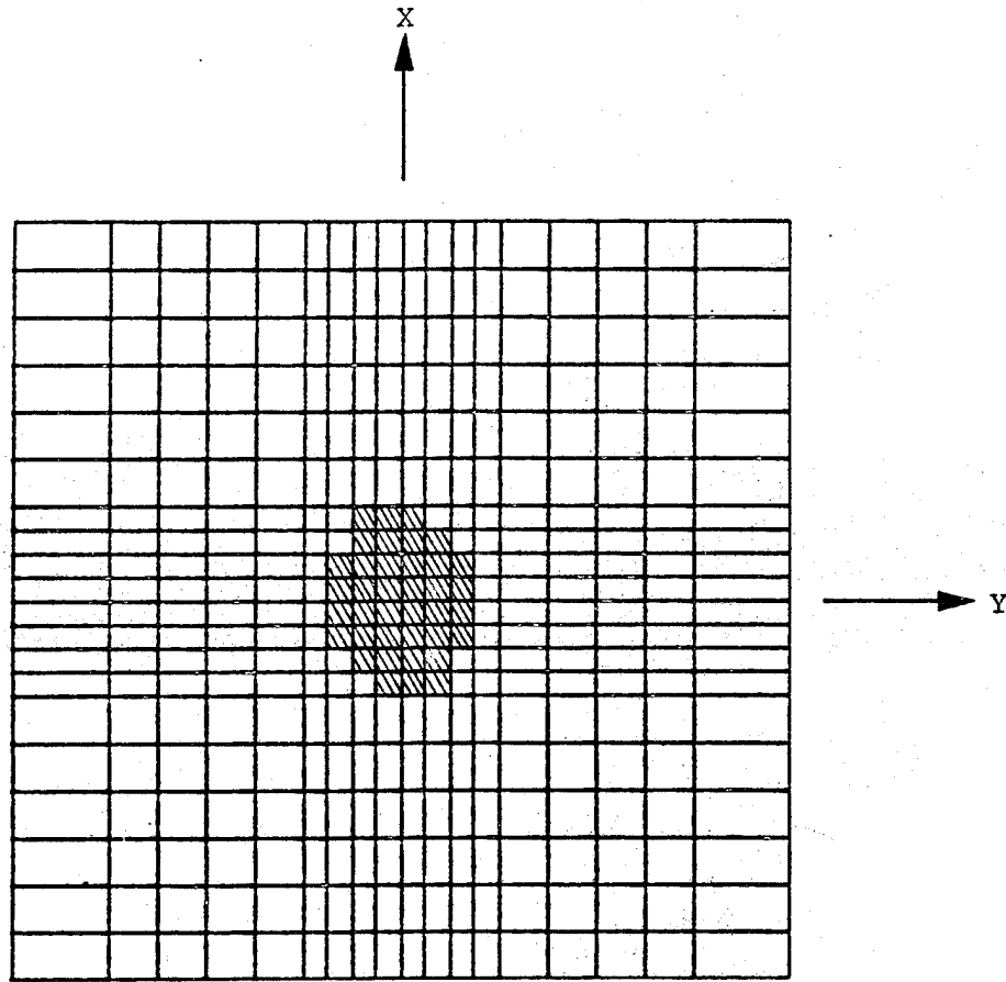
Figure 18. Elements with Ply Damage, T = 3.75 \times 10^{-5} sec., Stress Solution, Mass Lumped at One Node
