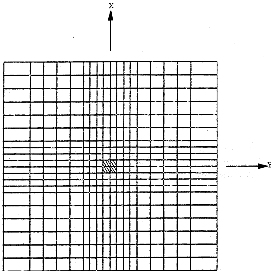
Figure 28. Elements with Fiber Damage, T = 5.0 \times 10^{-5} sec., Stress Solution, Mass Distributed at 5 Nodes
