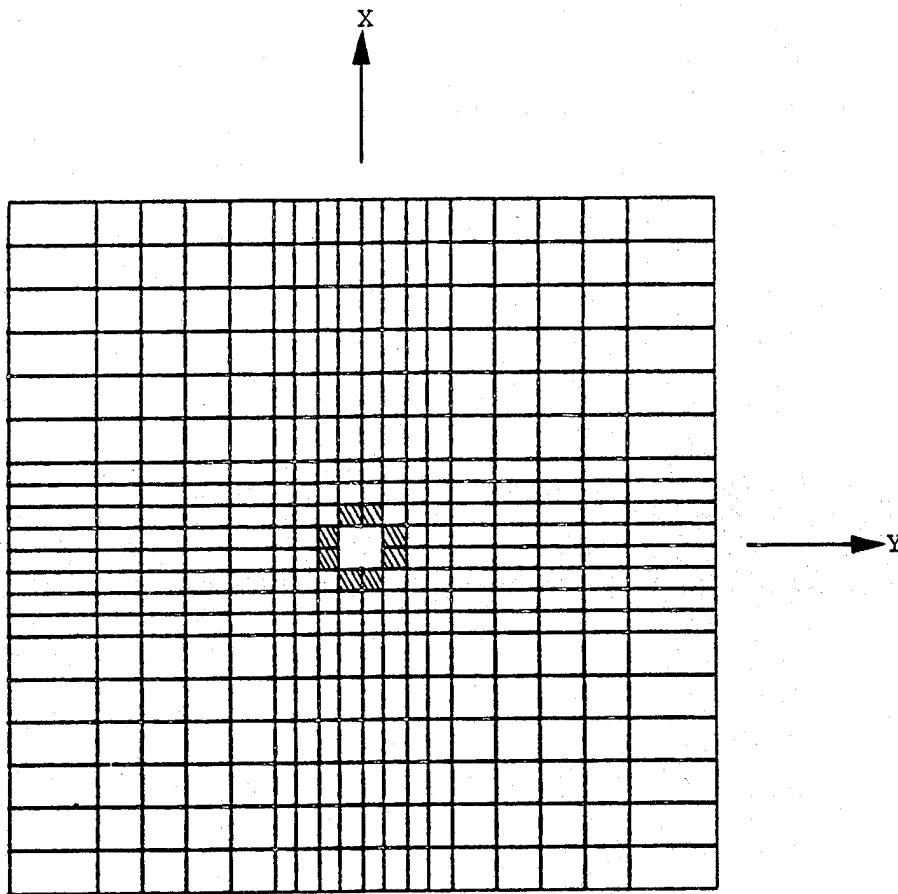
Figure 32. Elements with Interlaminar Damage, T = 1.25 \times 10^{-5} sec., Stress Solution, Modified Model
