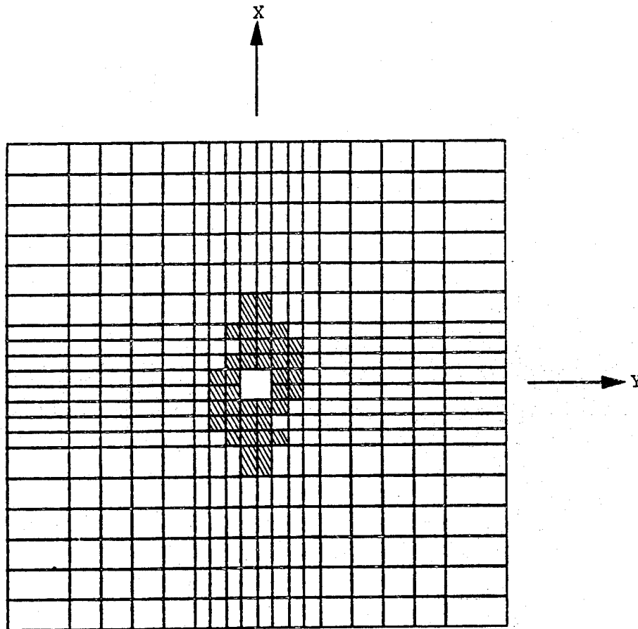
Figure 36. Elements with Ply Damage, T = 6.25 \times 10^{-5} sec., Stress Solution, Modified Model
