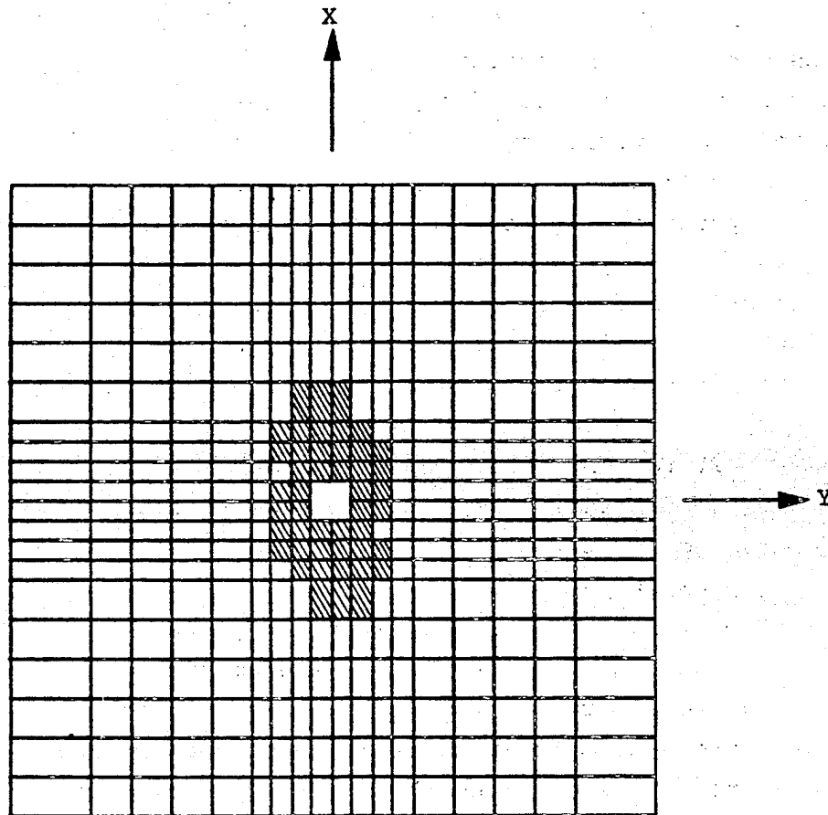
Figure 37. Elements with Ply Damage, T = 7.5 \times 10^{-5} sec., Stress Solution, Modified Model
