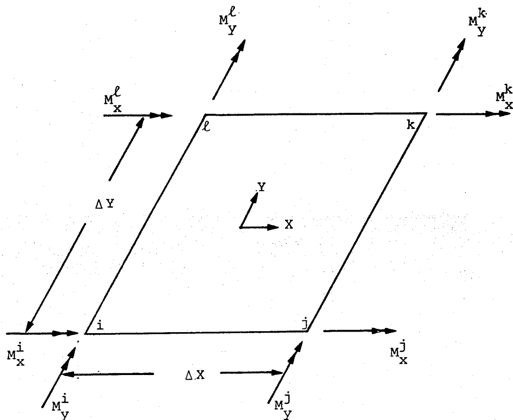
Figure A-2. Elemental Nodal Moments
