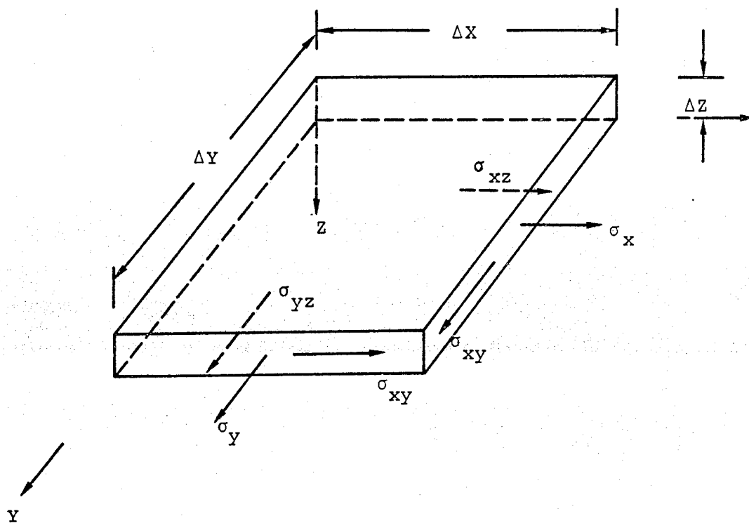
Figure B-2. Interlaminar Shear Stresses
