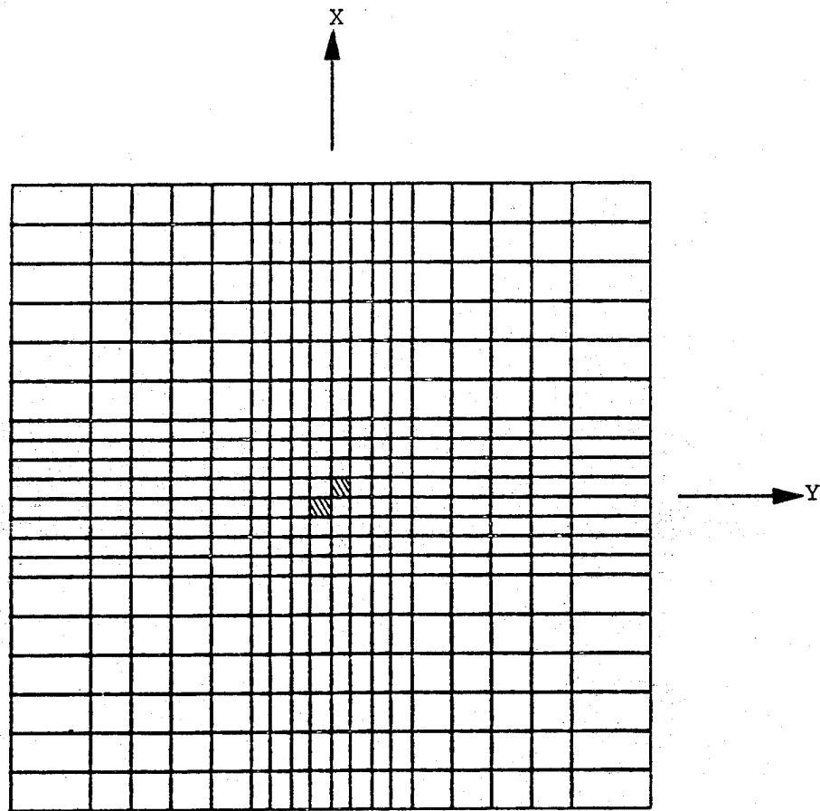
Figure 22. Elements with Fiber Failure, T = 7.5 \times 10^{-5} sec., Stress Solution, Mass Lumped at One Node
