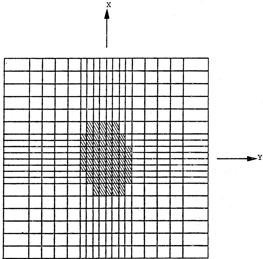
Figure 20. Elements with Ply Damage, T = 7.5 \times 10^{-5} sec., Stress Solution, Mass Lumped at One Node
