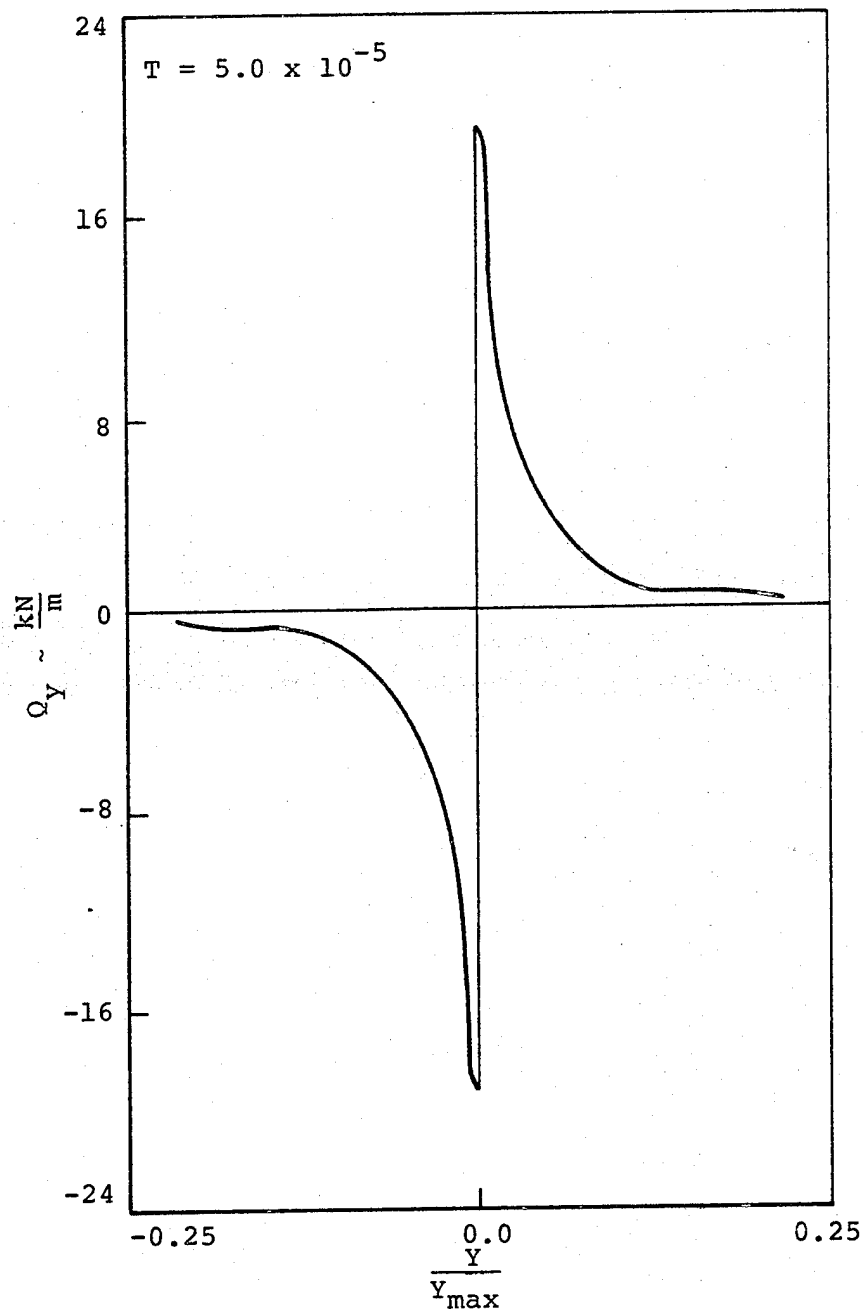
Figure 12. Transverse Shear Resultant, Q_y , Through the Plate Center Along the Shorter Axis, Stress Solution, Mass Lumped at One Node.
