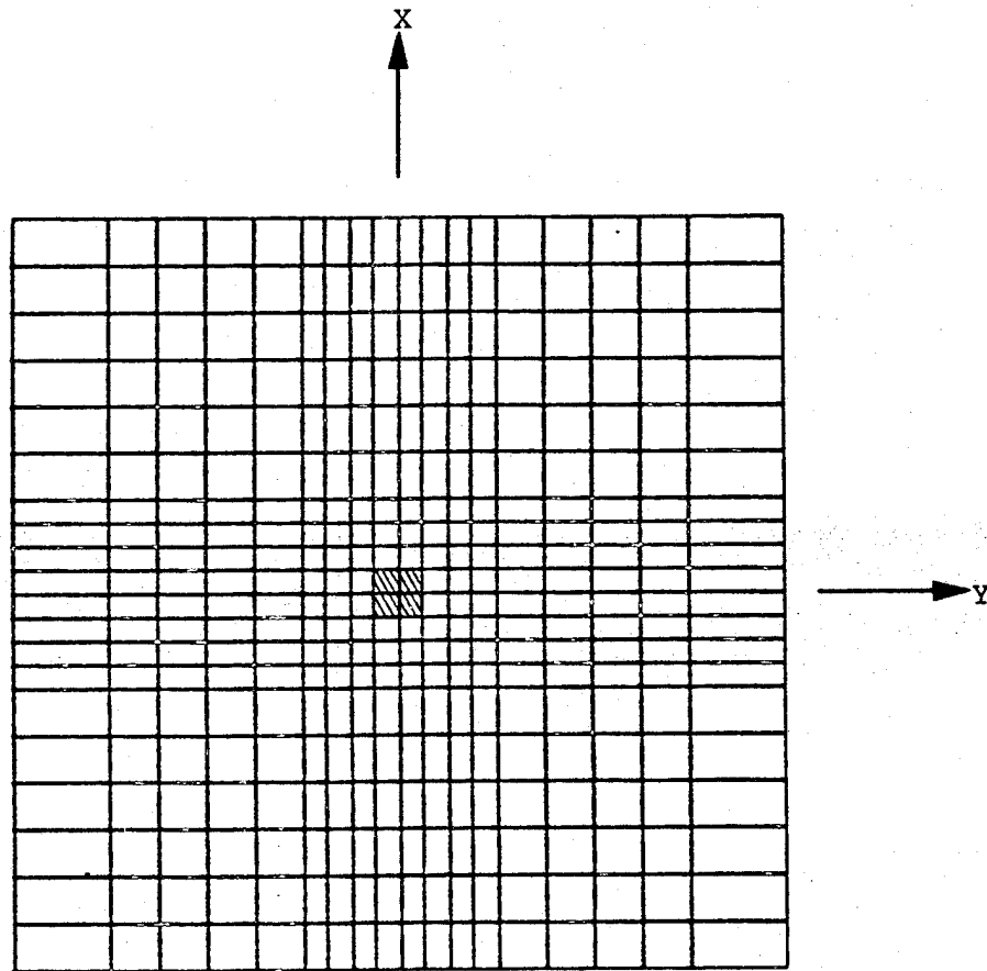
Figure 29. Elements with No Remaining Intact Ply Interfaces, T = 2.5 \times 10^{-5} sec., Stress Solution, Mass Distributed at 5 Nodes
