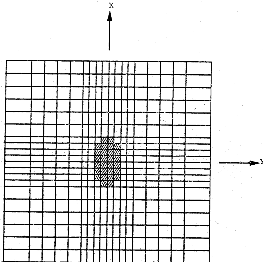
Figure 16. Elements with Ply Damage, T = 2.5 \times 10^{-5} sec., Stress Solution, Mass Lumped at One Node
