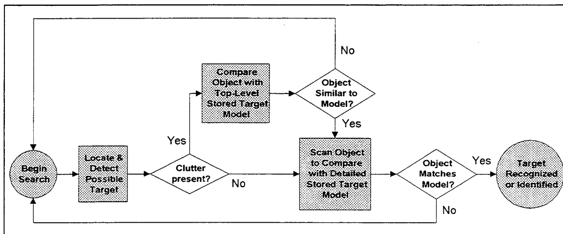
Figure 1. Search and Scan Processes With and Without Clutter Present.
