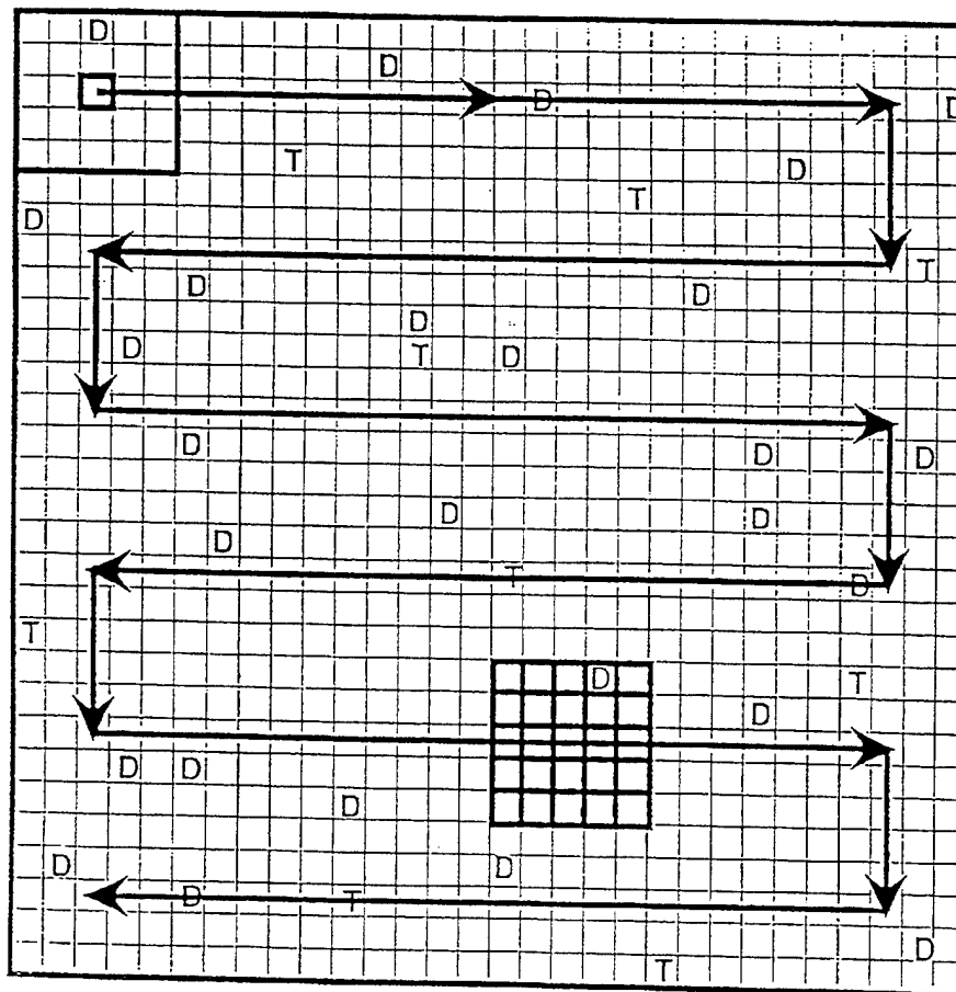
Figure 15. Example of a Search Scene. Each large square (upper left) represents 5 degrees of visual angle, the visual lobe size set for one glimpse of the scene. A small square (center of the large square) represents 1 degree of the visual lobe. A systematic row search pattern is illustrated here. The letter T indicates the location of a target; D indicates a decoy. The center 1-degree square within a 5-degree total glimpse area represents the extent of foveal vision (0.5 degree) plus 0.5 degree of peripheral vision; the distance of the other small squares from this central square represents the eccentricity (distance into the periphery) of a target/decoy. [See Footnote 15]
