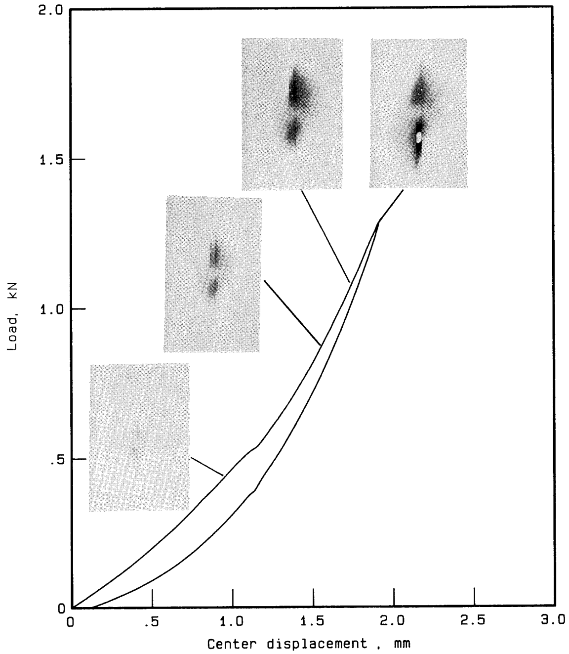
Figure 10.- X-ray delamination analysis for static test conditions.
