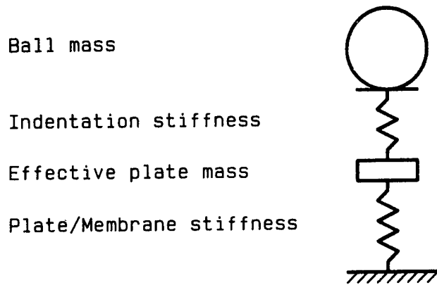
Figure 6.- Two-degree-of-freedom model for impact on a thin plate.
