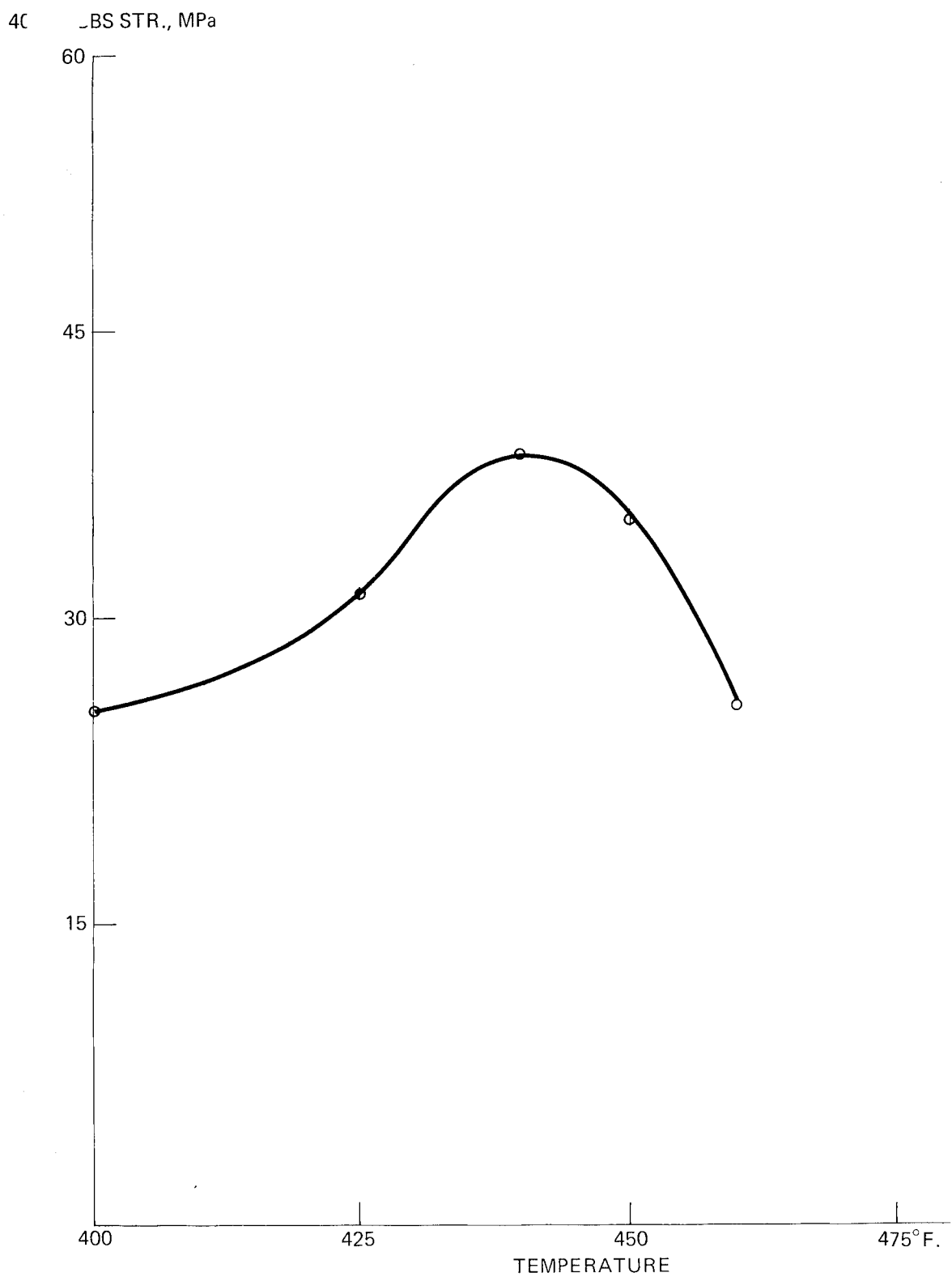
FIGURE 25 — NCNS-12M/181E GLASS FABRIC LAMINATE I-19N-139 POST CURING STUDIES
