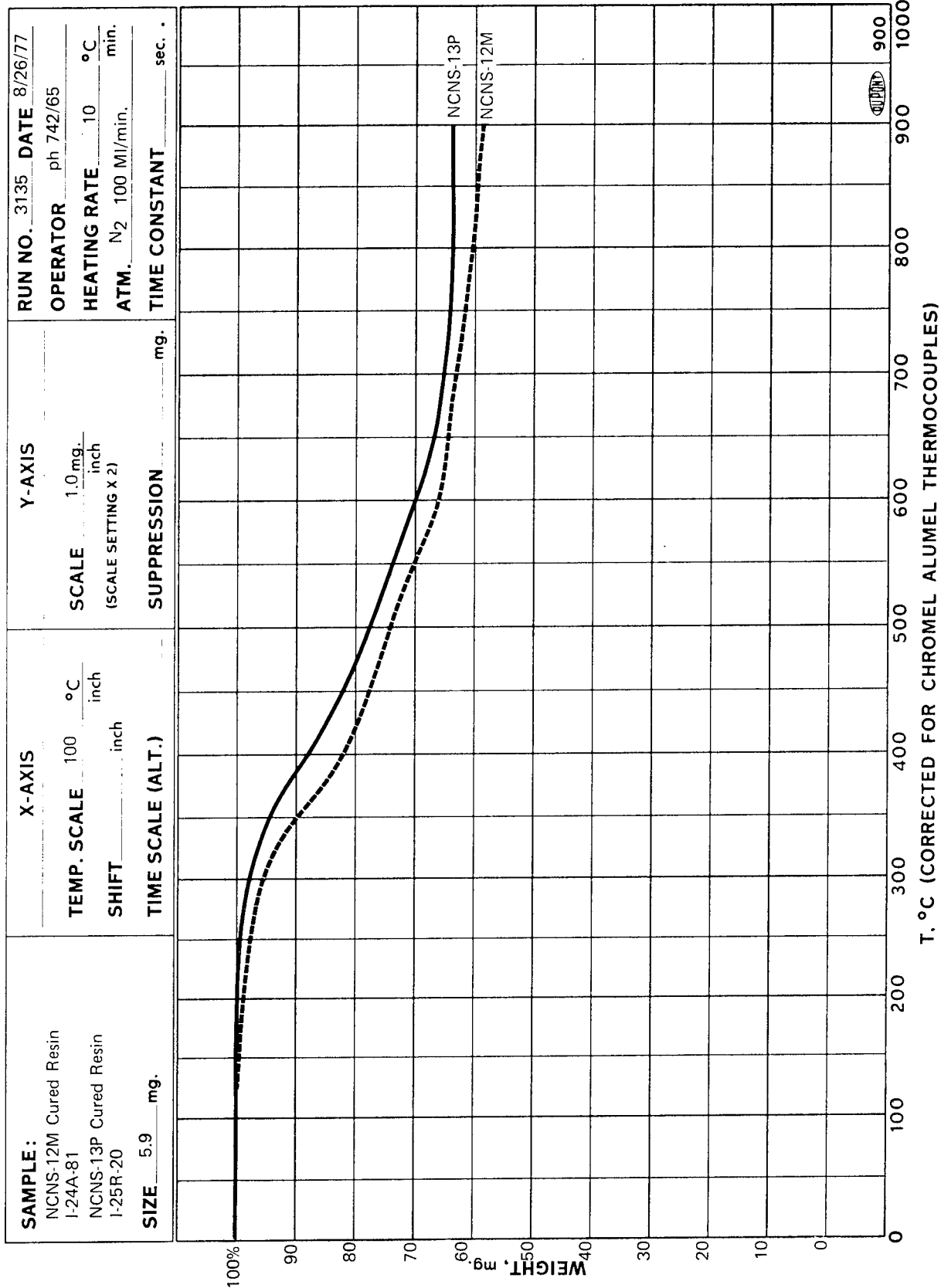
FIGURE 24 — THERMOGRAVIMETRIC ANALYSIS OF NCNS CURED RESINS
