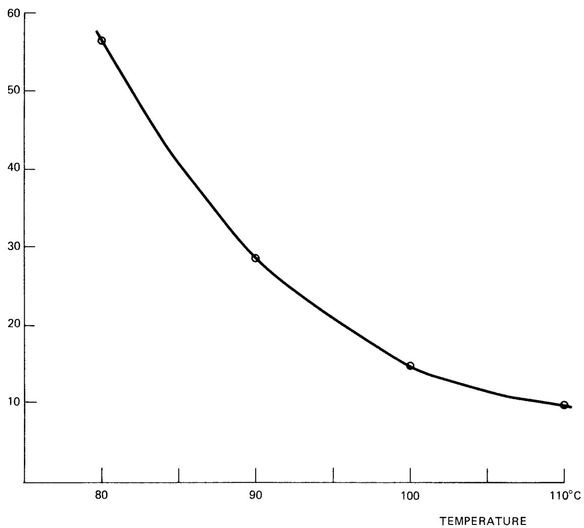
FIGURE 47 — GEL TIME VS. TEMPERATURE FOR 90/10 NCNS-13P/CY 179 RESIN BATCH NO. I-261-72
