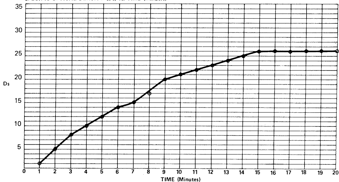
SPECIFIC OPTICAL DENSITY (Ds) vs. TIME (Minutes)
