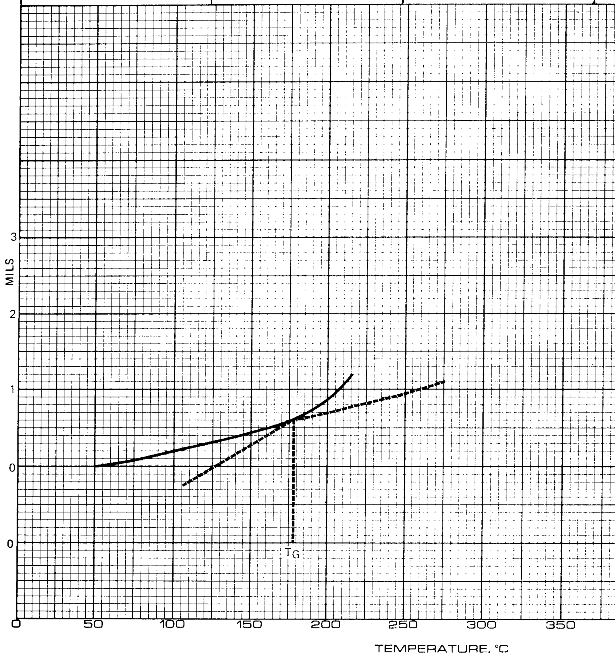
FIGURE 34 – Z-AXIS THERMAL EXPANSION OF NCNS-13P/HT-S GRAPHITE FIBER LAMINATE I-24A-105 AFTER 30 DAY, 95% R.H., 120°F, HUMIDITY EXPOSURE
