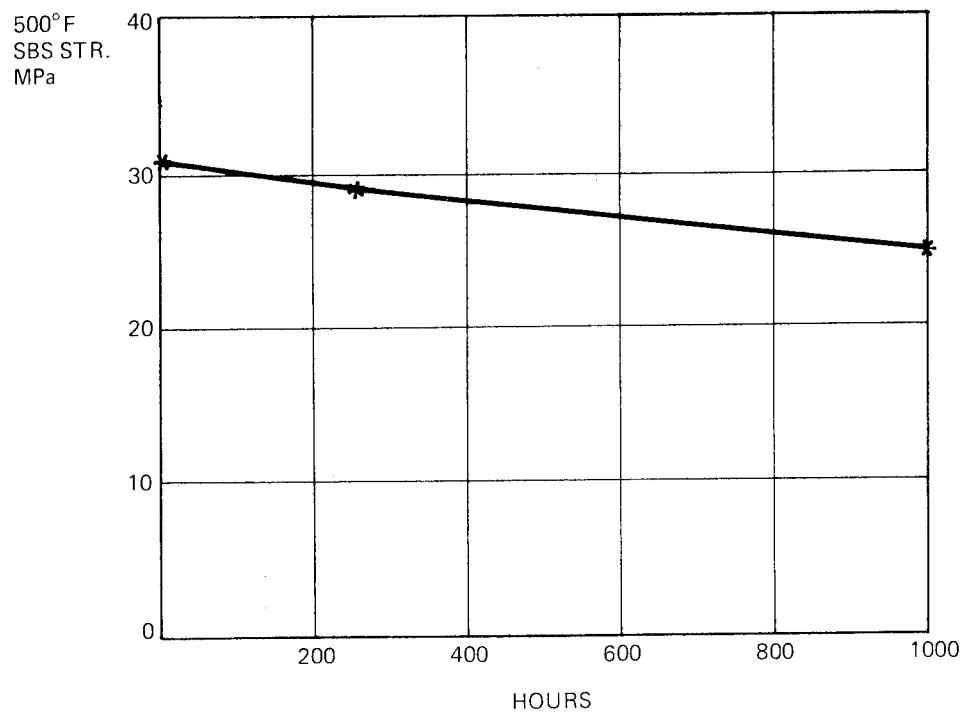
FIGURE 4 – 500°F. OXIDATIVE AGING OF LAMINATE I-22F-106
