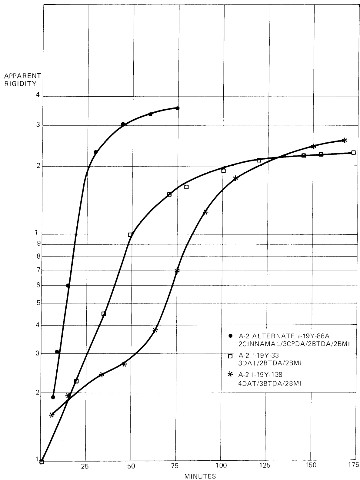
FIGURE 18 — APPARENT RIGIDITY VS. TIME FOR 400°F. AUTOCLAVE POLYIMIDES—CURE TEMPERATURE 400°F.
