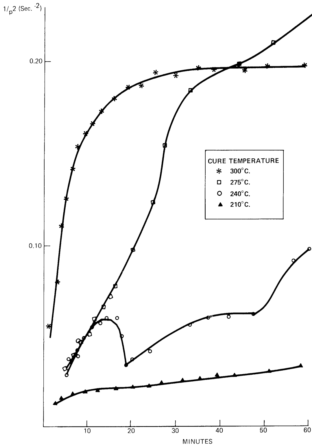
FIGURE 8 — TBA CURING STUDY ON 4/2/1 IMIDE PREPOLYMER — — APPARENT RIGIDITY VS TIME
