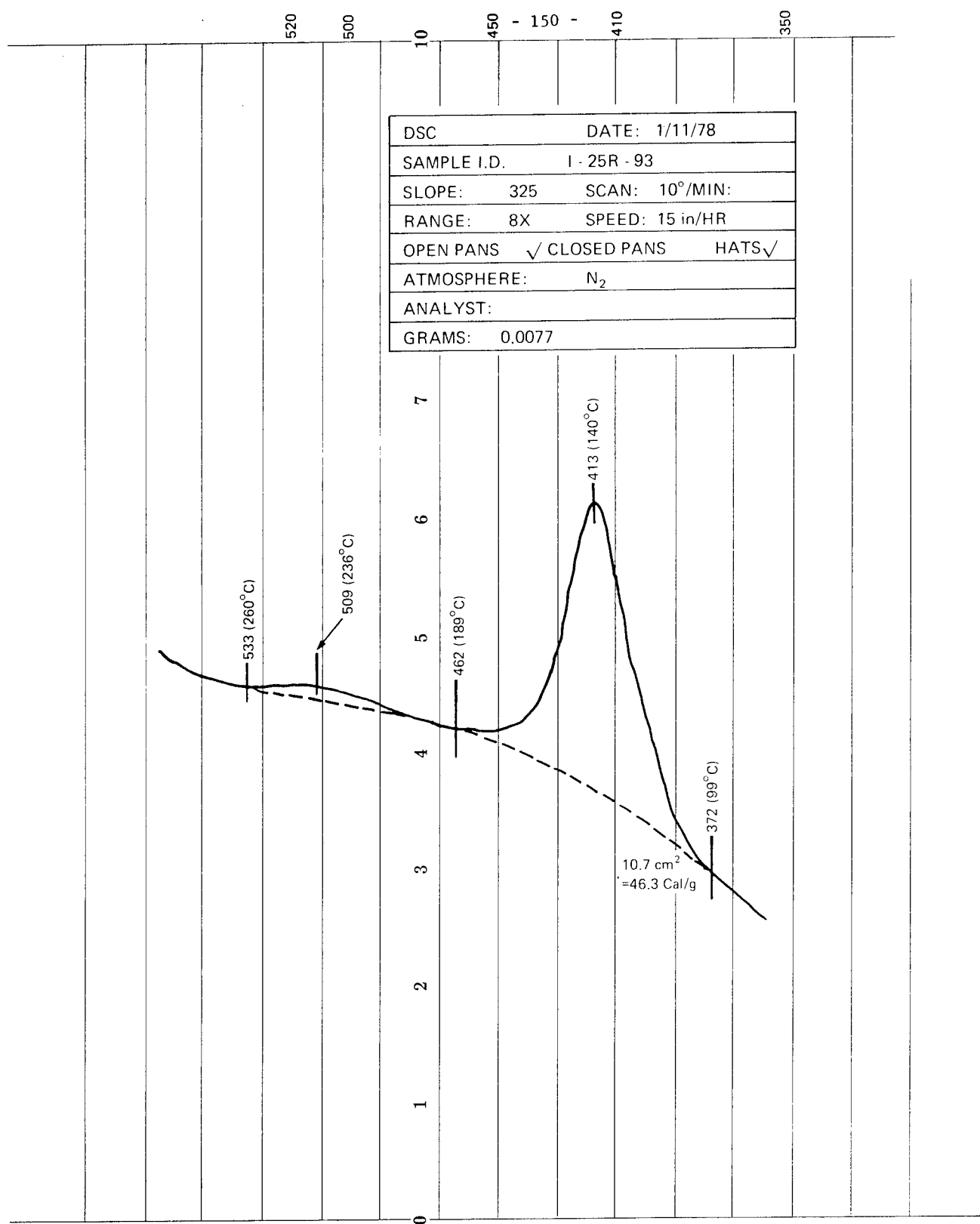
FIGURE 48 – DIFFERENTIAL SCANNING CALORIMETRY RUN ON 90% NCNS-13P/10% CY 179 EPOXY ALLOY
