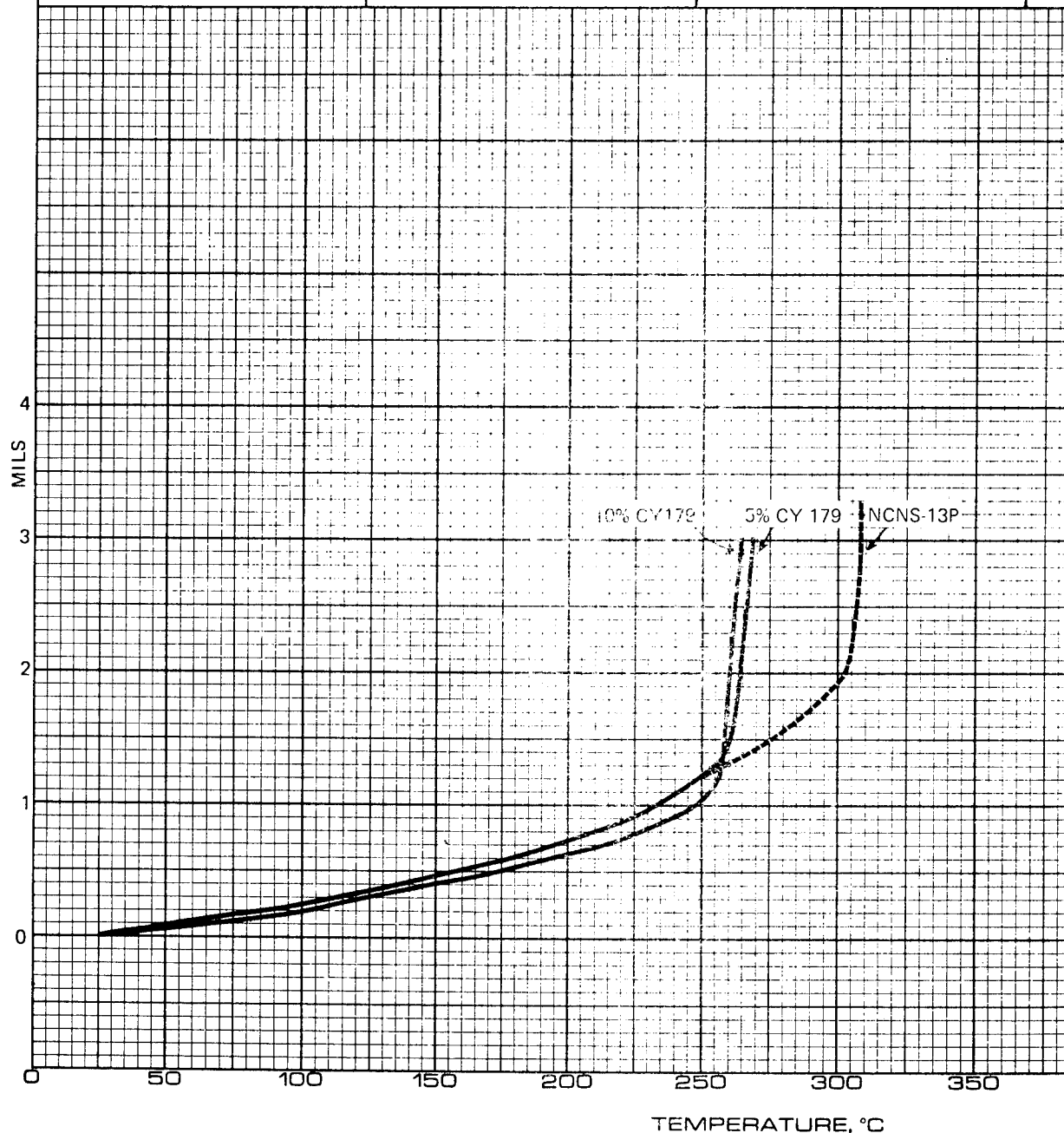
FIGURE 49 – Z-AXIS THERMAL EXPANSIONS OF AS UNIDIRECTIONAL GRAPHITE FIBER LAMINATES PREPARED FROM NCNS-13P RESIN WITH VARYING AMOUNTS OF ARLDITE CY179 EPOXY RESIN
