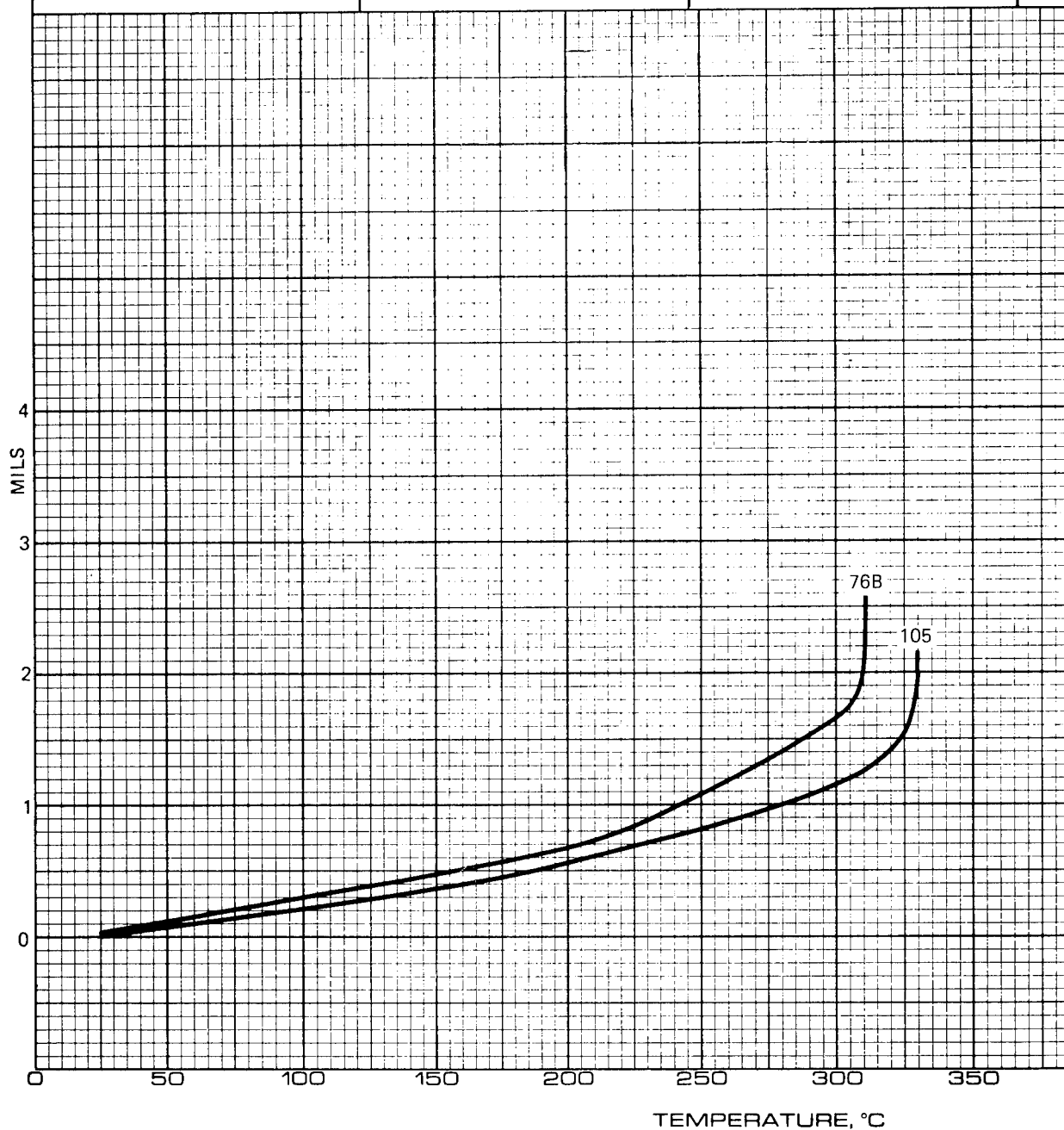
FIGURE 33 — EFFECT OF POST CURE CYCLE ON THERMAL EXPANSION IN Z-AXIS OF NCNS-13P/HT-S UNIDIRECTIONAL GRAPHITE FIBER LAMINATES
