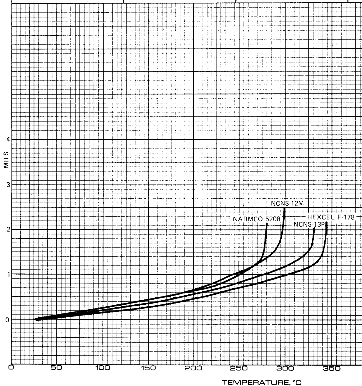
FIGURE 35 – COMPARISON OF THERMAL EXPANSION IN Z-AXIS OF COMPETITIVE RESINS IN UNIDIRECTIONAL GRAPHITE FIBER LAMINATES
