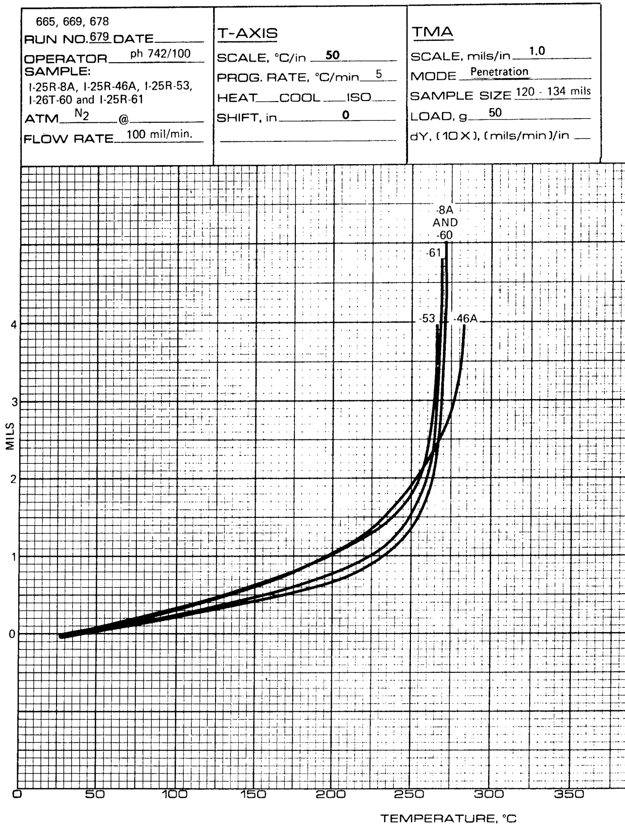
FIGURE 46 – Z-AXIS THERMAL EXPANSION OF 181E GLASS CLOTH LAMINATES PREPARED FROM NCNS-13PE RESINS I-25R-8A, I-25R-46A, I-25R-53, I-25R-60 AND I-25R-61
