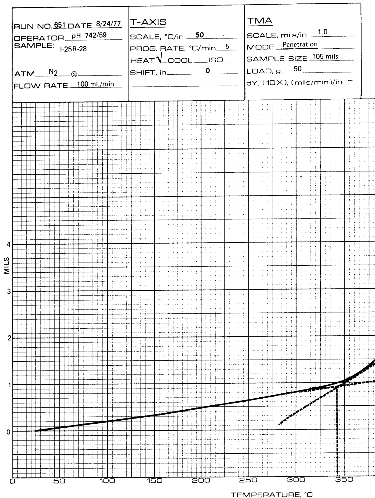
FIGURE 10 — THERMAL EXPANSION IN Z-AXIS OF GLASS CLOTH LAMINATE I-25R-28
