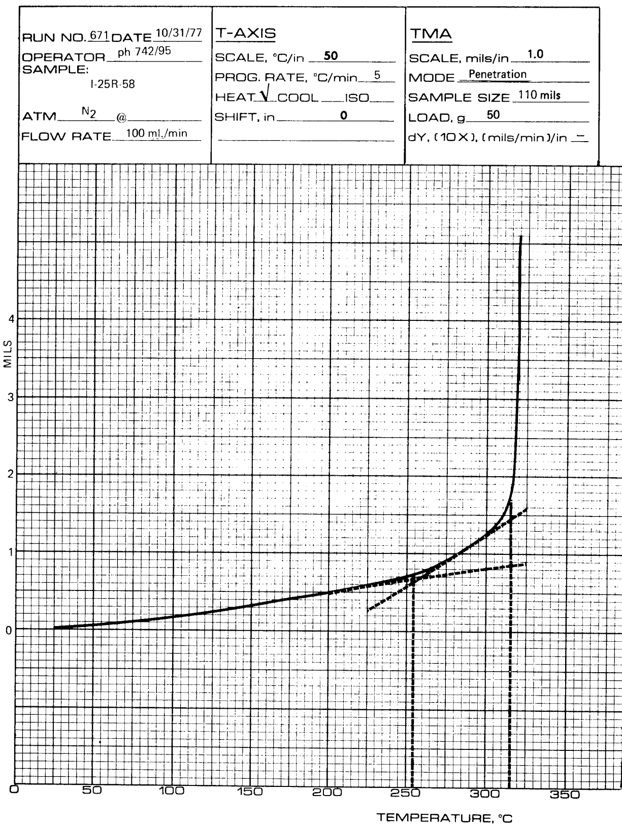
FIGURE 31 — Z-AXIS THERMAL EXPANSION OF NCNS-13P/181E GLASS CLOTH LAMINATE I-25R-58
