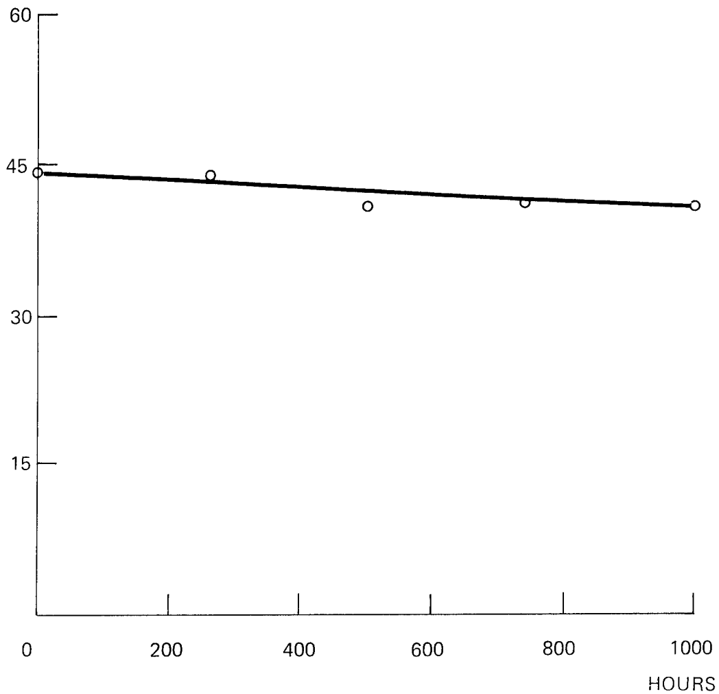
FIGURE 26 – 400°F. OXIDATIVE AGING OF NCNS-13M/181E GLASS LAMINATE I-22F-16
