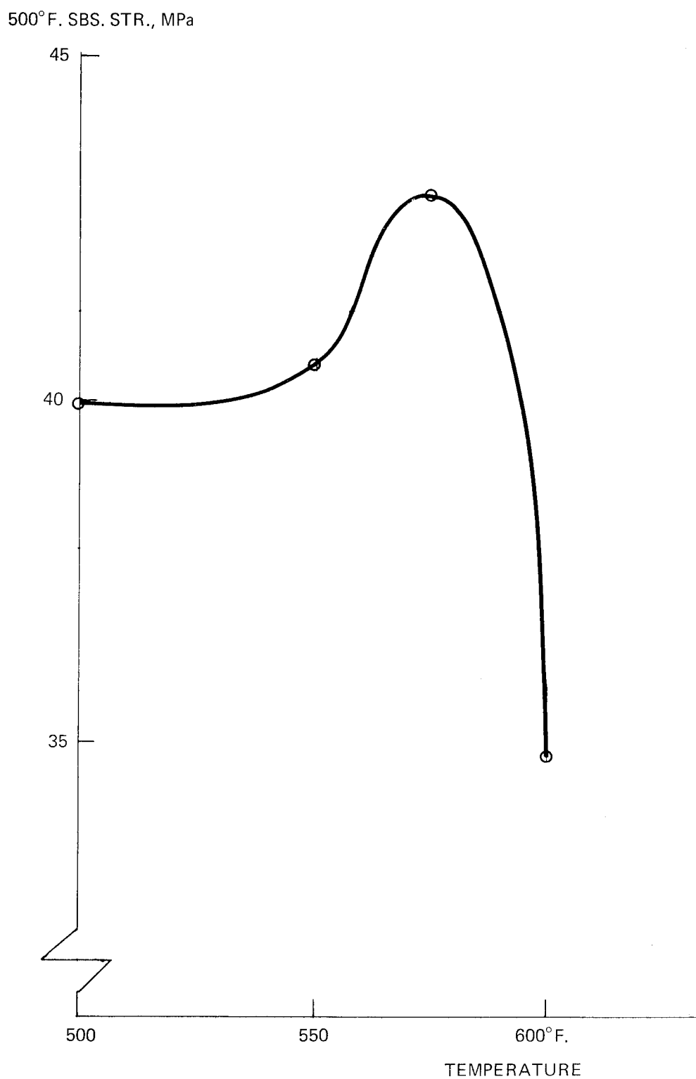
FIGURE 19 – A-2 ALTERNATE-181E GLASS FABRIC LAMINATE I-19N-124 POST CURING STUDIES
