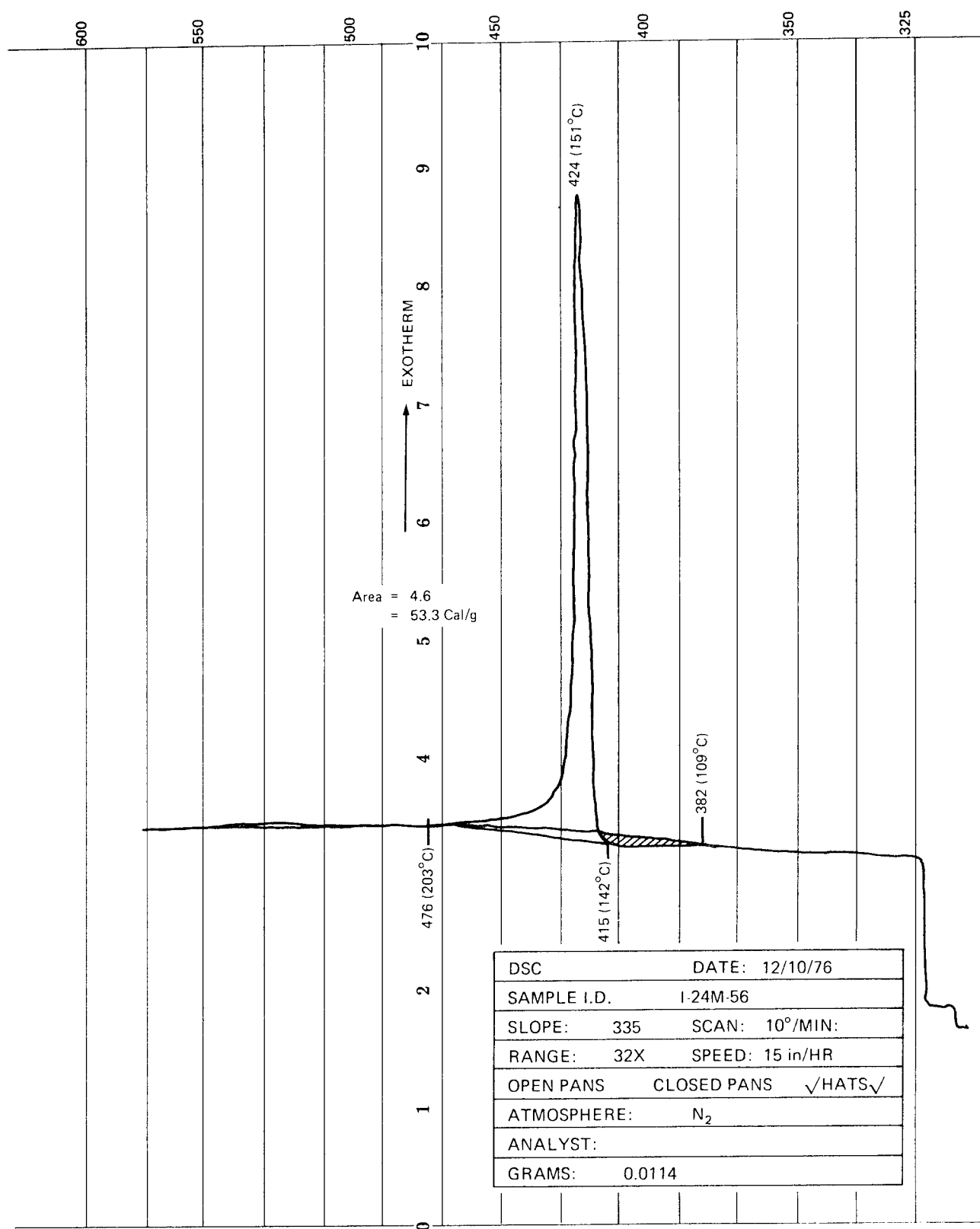
FIGURE 30 – DIFFERENTIAL SCANNING CALORIMETRY OF NCNS-14P RESIN RUN No. I-24M-56
