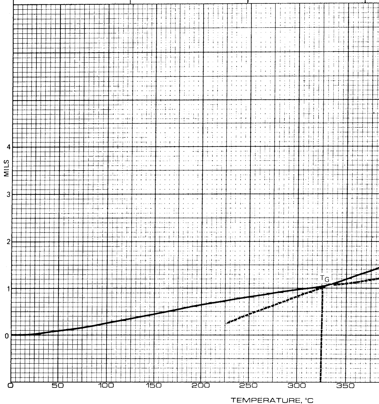
FIGURE 16 – Z-AXIS THERMAL EXPANSION OF 1-25R-151 POLYIMIDE/CELION 6000 UNIDIRECTIONAL GRAPHITE FIBER LAMINATE
