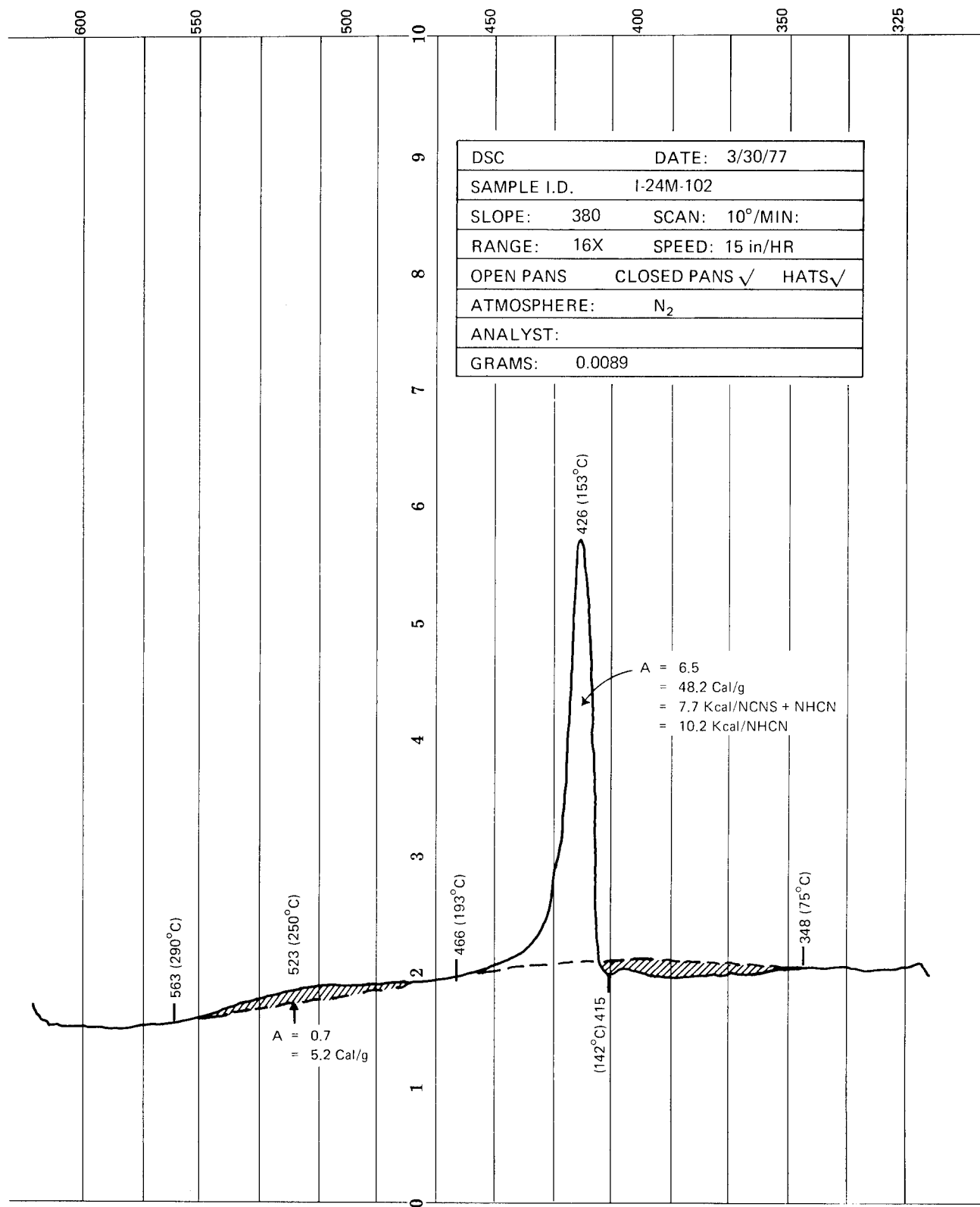
FIGURE 29 — DIFFERENTIAL SCANNING CALORIMETRY OF NCNS - 13P RUN No. I-24A-102
