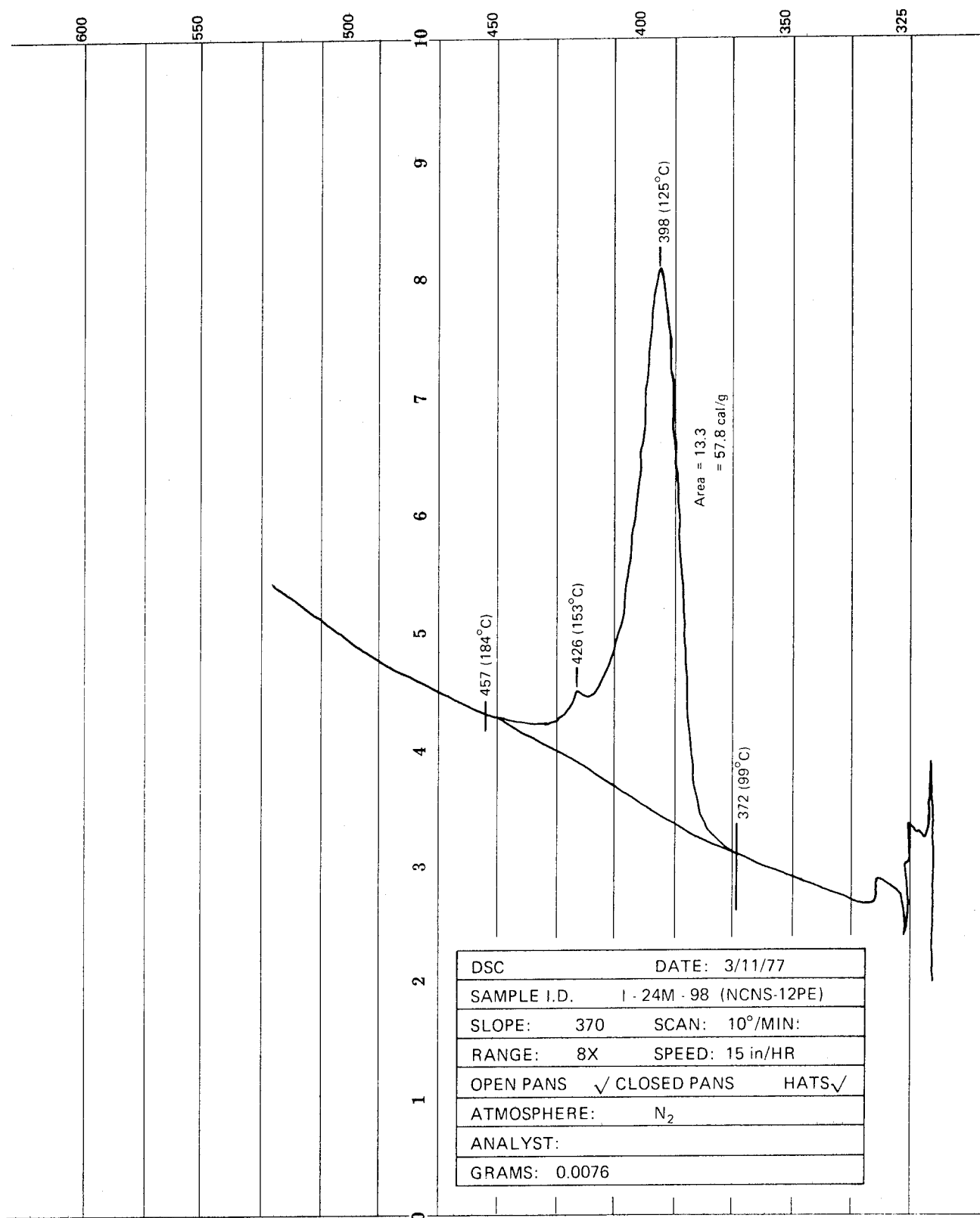
FIGURE 40 — DIFFERENTIAL SCANNING CALORIMETRY OF NCNS - 12PE RESIN RUN No. I-24M-98
