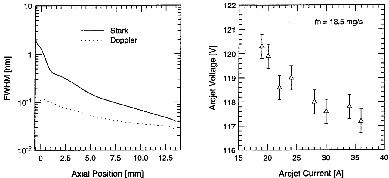
Figure 2. A comparison between the Stark and Doppler broadening of H_\alpha along the axis of the 5 kW arcjet.
