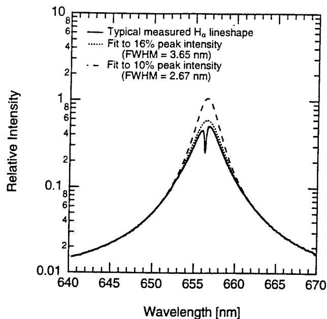
Figure 7. Typical measured H_\alpha lineshape with best fit Lorentzian functions to the linewings. The best fits differ in how much of the linewings are used in the fitting procedure as indicated by the percentage of the peak intensity used in the fitting. The difference in FWHM of nearly forty percent corresponds to a difference in electron number density of nearly seventy percent.
