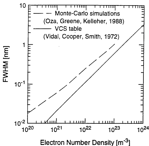
Figure 6. The Stark broadening of H_\alpha showing the discrepancy between the static ion calculations by Vidal, Cooper and Smith (solid) and the more recent dynamic ion Monte-Carlo simulations by Oza, Greene and Kelleher (dashes).
