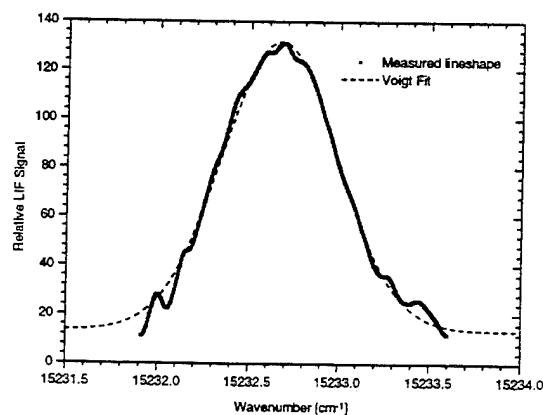
Figure 6. Typical LIF scan of H_{\alpha} at the arcjet exit plane centerline and best fit "forced" Voigt function.
