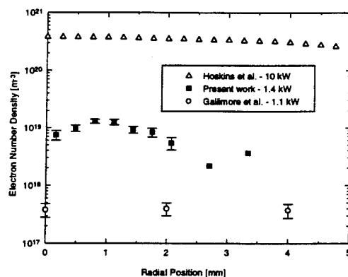
Figure 12. A comparison of measured electron number densities in the arcjet plume. The error bars are omitted for the data points at 2.7 and 3.3 mm because the errors are greater than 100 percent.
