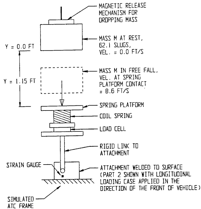
Figure 18. Test setup.
