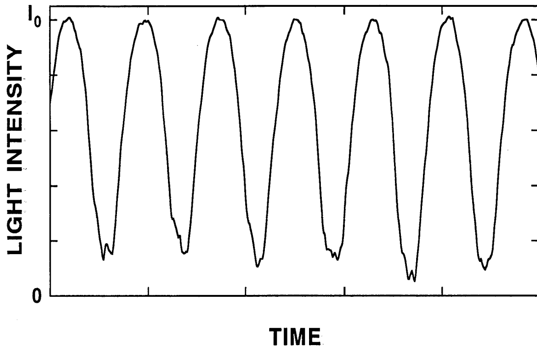
Figure 3. Trace of signal obtained from a modulated HeNe laser beam which has been bounced off a substrate and through the tuning fork chopper.
