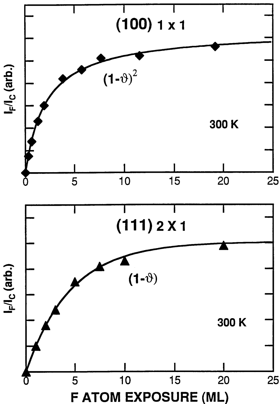
Figure 2. Uptake of fluorine atoms on the (100) and (111) surfaces as a function of F atom exposure at 300 K. (1 ML is the equivalent of one fluorine atom per surface carbon.) The integrated fluorine signal from the XPS F 1s spectra have been normalized to the integrated carbon 1s spectra. The fits to the data (represented by solid curves) assume a model in which the uptake rate of fluorine atoms is proportional to some order to the number of unoccupied sites, 1-\theta , where \theta is the fractional fluorine atom coverage.
