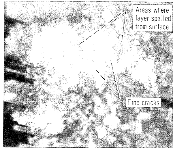
(b) Sliding interval, 15 kilocycles.
