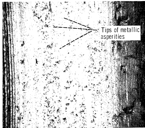
(b) Sliding interval, 3500 kilocycles.
