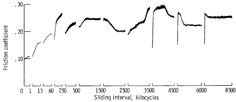
Figure 2. - Friction trace for 440C HT stainless-steel rider (with 0.95-mm-diam flat) sliding on polyimide-bonded graphite fluoride film. Load, 1 kilogram; speed, 2.6 meters per second; test temperature, 25° C; test atmosphere, moist air (10 000 ppm H 2 O).
