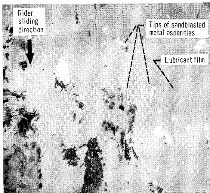
(a) Sliding interval, 3500 kilocycles.
