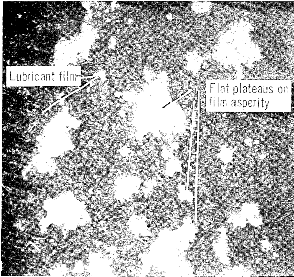
(a) Sliding interval, 1 kilocycle.
