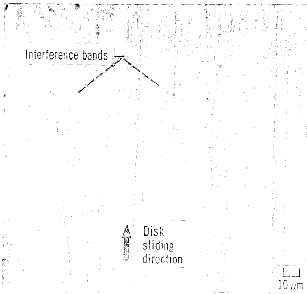
(a) Middle of scar (after 1 kilocycle).
