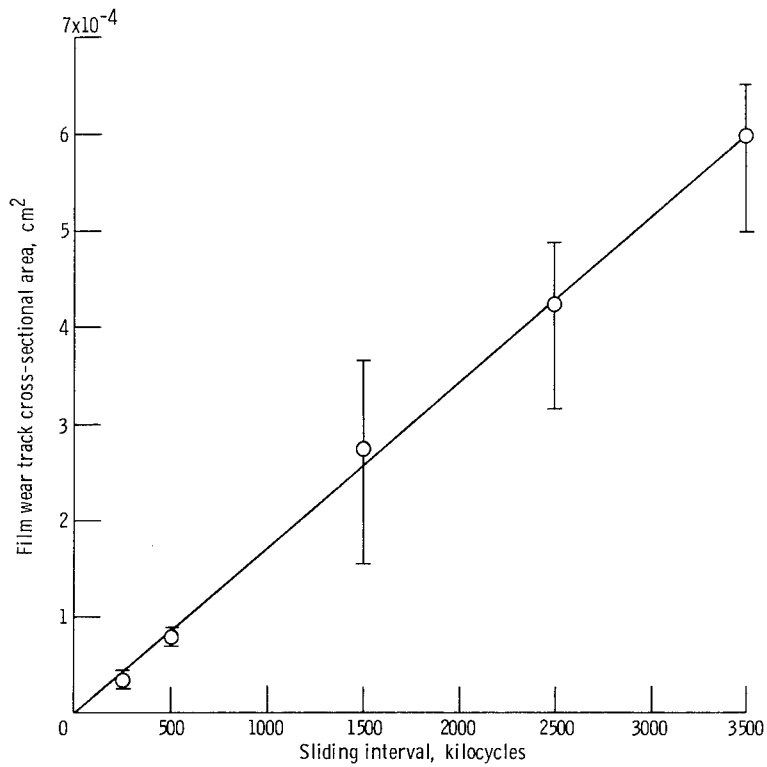
Figure 4. - Wear of polyimide-bonded graphite fluoride film as function of sliding interval. Rider and substrate material, 440C HT stainless steel; load, 1 kg; projected contact stress, 14 MPa (2000 psi); sliding speed, 2.6 m/sec; temperature, 25° C; atmosphere, moist air (10 000 ppm H 2 O).
