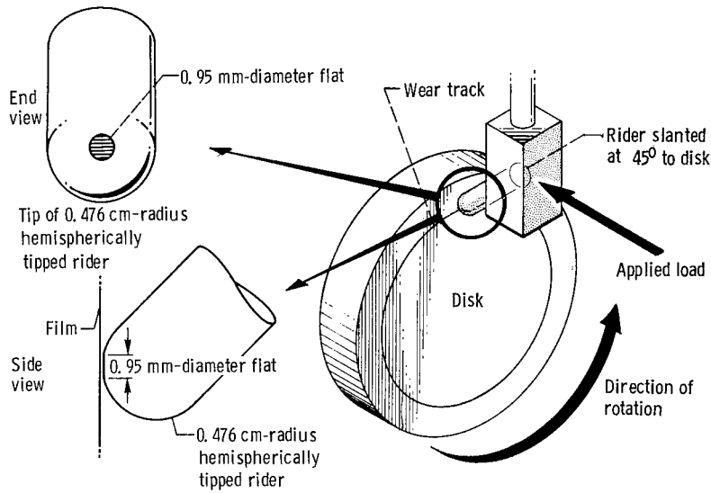
Figure 1. - Schematic arrangement of friction specimens.
