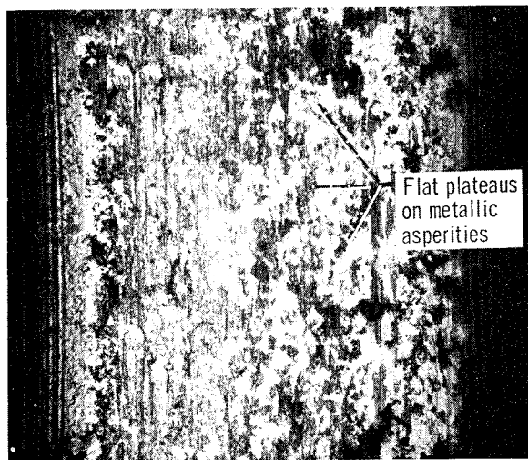
(c) Sliding interval, 6000 kilocycles.
