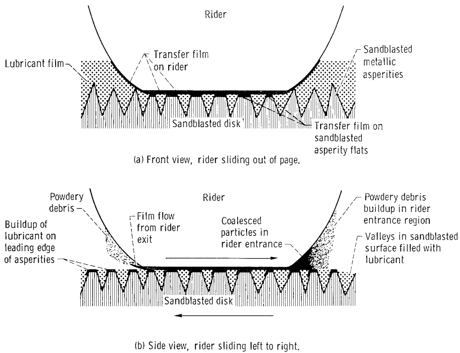
Figure 11. - Idealized schematic drawing of sliding surfaces, illustrating lubricating mechanism in the second stage of lubrication.
