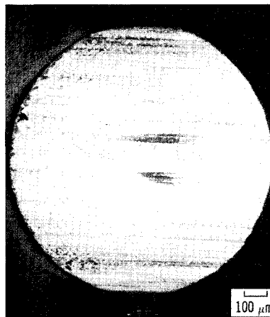
(f) Flat after 8500 kilocycles of sliding.
