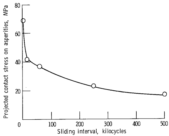
Figure 6. - Projected contact stress on asperities of polyimide-bonded graphite fluoride films as function of sliding interval. Rider and disk substrate material, 440C HT stainless steel; load, 1 kg on 0.95-mm-diameter flat on rider; sliding speed, 2.6 m/sec; temperature, 25° C; atmosphere, moist air (10 000 ppm H 2 O).
