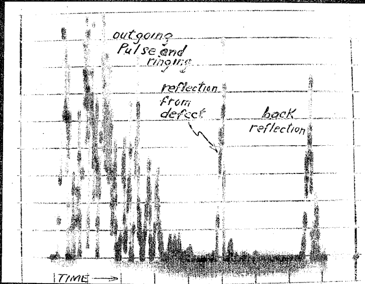
Fig. 2A- Pulse-echo transmission showing reflection from 1 in. dia. hole 8 in. from transducer. Extensive transducer ringing due to high input energy.
