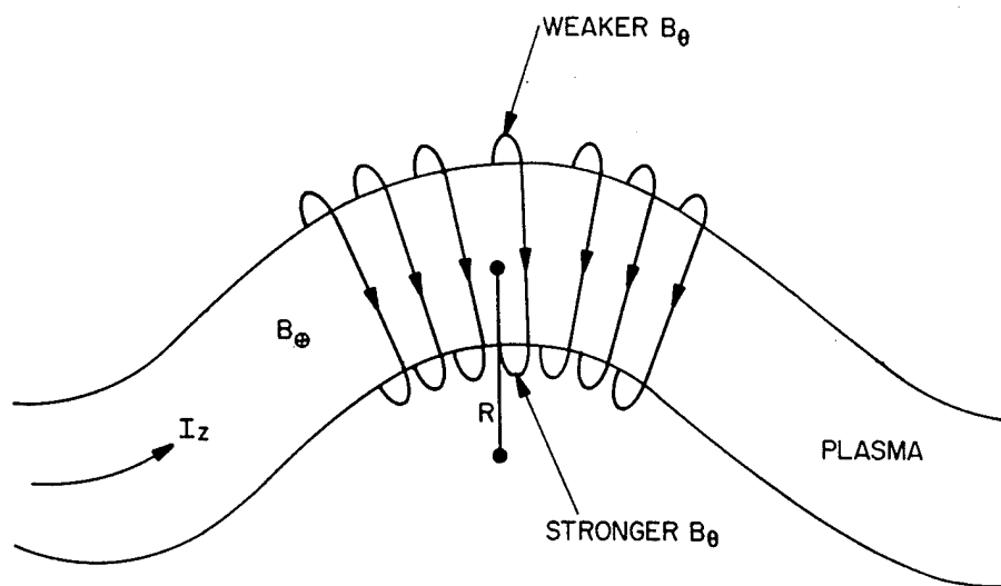
Fig. 10. Development of the kink instability in the lightning channel of Fig. 9. The helically twisted plasma looks like a single strand of multistrand rope, and the instability is driven by the stronger magnetic field on the inside radius of curvature. (Taken from Roth. 12 )
