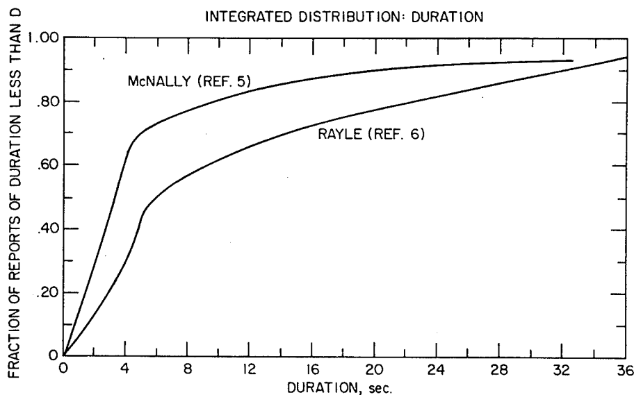
Fig. 3. Cumulative distribution function of reported ball lightning durations from the McNally 5 and the Rayle 6 surveys. (Taken from Ref. 6.)
