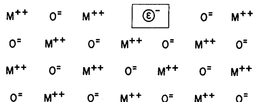
FIGURE IV-7.— S' center.
