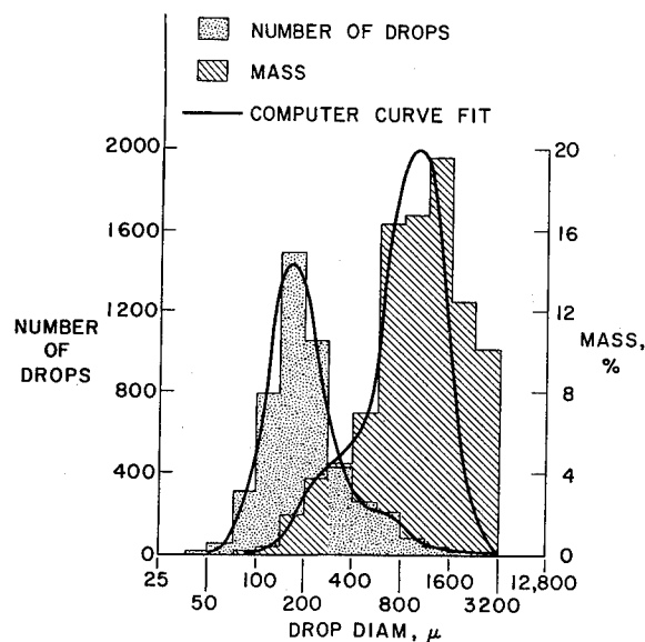
FIGURE I-13.—Drop size distribution for impinging jet spray.
