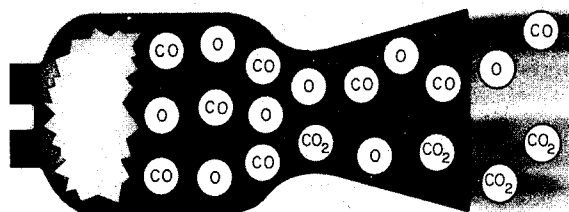
FIGURE I-5.—Chemical reaction rates.
