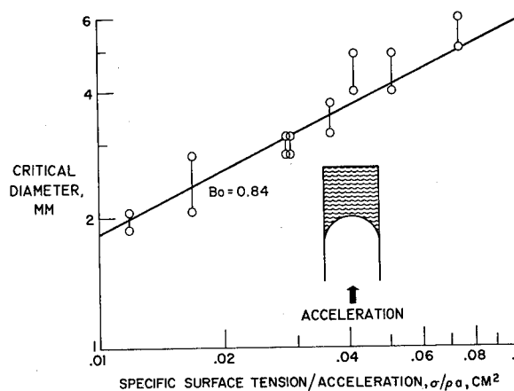
FIGURE III-23.—Stability characteristics in vertical cylinder. Acceleration, 980.2 centimeters per second per second.
