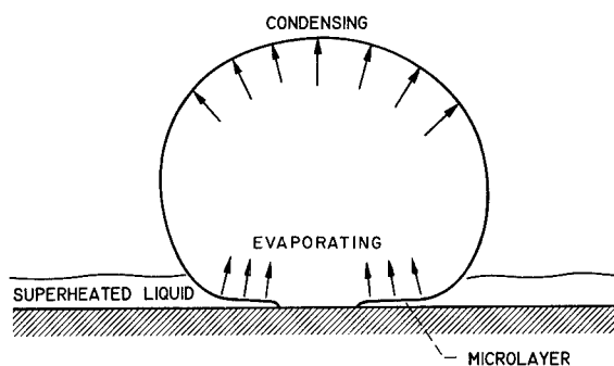
FIGURE II-22.—Microlayer evaporation heat-transfer mechanism.
