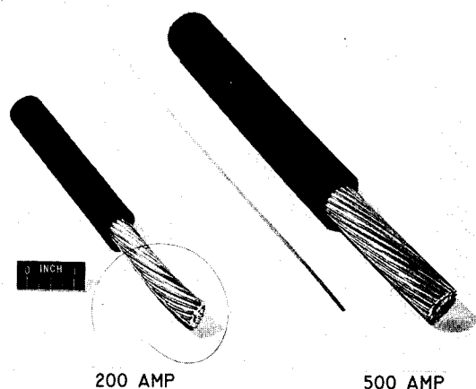
FIGURE V-14.—Current capacity.
