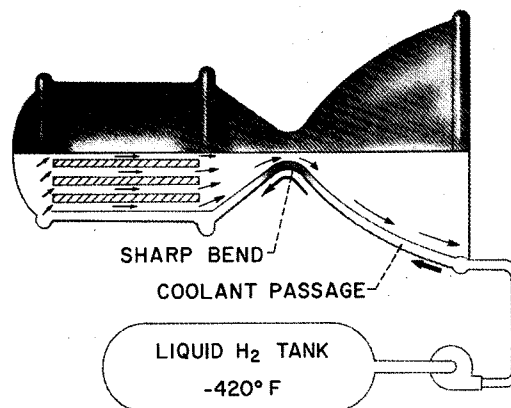
FIGURE II-10.—Sharp bend in coolant passage at nozzle throat.
