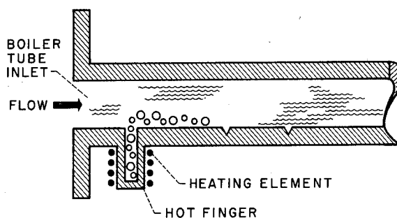
FIGURE II-33.—Nucleating device for liquid-metal boiler tube.
