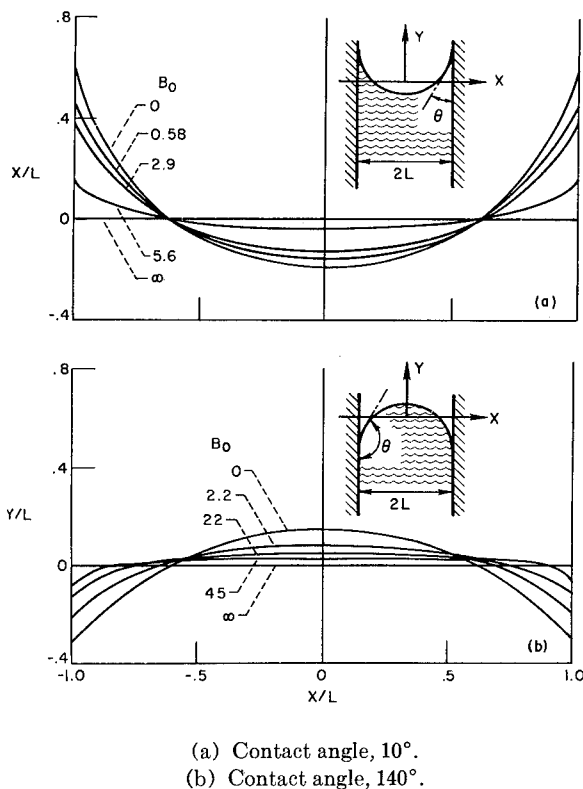
FIGURE III-11.—Calculated configuration of liquid-vapor interface between parallel plates for various Bond numbers and contact angles.
