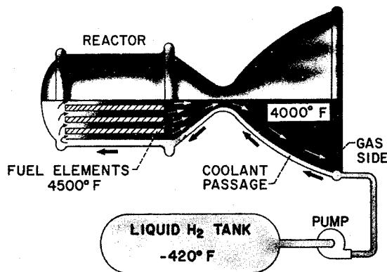
FIGURE II-1.—Nuclear rocket engine.
