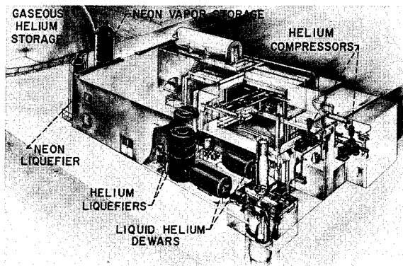
FIGURE VIII-19.—Helium liquefier.
