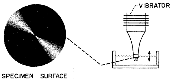
FIGURE VI-38.—Magnetostrictive cavitation damage apparatus.
