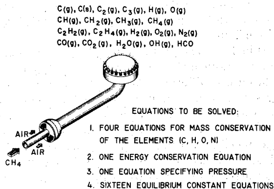
FIGURE I-6.—Combustion process.
