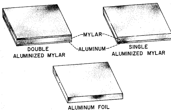
FIGURE VIII-51.—Multilayer insulation reflective shields.
