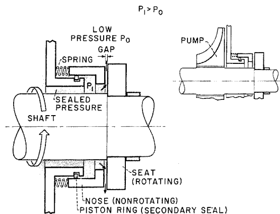
FIGURE VII-28.—Face contact seal.
