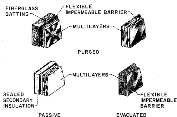
FIGURE VIII-55.—Multilayer insulation systems.
