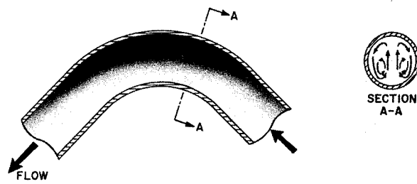
FIGURE II-11.—Density gradient and secondary flow in tube bend.
