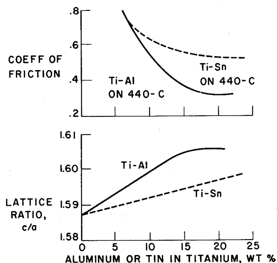
FIGURE VII-13.—Friction and lattice ratio ( c/a ) for titanium alloys. Load, 1000 grams; sliding velocity, 390 feet per minute; pressure, 10^{-10} millimeter of mercury.
