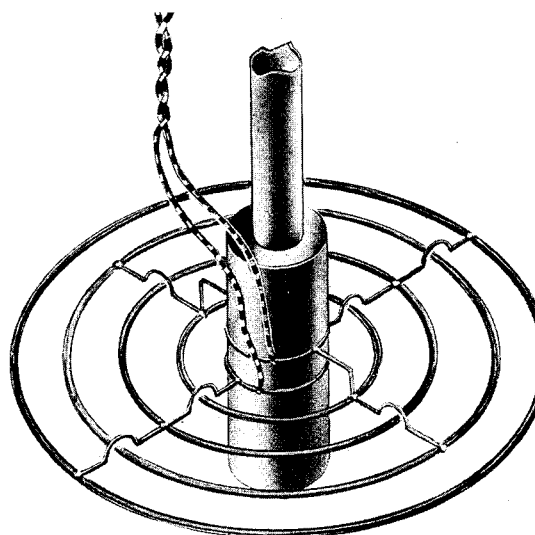
FIGURE VIII-70.—Capacitance point-level indicator.
