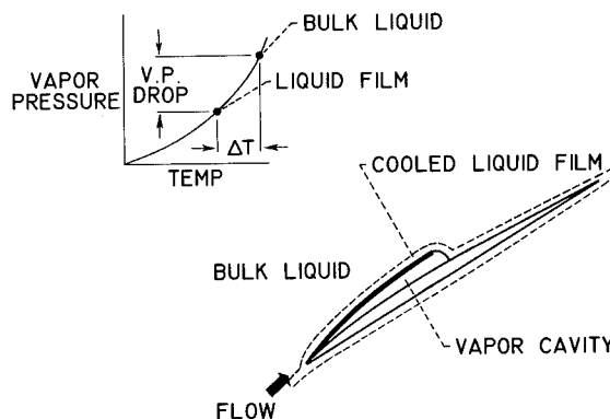
FIGURE VI-26.—Cavitation cooling.
