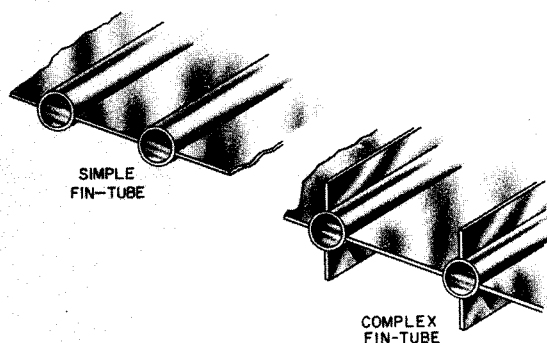
FIGURE II-37.—Fin tube configurations for space radiator.
