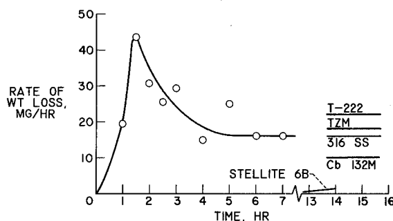
FIGURE VI-40.—Cavitation damage rate in liquid sodium at 400° F.
