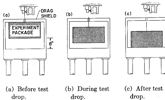
FIGURE III-6.—Zero-gravity drag shield.
