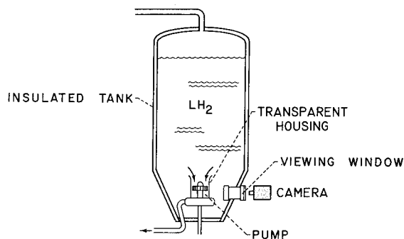
FIGURE VI-33.—Hydrogen-pump test arrangement.
