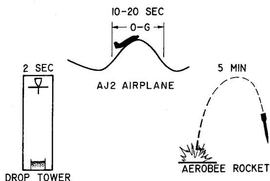
FIGURE III-3.—Zero-gravity facilities.
