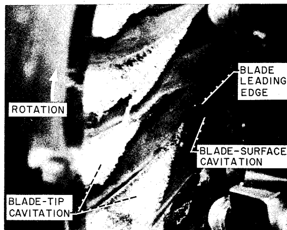
FIGURE VI-3.—Pump cavitation.
