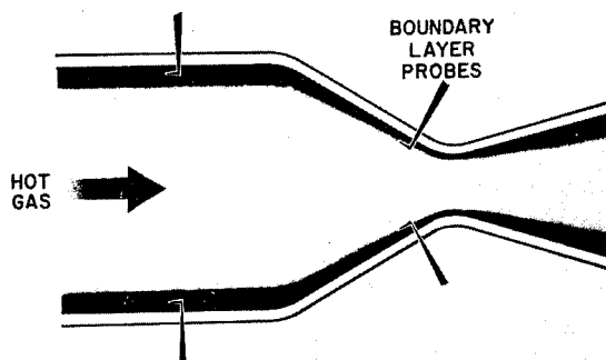
FIGURE II-5.—Experimental nozzle boundary layer facility.
