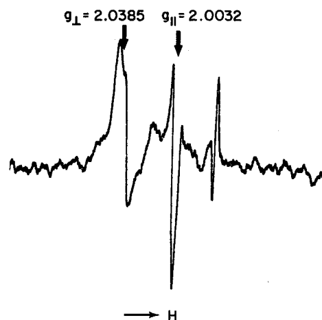
FIGURE IV-2.—Spin resonance curve of magnesium oxide catalyst degassed at 290^\circ\text{C} in vacuum and given 2537\text{ \AA} ultraviolet irradiation.
