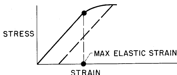
FIGURE VIII-34.—Elastic strain.
