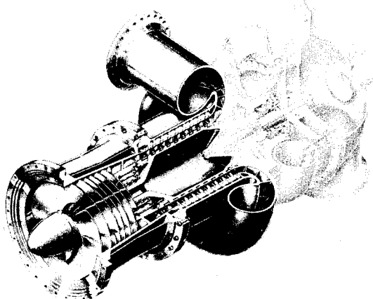
FIGURE VI-23.—Axial-flow liquid-hydrogen pump.
