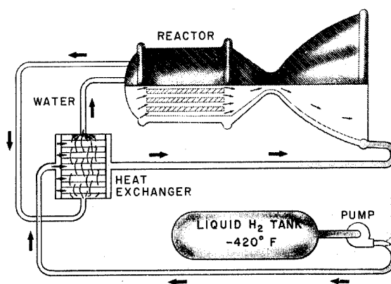
FIGURE II-14.—Liquid-hydrogen-water heat exchanger.
