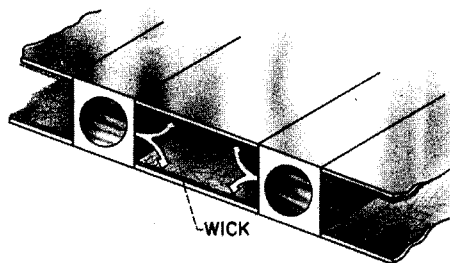
FIGURE II-38.—Use of secondary fluid to provide constant temperature fins.
