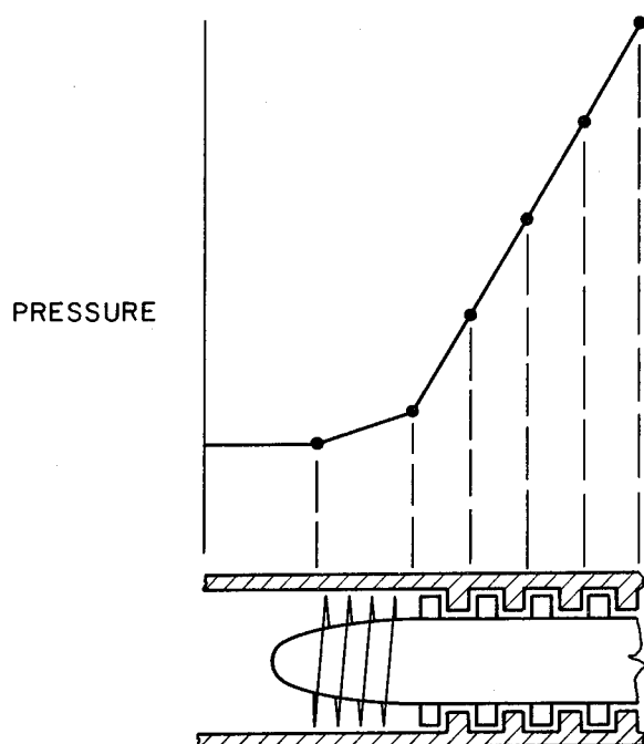
FIGURE VI-18.—Pressure rise in axial-flow pump with inducer.
