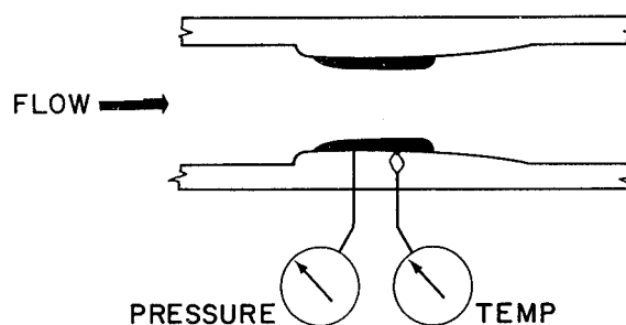
FIGURE VI-28.—Venturi with cavitation.
