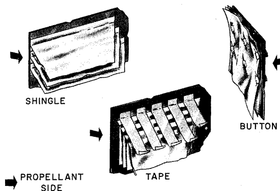
FIGURE VIII-56.—Multilayer insulation attachment methods.
