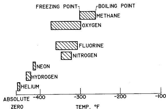
FIGURE VIII-1.—Liquid temperature range of cryogenic fluids at 1 atmosphere.
