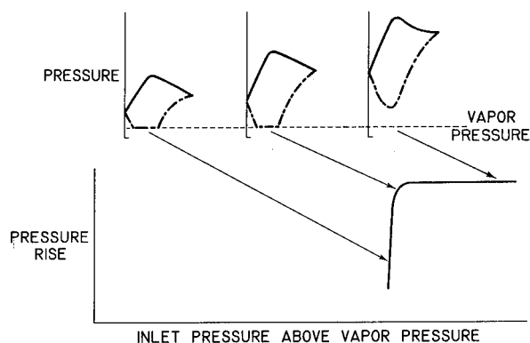
FIGURE VI-14.—Pump performance.
