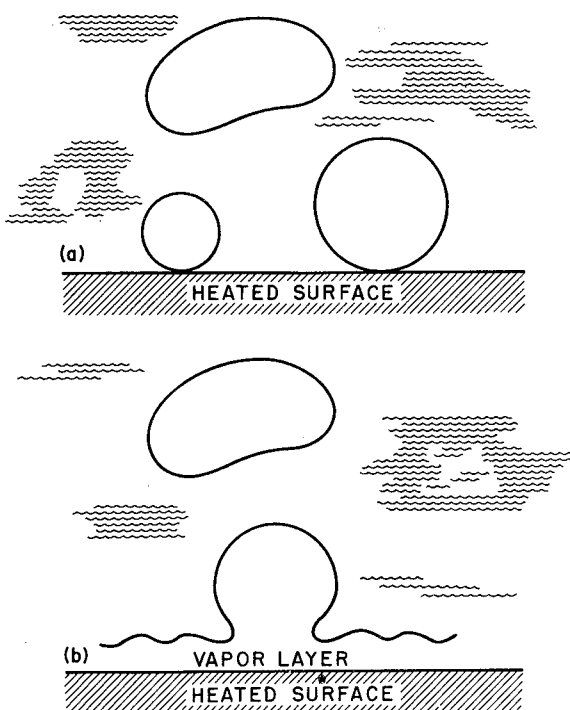
FIGURE II-20.—Bubble agitation mechanism in nucleate boiling.
