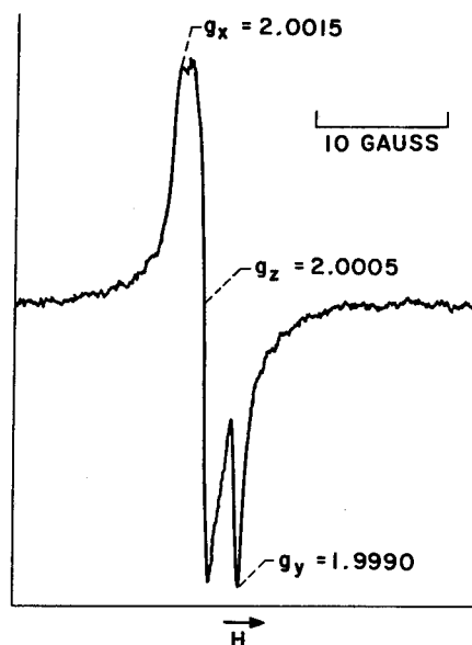
FIGURE IV-5.— S' spectrum of ultraviolet-irradiated magnesium oxide.
