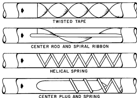
FIGURE II-26.—Centrifugal types of boiler tube inserts.
