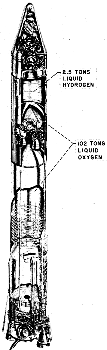
FIGURE VIII-5.—Schematic drawing of Atlas-Centaur.
