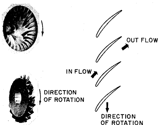
FIGURE VI-8.—Pump blades.
