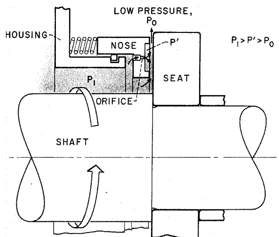
FIGURE VII-32.—Pressure compensated seal.
