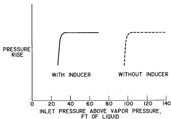
FIGURE VI-20.—Pump performance.
