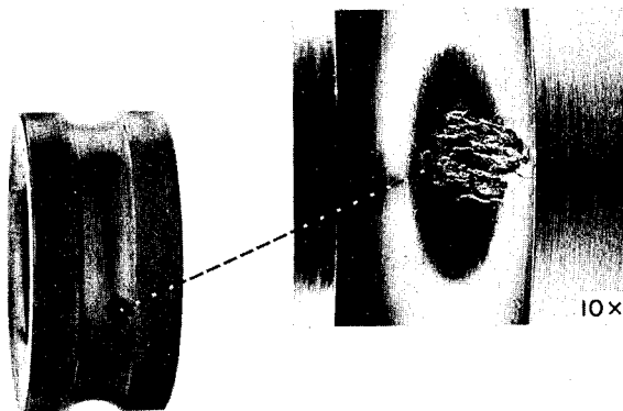
FIGURE VII-17.—Typical fatigue spall.
