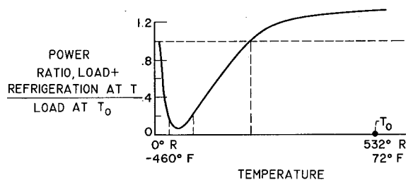
FIGURE V-5.—Power requirements of load and refrigeration plant.
