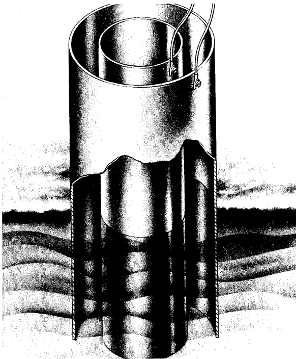
FIGURE VIII-72.—Continuous capacitance mass sensor.
