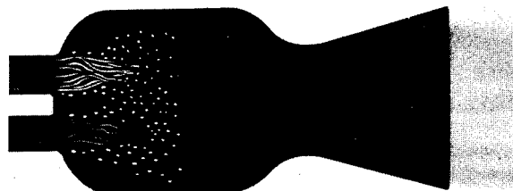
FIGURE I-3.—Atomization and vaporization.
