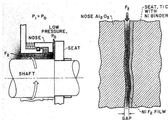
FIGURE VII-35.—Liquid fluorine seal.
