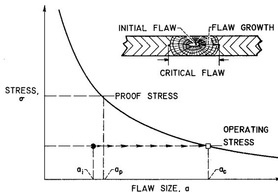
FIGURE VIII-29.—Service failure due to flaw growth.
