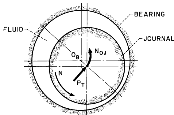
FIGURE VII-24.—Whirl instability due to unbalanced film force.
