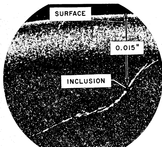
FIGURE VII-18.—Fatigue crack originating at an inclusion.
