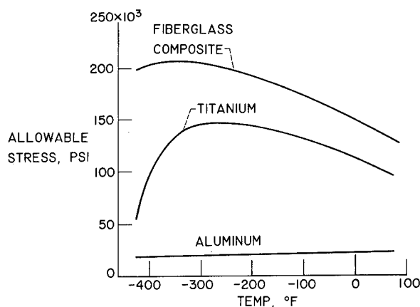
FIGURE VIII-32.—Effect of temperature on allowable strength for 3000-pound-per-square-inch pressure-vessel application.
