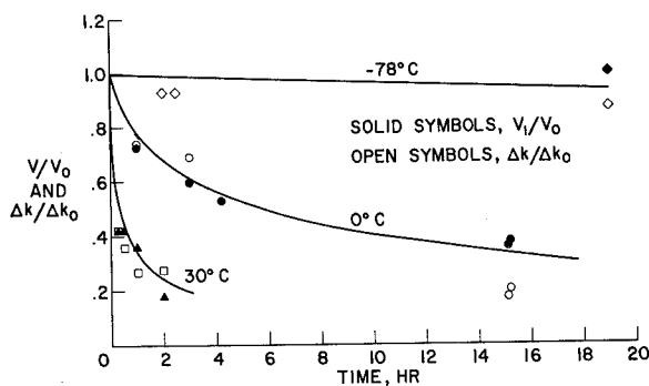
FIGURE IV-4.—Thermal decay at three temperatures following 2537 Å ultraviolet irradiation.
