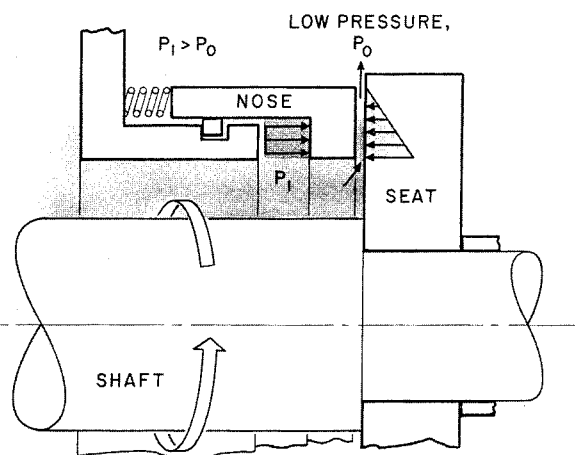
FIGURE VII-31.—Pressure balanced contact seal.
