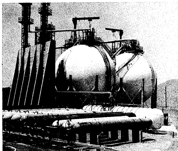
FIGURE VIII-10.—M-1 propellant storage area.
