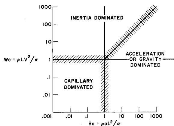
FIGURE III-2.—Hydrodynamic regimes.
