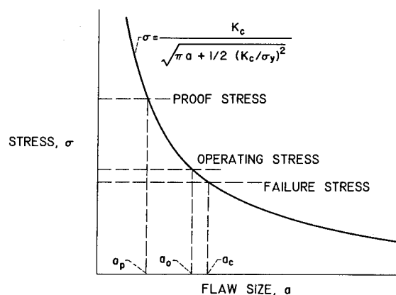
FIGURE VIII-28.—Graphical presentation of pressure vessel failure.
