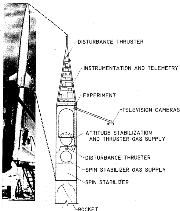
FIGURE III-10.—WASP rocket zero-gravity facility.
