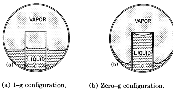
FIGURE III-15.—Capillary-type ullage control surface.
