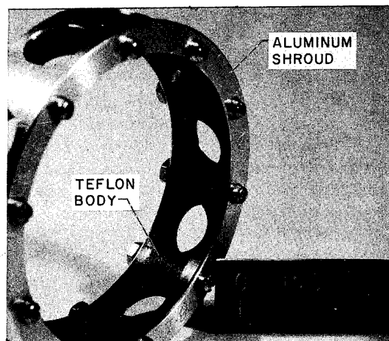
FIGURE VII-15.—Teflon—glass fiber reinforced cage.
