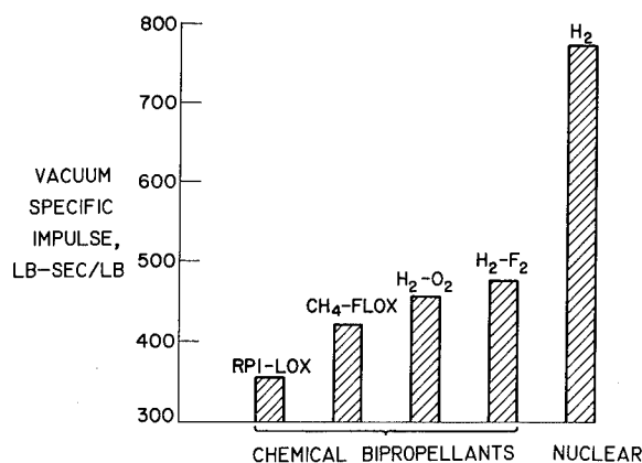
FIGURE VIII-2.—Rocket performance of cryogenic liquids.
