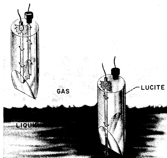
FIGURE VIII-71.—Optical point-level sensor.
