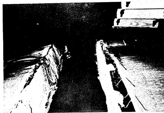
FIGURE VIII-58.—Application of multilayer insulation to ground storage tank.
