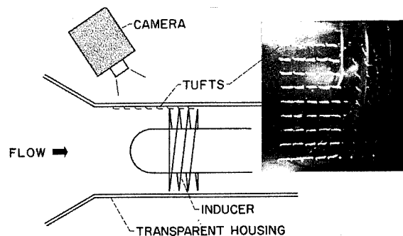
FIGURE VI-42.—Experimental arrangement for flow instability study.
