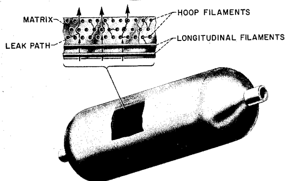
FIGURE VIII-33.—Glass-fiber-filament-wound pressure vessel.
