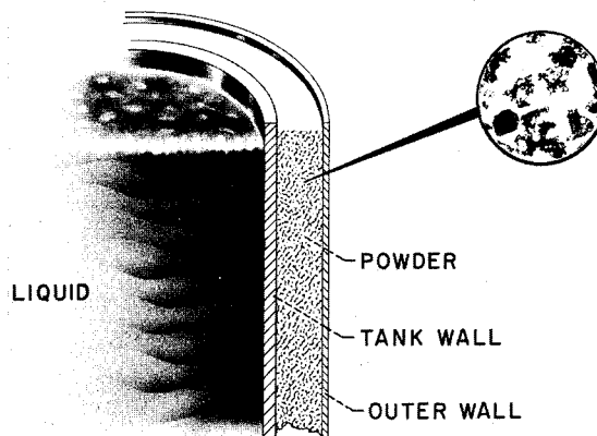
FIGURE VIII-42.—Powder insulation.
