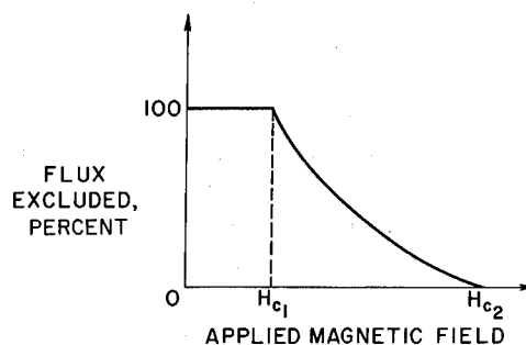
FIGURE V-13.—Flux exclusion as function of magnetic field for high-current—high-field superconductors.
