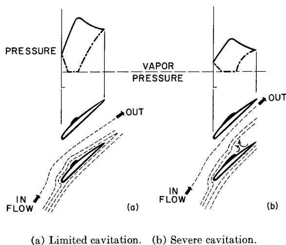
FIGURE VI-13.—Blade pressure distributions with two degrees of cavitation.
