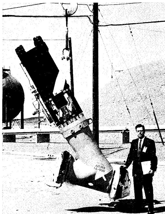
FIGURE VIII-11.—14-Inch unjacketed liquid-hydrogen valve.
