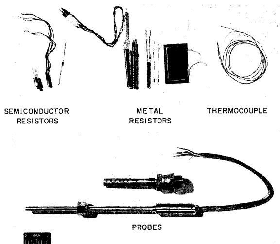
FIGURE VIII-62.—Temperature sensors.
