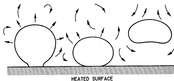
FIGURE II-20.—Bubble agitation mechanism in nucleate boiling.
