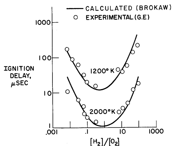
FIGURE I-18.—Hydrogen-oxygen ignition delays. Pressure, approximately 1 atmosphere.
