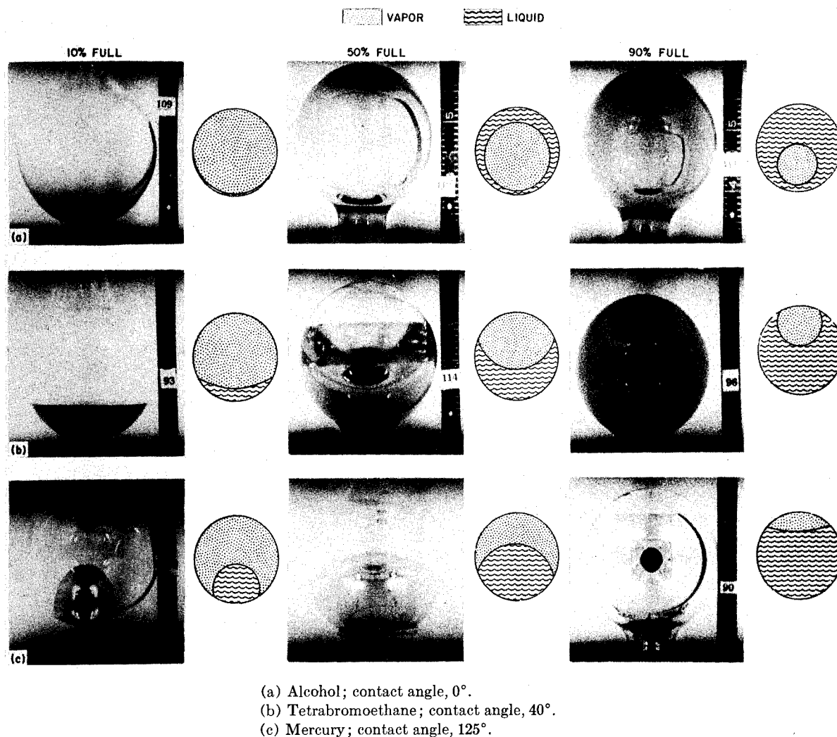
FIGURE III-13.—Configuration of liquid-vapor interface during weightlessness in spheres.
