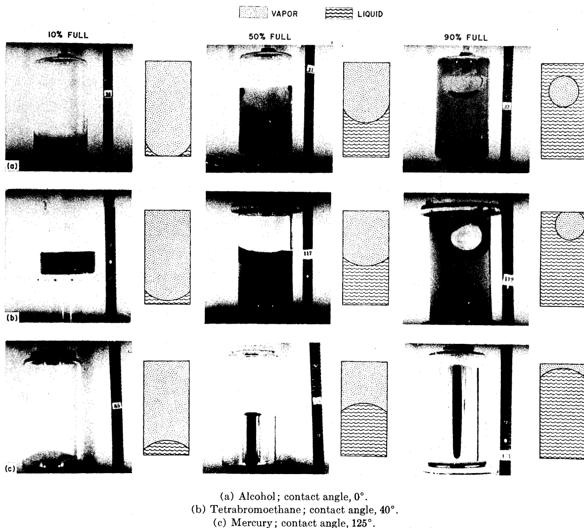
FIGURE III-14.—Configuration of liquid-vapor interface during weightlessness in cylinders.
