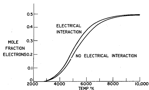
FIGURE I-7.—Mole fraction of electrons in cesium plasma.
