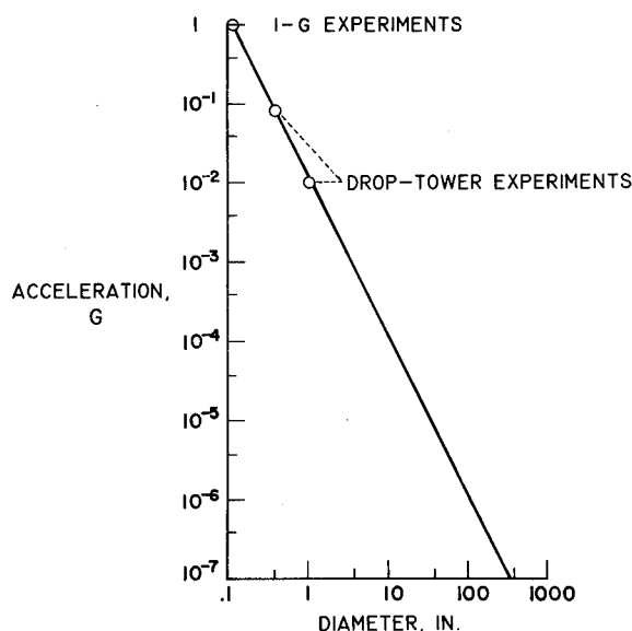
FIGURE III-27.—Interfacial stability as function of acceleration. Specific surface tension, 28.28 cubic centimeters per second. 2
