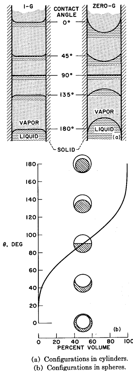
FIGURE III-12.—Weightlessness configurations in cylinders and spheres.
