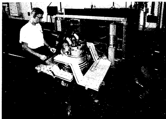
FIGURE V-16.—Water-cooled electromagnet.
