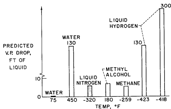
FIGURE VI-30.—Predicted vapor-pressure drops for Venturi.
