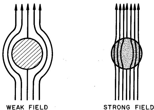
FIGURE V-12.—Magnetic field behavior of high-current—high-field superconductors.
