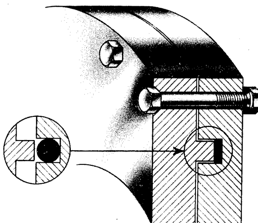
FIGURE VIII-17.—O-ring seal design for cryogenic applications.
