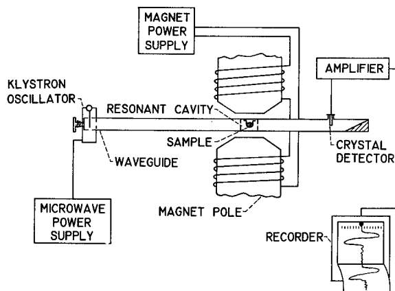
FIGURE IV-1.—Electron paramagnetic resonance apparatus.
