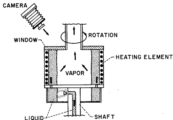
FIGURE II-25.—Rotating boiler experiment.
