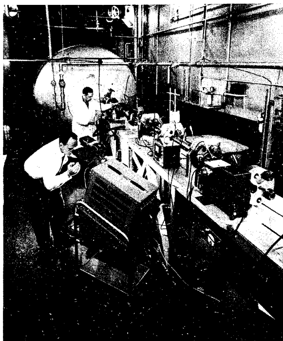
FIGURE I-23.—Shock tube for recombination studies.
