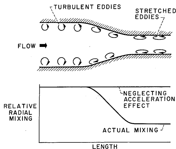
FIGURE II-7.—Effect of flow contraction on radial turbulent mixing.
