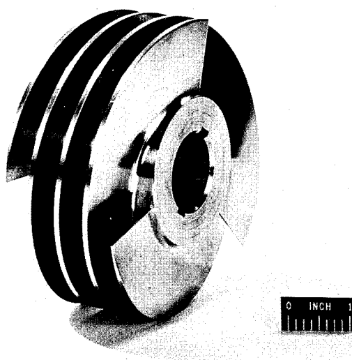
FIGURE VI-16.—Inducer.
