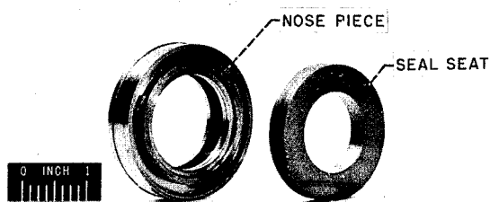
FIGURE VII-29.—Face contact seal components.
