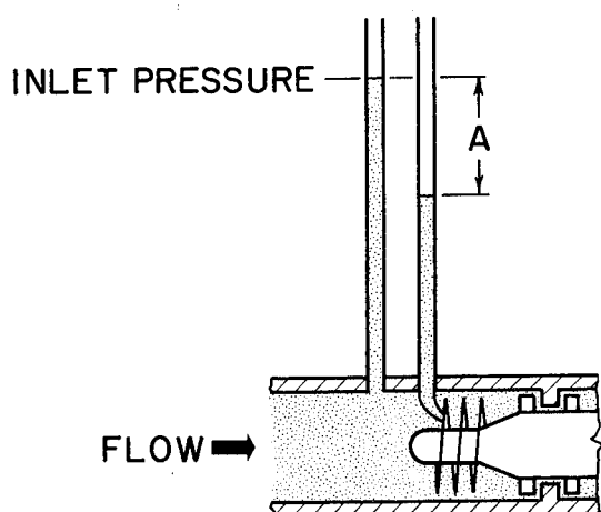
FIGURE VI-24.—Schematic pressure measurements.
