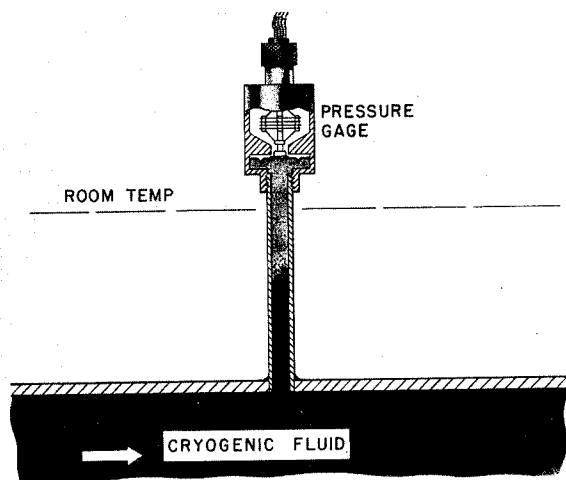
FIGURE VIII-63.—Cryogenic fluid pressure measurement. Conventional pressure-gage installation.
