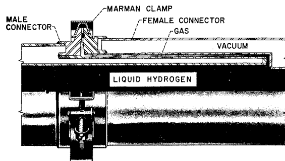
FIGURE VIII-15.—Liquid-hydrogen bayonet-type low-temperature joint.
