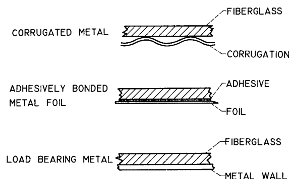
FIGURE VIII-35.—Liner concepts.
