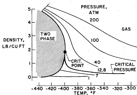
FIGURE II-9.—Density of normal hydrogen as function of temperature and pressure.
