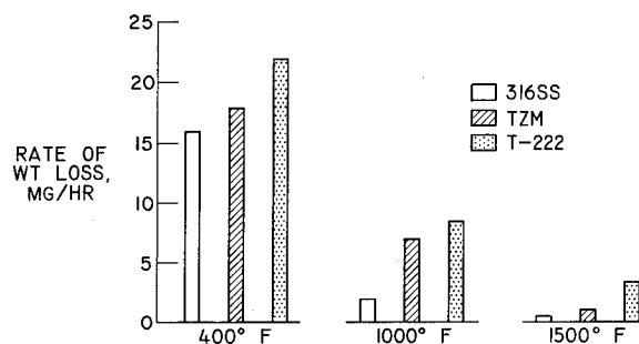
FIGURE VI-41.—Effect of temperature on cavitation damage rate in liquid sodium.
