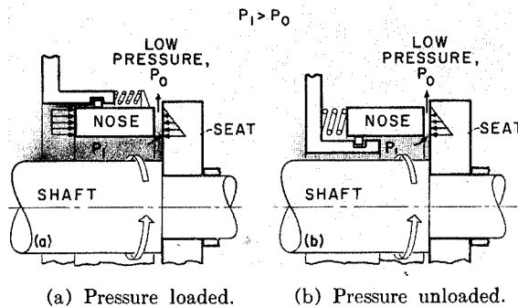
FIGURE VII-30.—Unbalanced face contact seals.
