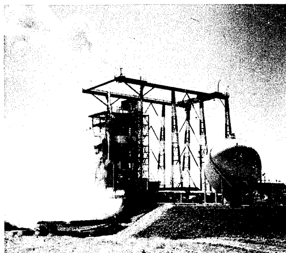
FIGURE VIII-8.—Saturn S-IV stage ground test facility.
