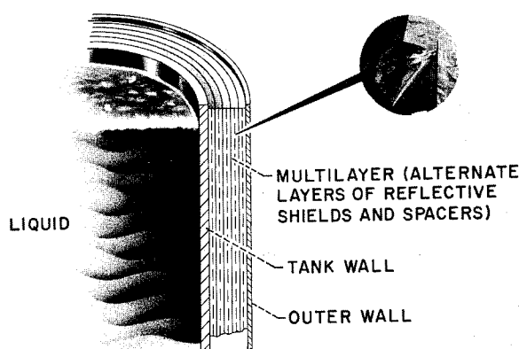
FIGURE VIII-43.—Multilayer insulation.
