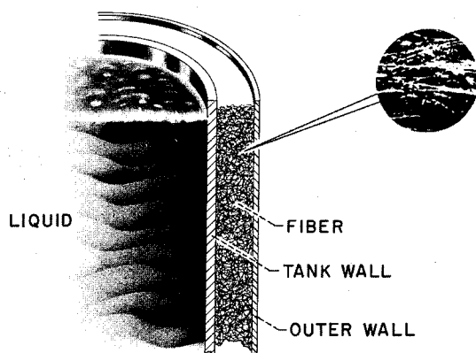
FIGURE VIII-41.—Fiber insulation.
