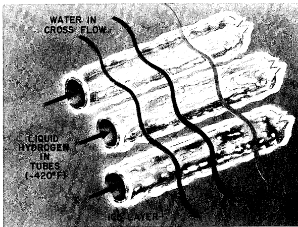
FIGURE II-16.—Ice formation on tubes in liquid hydrogen-water heat exchanger.
