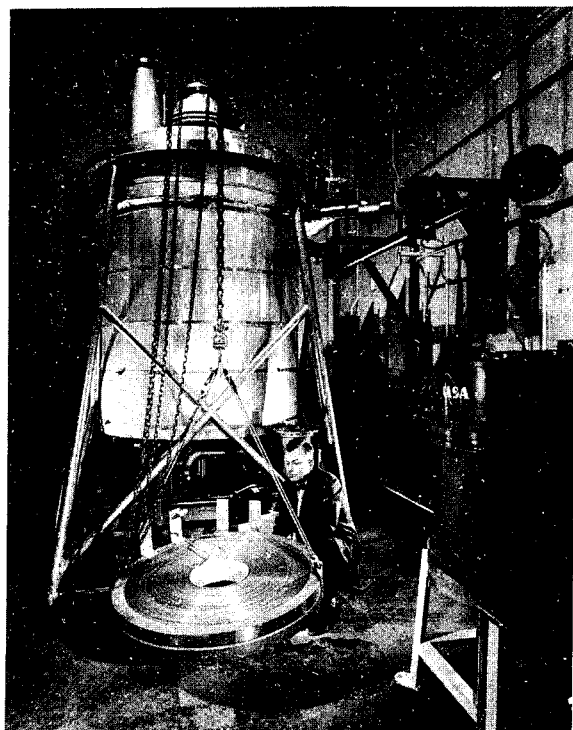
FIGURE V-6.—Cryogenic magnet.
