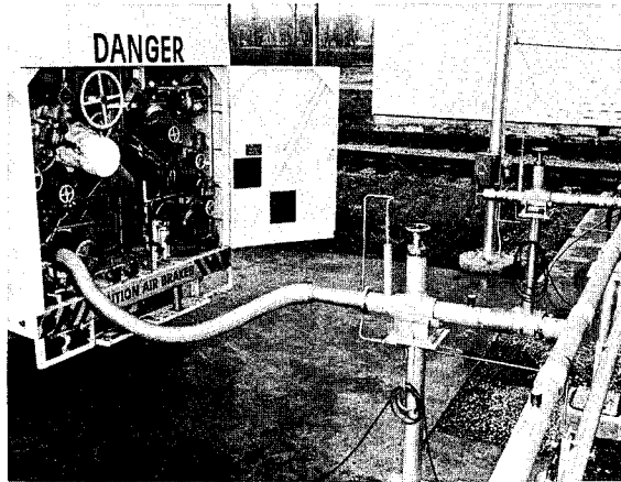
FIGURE VIII-14.—Flow line components.
