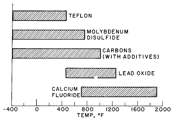
FIGURE VII-7.—Useful temperature ranges of self-lubricating materials.
