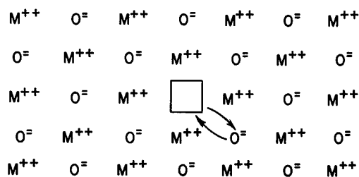
FIGURE IV-9.—Diffusion of oxygen in magnesium oxide.
