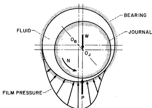
FIGURE VII-2.—Journal bearing under load.
