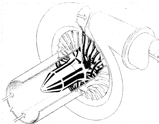
FIGURE VI-5.—Centrifugal pump.
