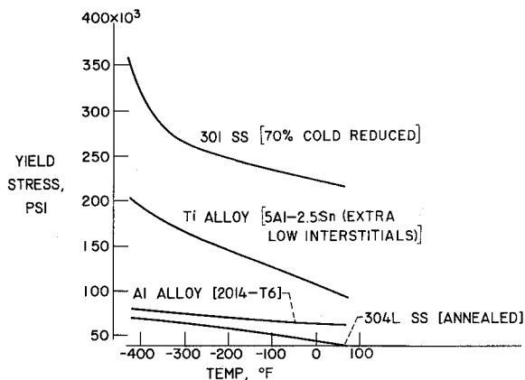
FIGURE VIII-22.—Effect of temperature on yield stress of structural alloys.
