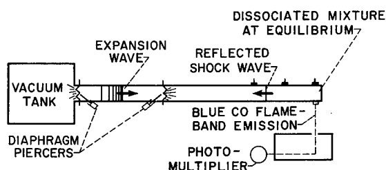
FIGURE I-24.—Recombination of carbon monoxide and oxygen in expansion waves.
