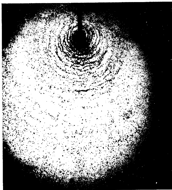
FIGURE I-12.—Spray from impinging water jets.
