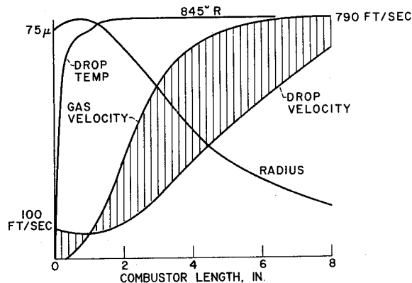
FIGURE I-15.—Calculated vaporization process for uniform heptane drops.
