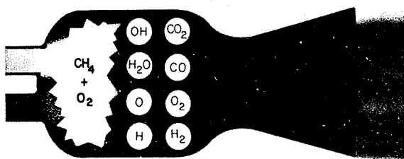
FIGURE I-1.—Chemical thermodynamics.
