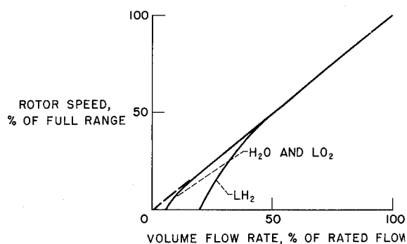
FIGURE VIII-68.—Turbine flowmeters.
