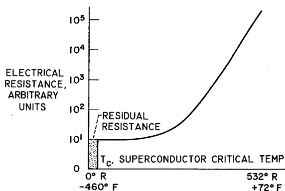
FIGURE V-1.—Resistance of conductors.
