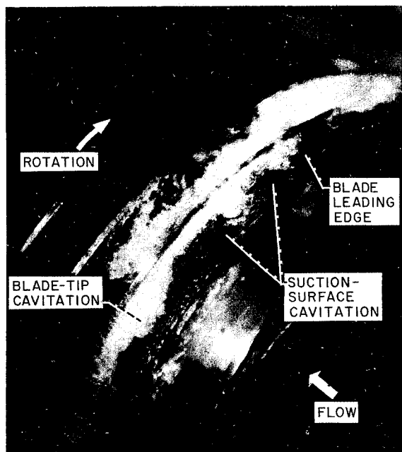
FIGURE VI-21.—Cavitating inducer.
