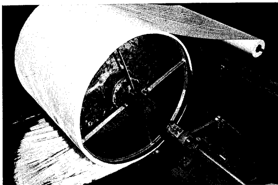
FIGURE VIII-45.—Machine winding of multilayer insulation on small tank. (Courtesy Linde Div., Union Carbide Corp.)
