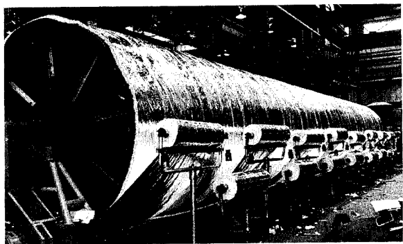
FIGURE VIII-44.—Machine winding of multilayer insulation on large tank. (Courtesy Linde Div., Union Carbide Corp.)
