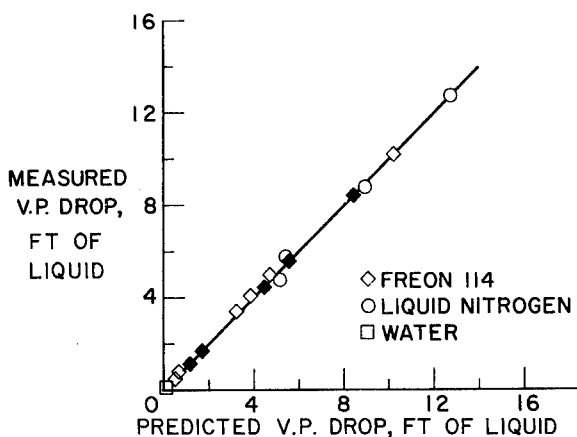
FIGURE VI-29.—Prediction of vapor-pressure drop.
