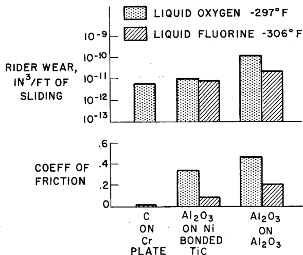
FIGURE VII-34.—Friction and wear of potential seal materials. Sliding velocity, 2300 feet per minute; load, 1000 grams.
