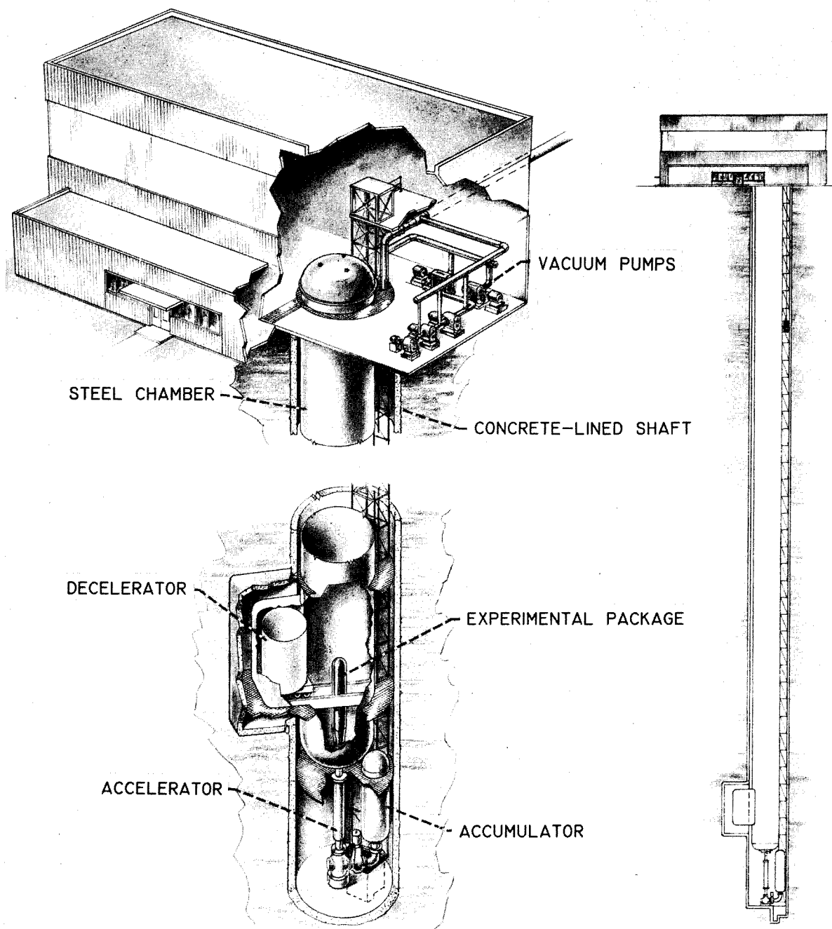
FIGURE III-7.—400-Foot zero-gravity drop facility (perspective cutaway view).
