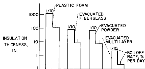
FIGURE VIII-47.—Insulation requirements for 10-foot-diameter liquid-hydrogen tank.
