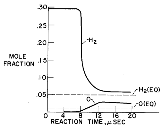
FIGURE I-16.—Characteristics of hydrogen-oxygen ignition reaction for hydrogen burning in air at 1 atmosphere and 1700° K.
