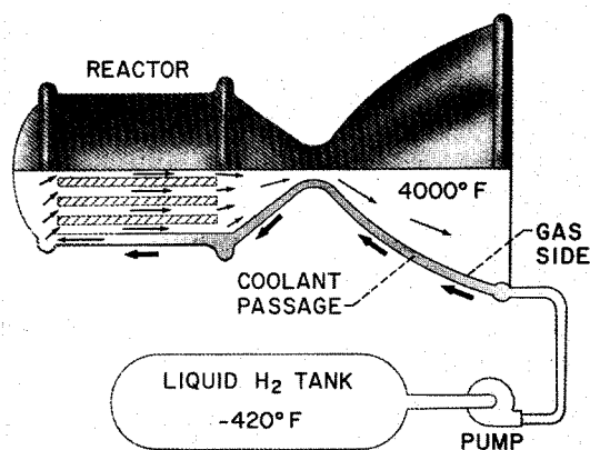
FIGURE II-8.—Coolant passages in rocket nozzle wall.
