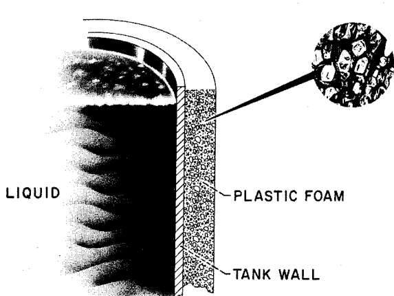
FIGURE VIII-40.—Plastic-foam insulation.
