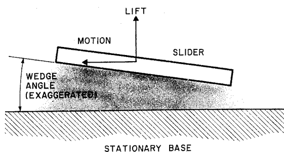
FIGURE VII-3.—Slider bearing wedge film.
