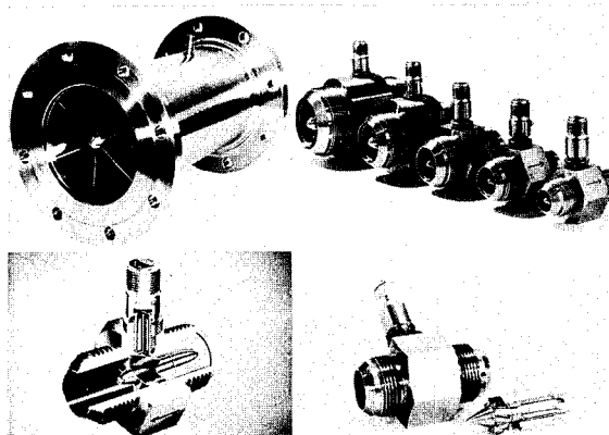
FIGURE VIII-67.—Turbine meter fluid calibration.
