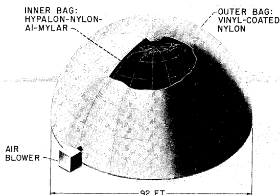
FIGURE VIII-20.—Helium gas holder. Helium capacity, 200 000 standard cubic feet.
