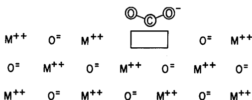
FIGURE IV-8.—Carbon dioxide adsorbed on S' center.
