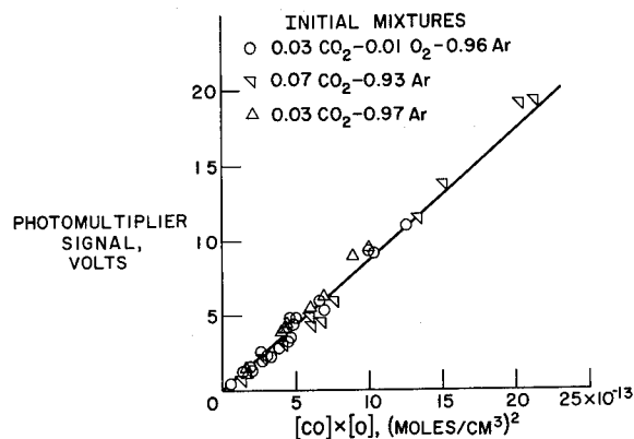
FIGURE I-26.—Flame-band intensity in equilibrium mixtures behind reflected shocks. Temperature, 3000° to 3600° K; pressure, 8 to 22 atmospheres; \text{CO} + \text{O} \rightarrow \text{CO}_2^* \rightarrow \text{CO}_2 + h\nu .
