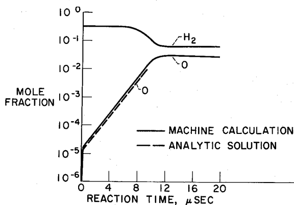
FIGURE I-17.—Semilogarithmic plot of characteristics of hydrogen-oxygen ignition reaction for hydrogen burning in air at 1 atmosphere and 1700° K.
