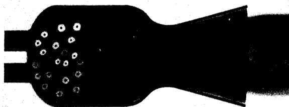
FIGURE I-2.—Transport properties.
