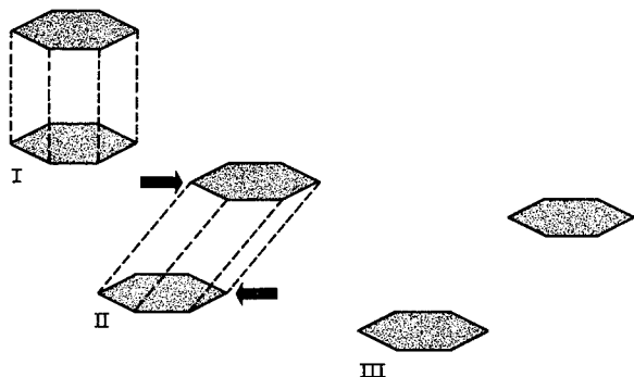
FIGURE VII-10.—Displacement of planes in hexagonal crystals with shear.
