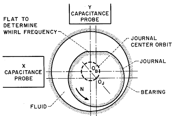
FIGURE VII-25.—Instrumentation for studying bearing whirl.
