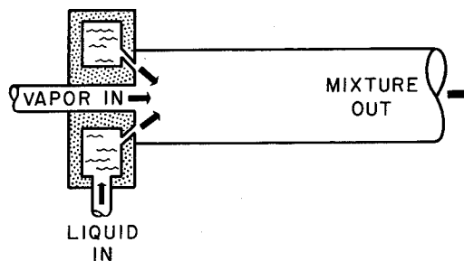
FIGURE II-24.—Jet mixing of liquid and vapor to demonstrate two-phase instabilities.
