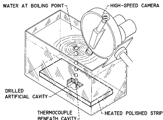
FIGURE II-31.—Experimental study of bubble nucleation from artificial cavities.
