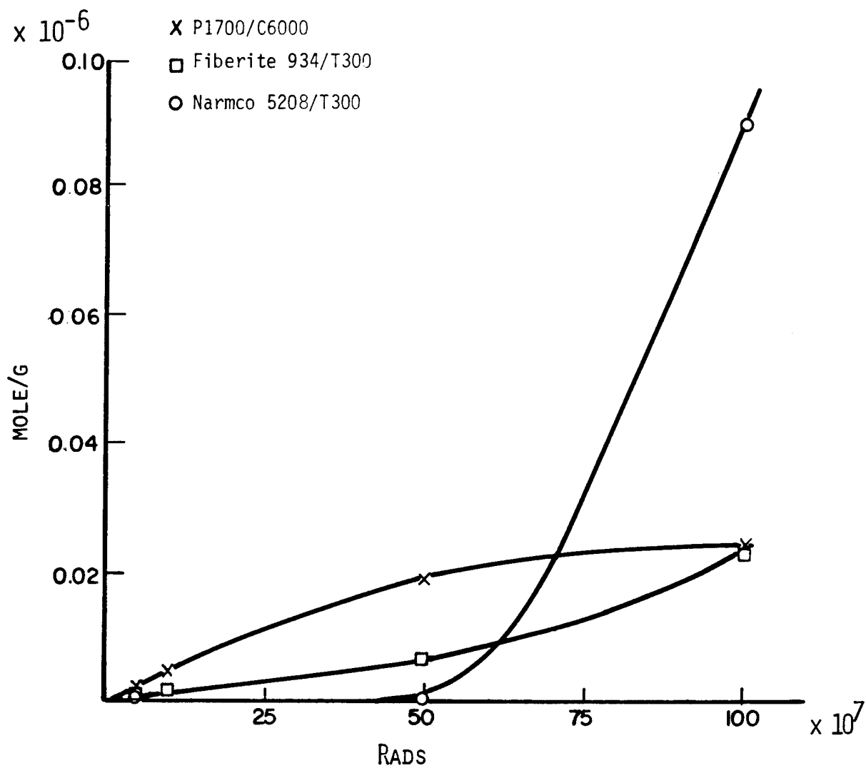
Figure 24. Ethane formation during electron radiation exposure.
