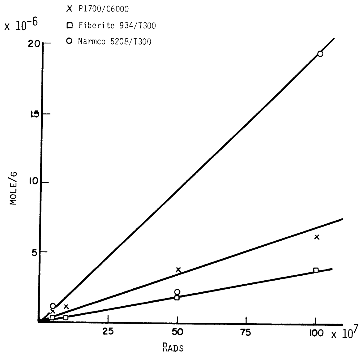
Figure 26. Carbon monoxide formation during electron radiation exposure.
