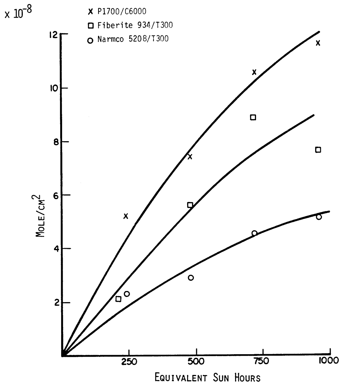
Figure 21. Carbon dioxide formation during ultraviolet radiation exposure.
