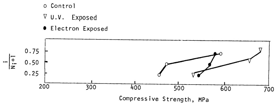
Figure 30. Compressive Strength Distribution for 934/T300
