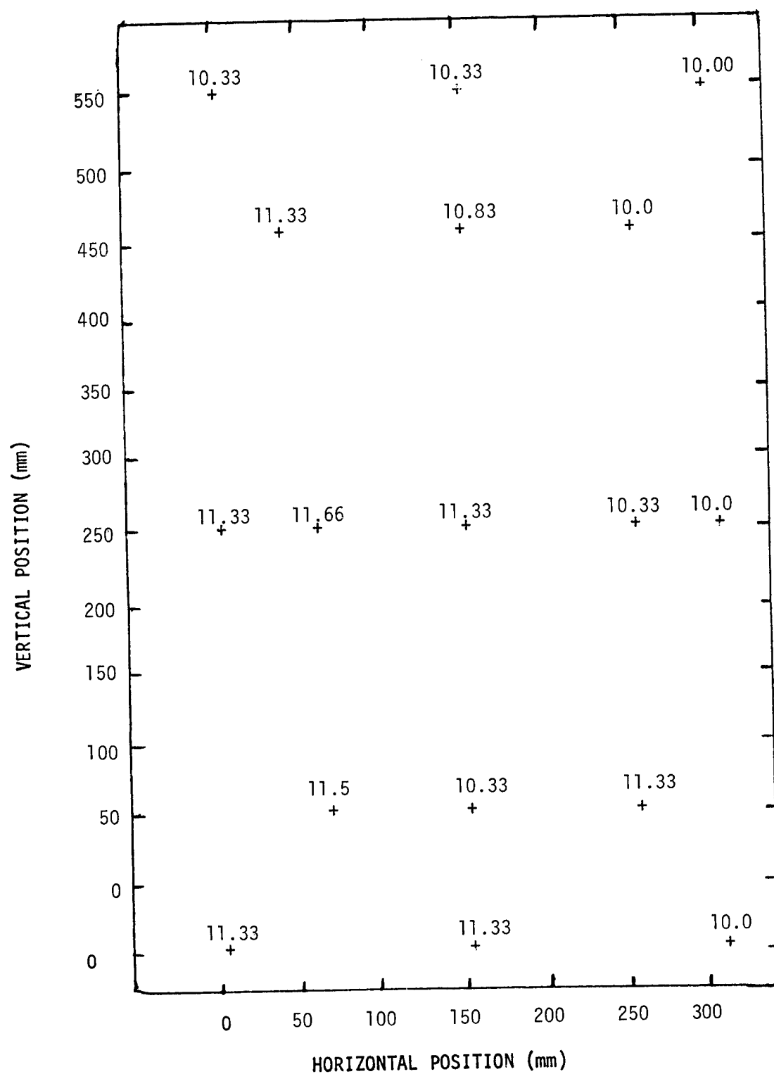
Figure 10. Dose rate map over the irradiation plane. Dose rates in krads/s.
