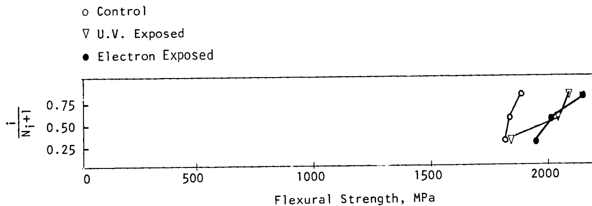
Figure 35. Flexural Strength Distribution for 5208/T300
