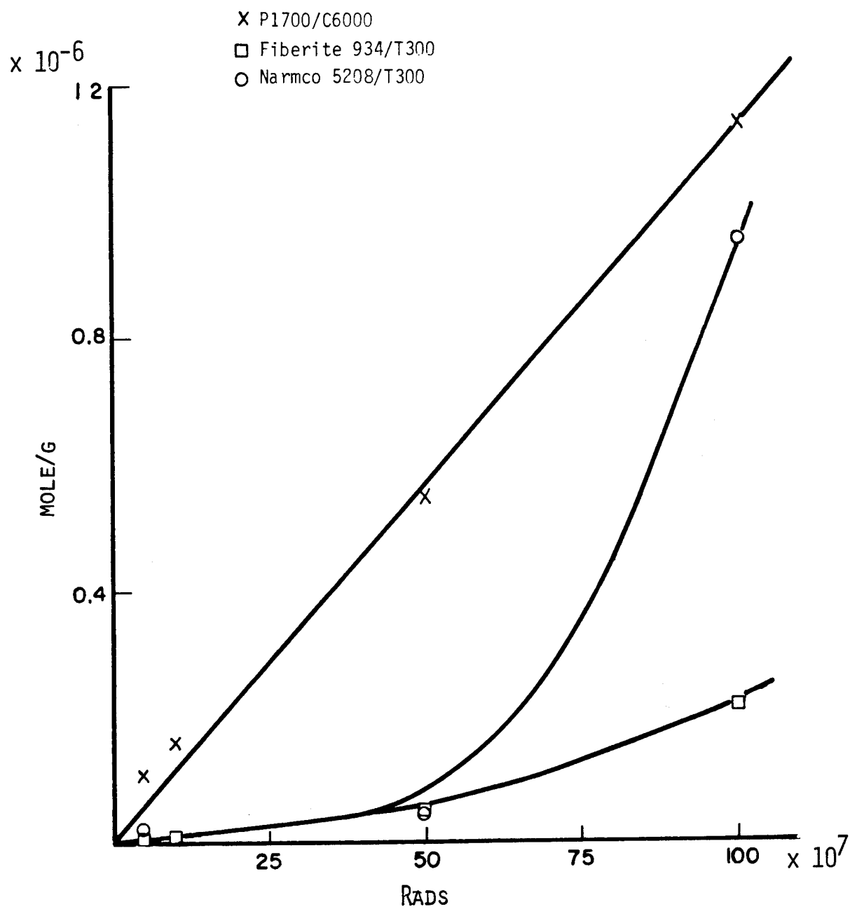
Figure 23. Methane formation during electron radiation exposure.
