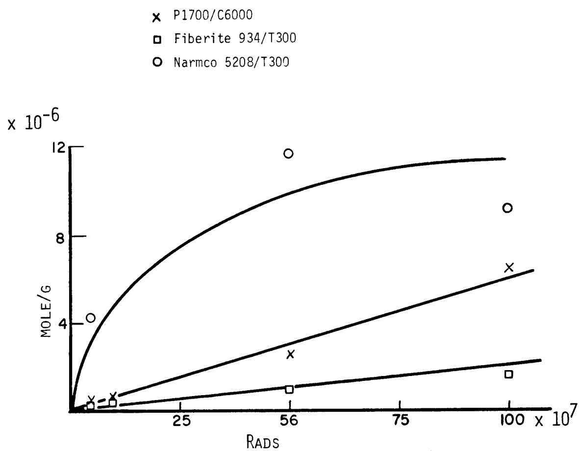
Figure 27. Carbon dioxide formation during electron radiation exposure.
