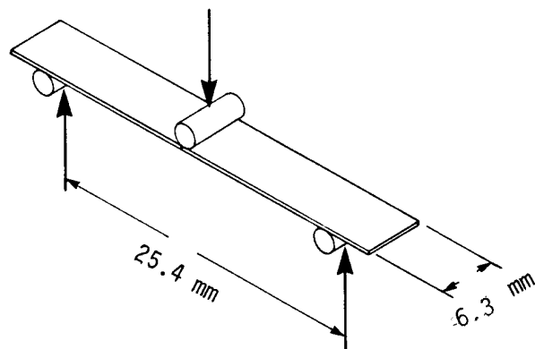
Figure 15. Flexural Specimen Geometry
