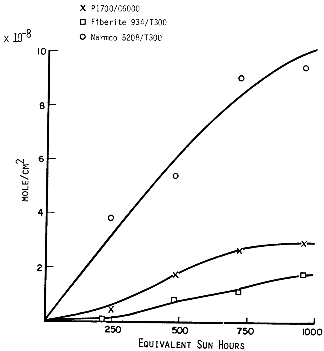
Figure 16. Hydrogen formation during ultraviolet radiation exposure.
