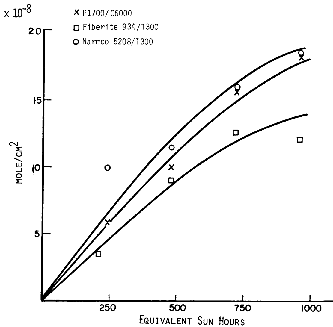
Figure 20. Carbon monoxide formation during ultraviolet radiation exposure.
