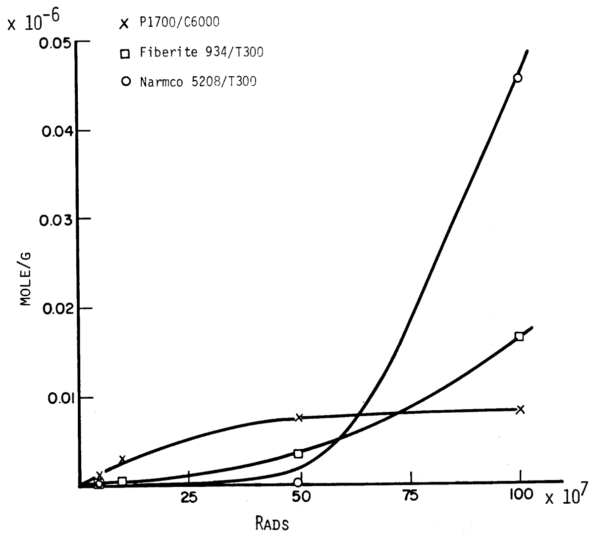
Figure 25. Propane formation during electron radiation exposure.
