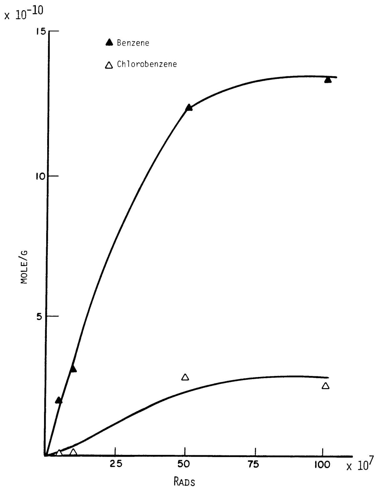
Figure 29. Benzene and Chlorobenzene formation during electron irradiation of P1700/C6000.
