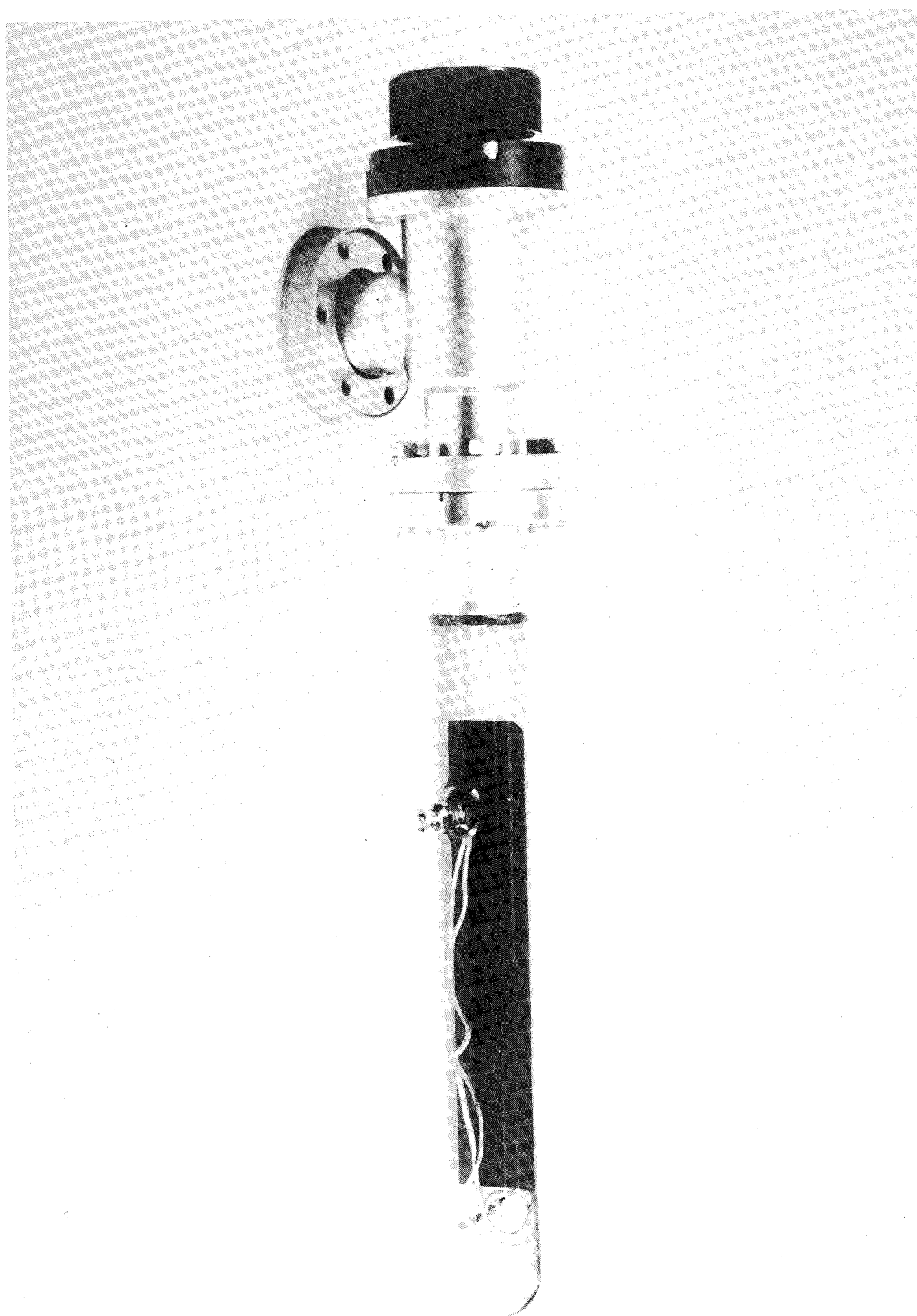
Figure 6. Vacuum Assembly for High-Energy Electron Exposure and Sample Temperature Monitoring
