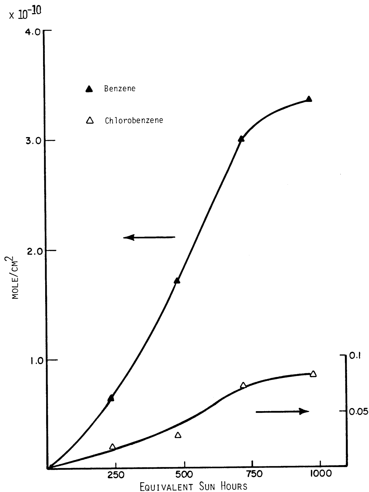
Figure 28. Benzene and chlorobenzene formation during ultraviolet irradiation of P1700/C6000.
