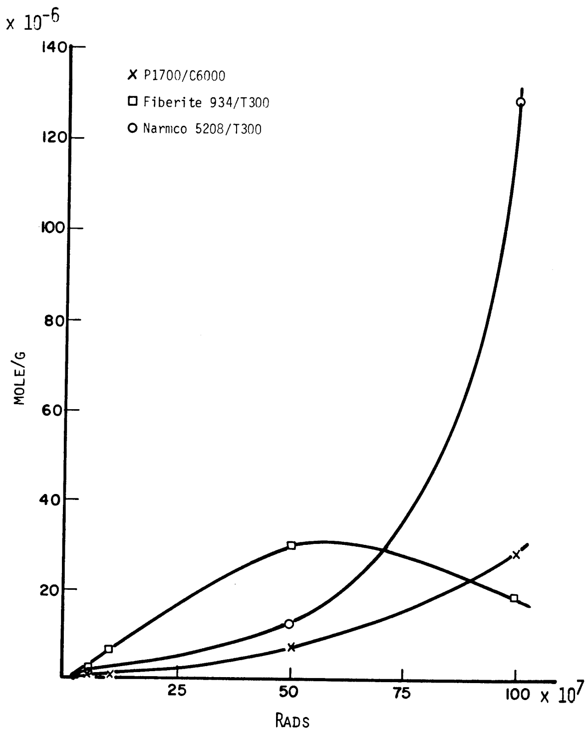
Figure 22. Hydrogen formation during electron radiation exposure.
