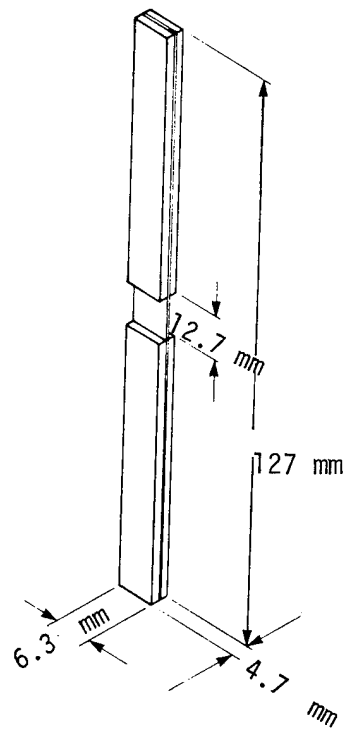
Figure 14. Compression Specimen Geometry
