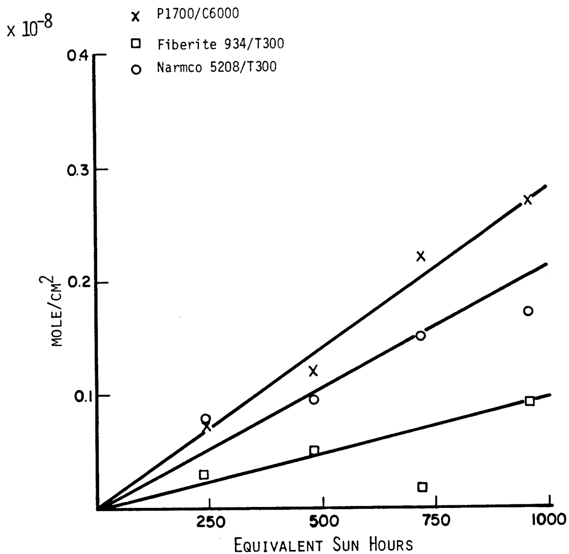
Figure 19. Propane formation during ultraviolet radiation exposure.
