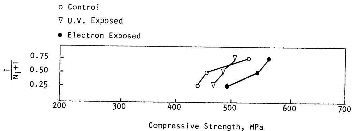
Figure 32. Compressive Strength Distribution for 5208/T300
