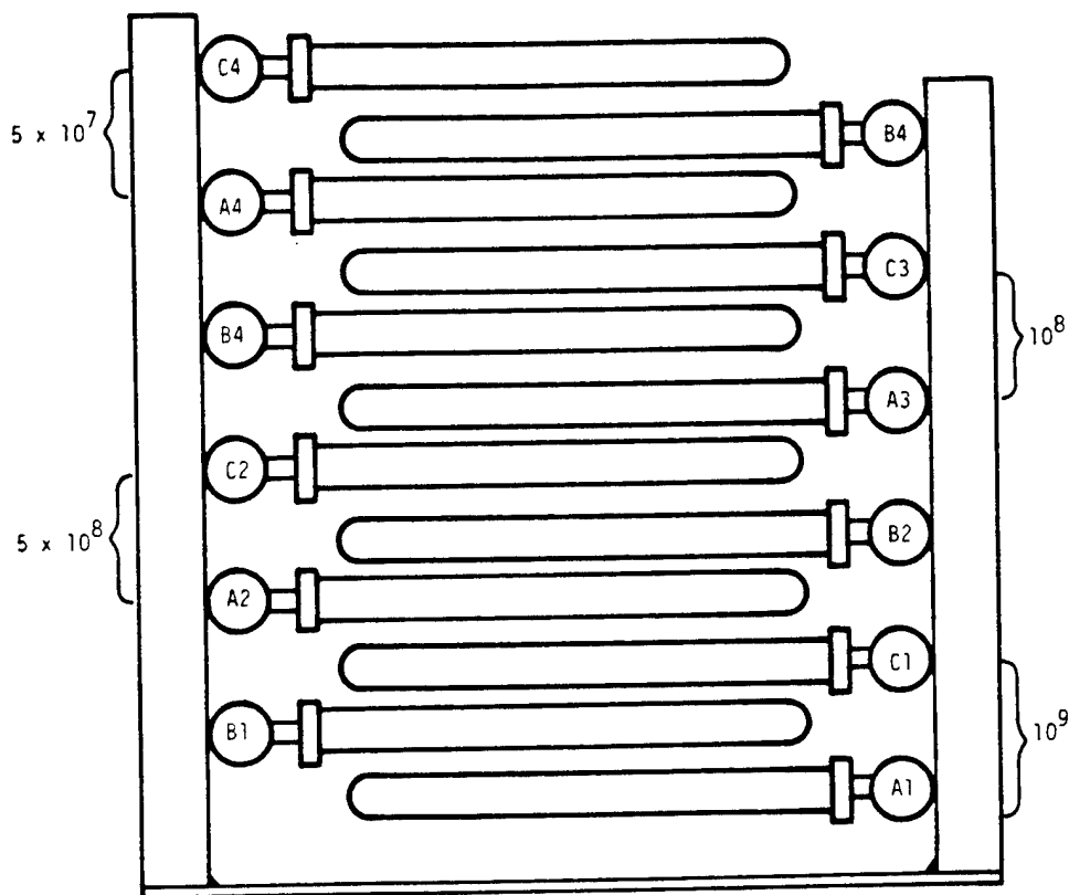
Figure 8. Irradiation configuration for composite samples. Sample position is indicated as is the total dose (rads) received.
