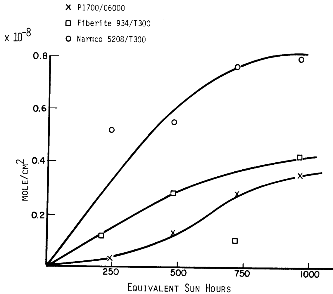
Figure 18. Ethane formation during ultraviolet radiation exposure.
