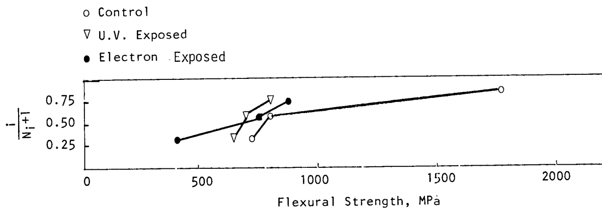
Figure 34. Flexural Strength Distribution for P1700/C6000
