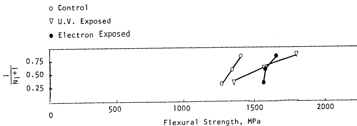
Figure 33. Flexural Strength Distribution for 934/T300
