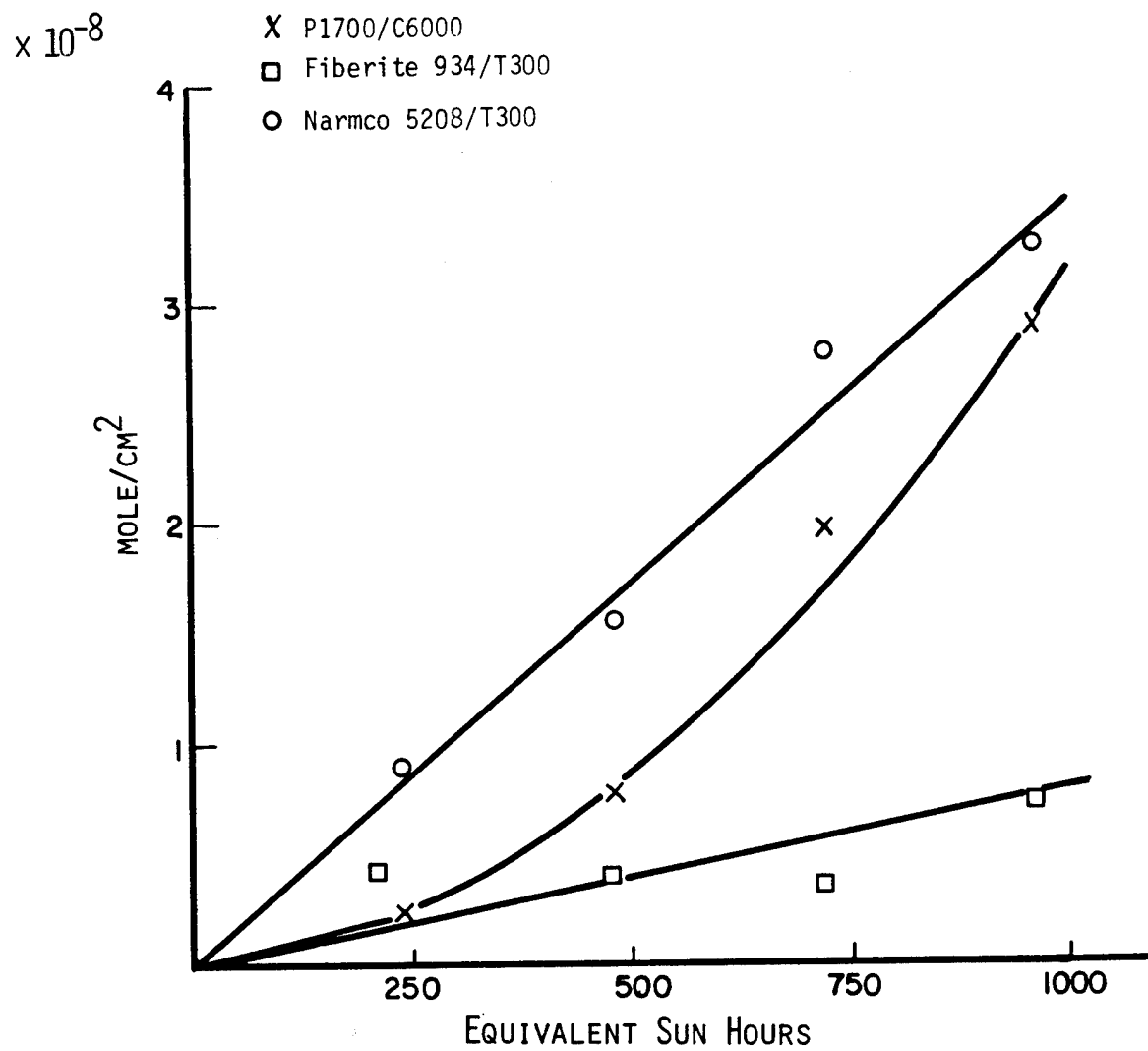
Figure 17. Methane formation during ultraviolet radiation exposure.
