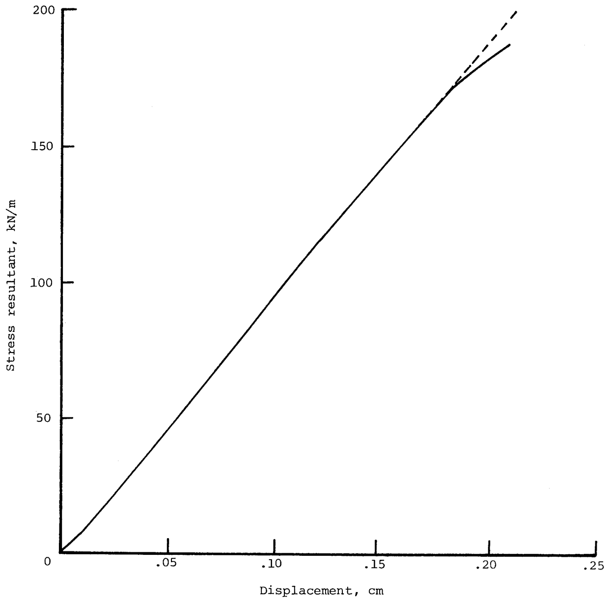
Figure 14.- End shortening as function of applied load for panel 1-36.
