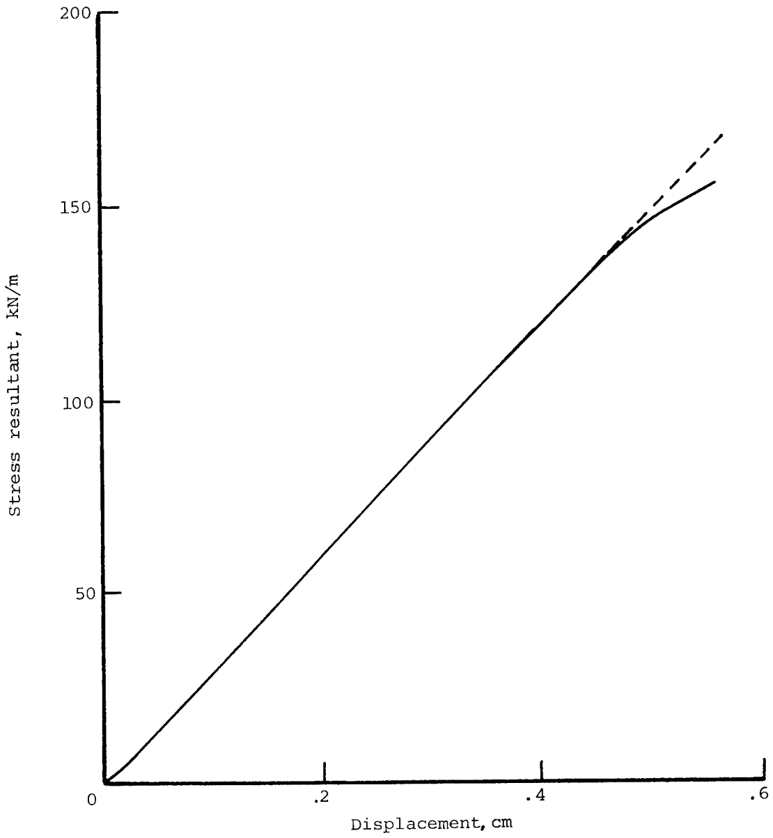
Figure 16.- End shortening as function of applied load for panel 1-100.
