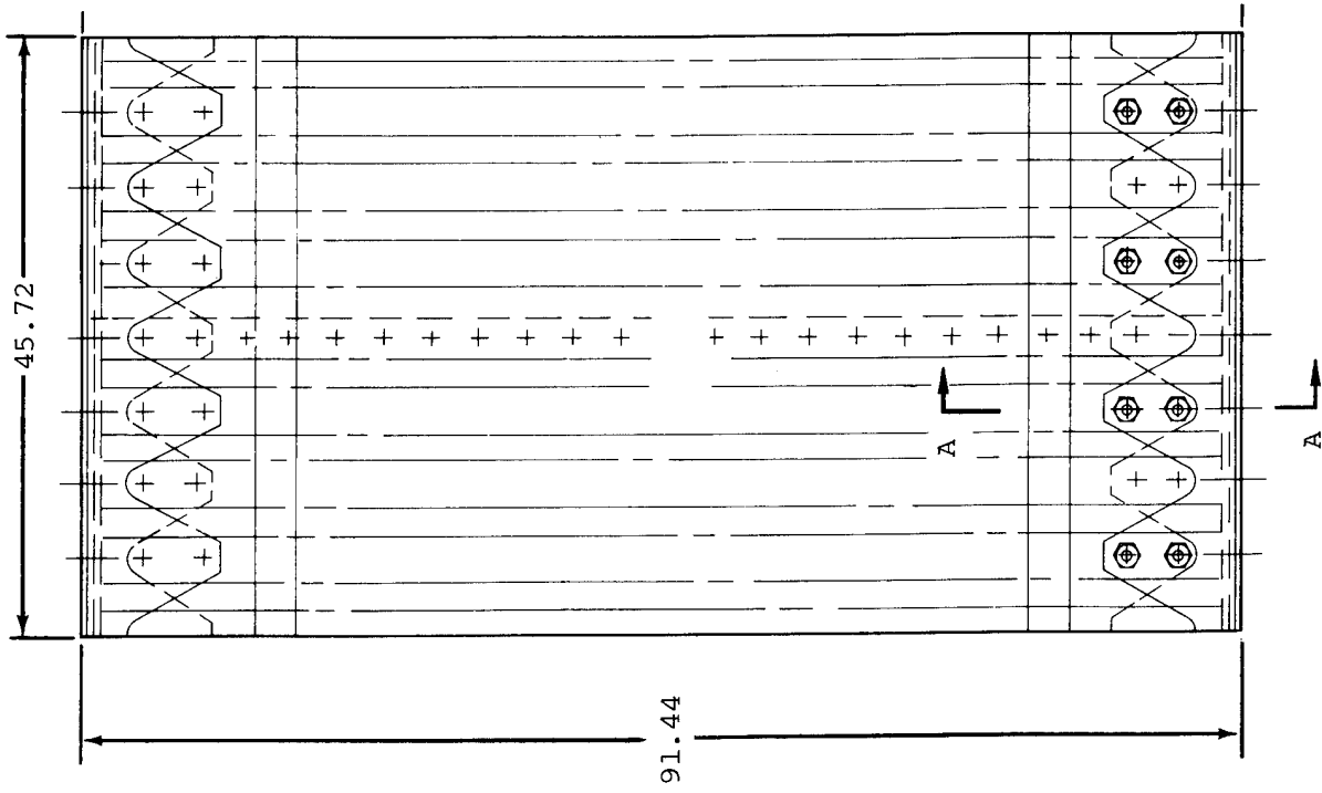
Figure 3.- Geometric details of 91.44-cm-long panels with longitudinal-joint and load-introduction fixtures. Dimensions are in centimeters.
