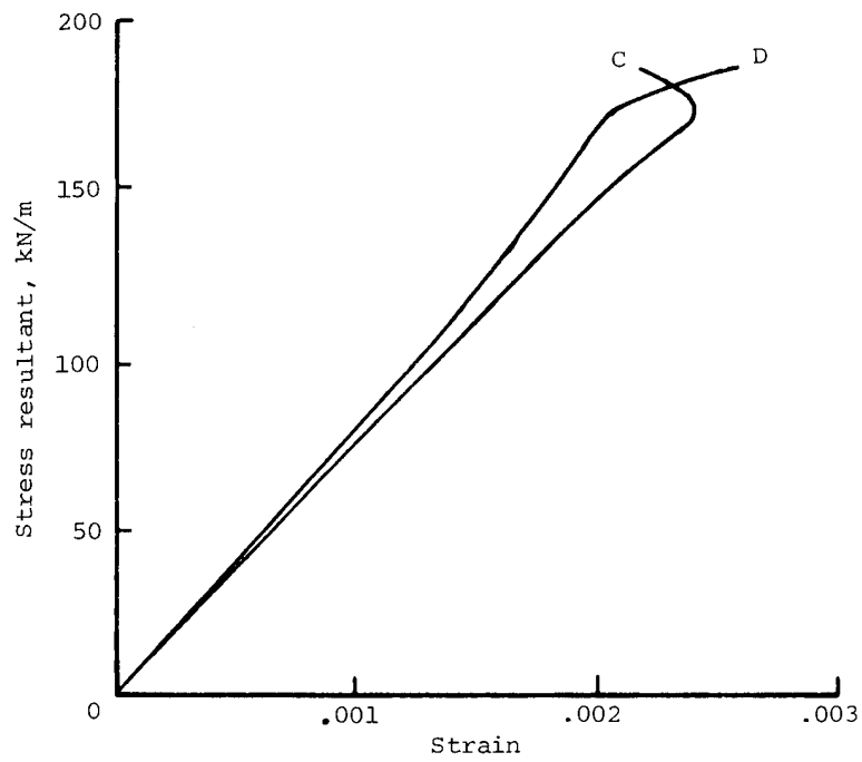
Figure 13.- Back-to-back strain-gage responses of adjacent corrugation crowns for panel 1-36.
