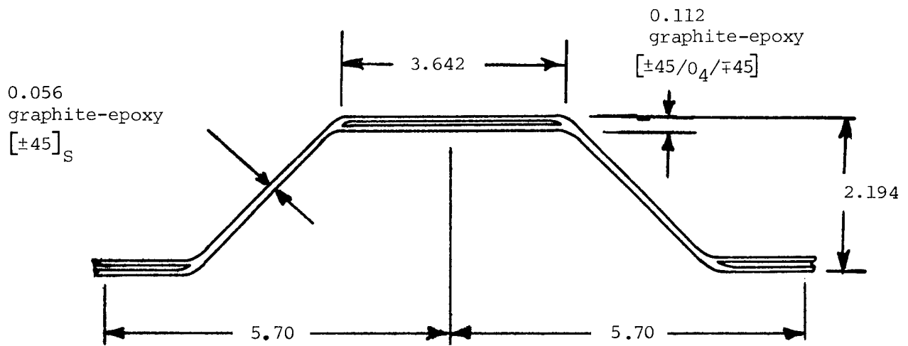
(a) Crown configuration with four 0° plies (panels 1-24 and 2-24).
