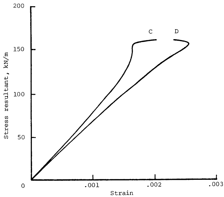
Figure 10.- Back-to-back strain-gage responses of adjacent corrugation crowns for panel 4-24.
