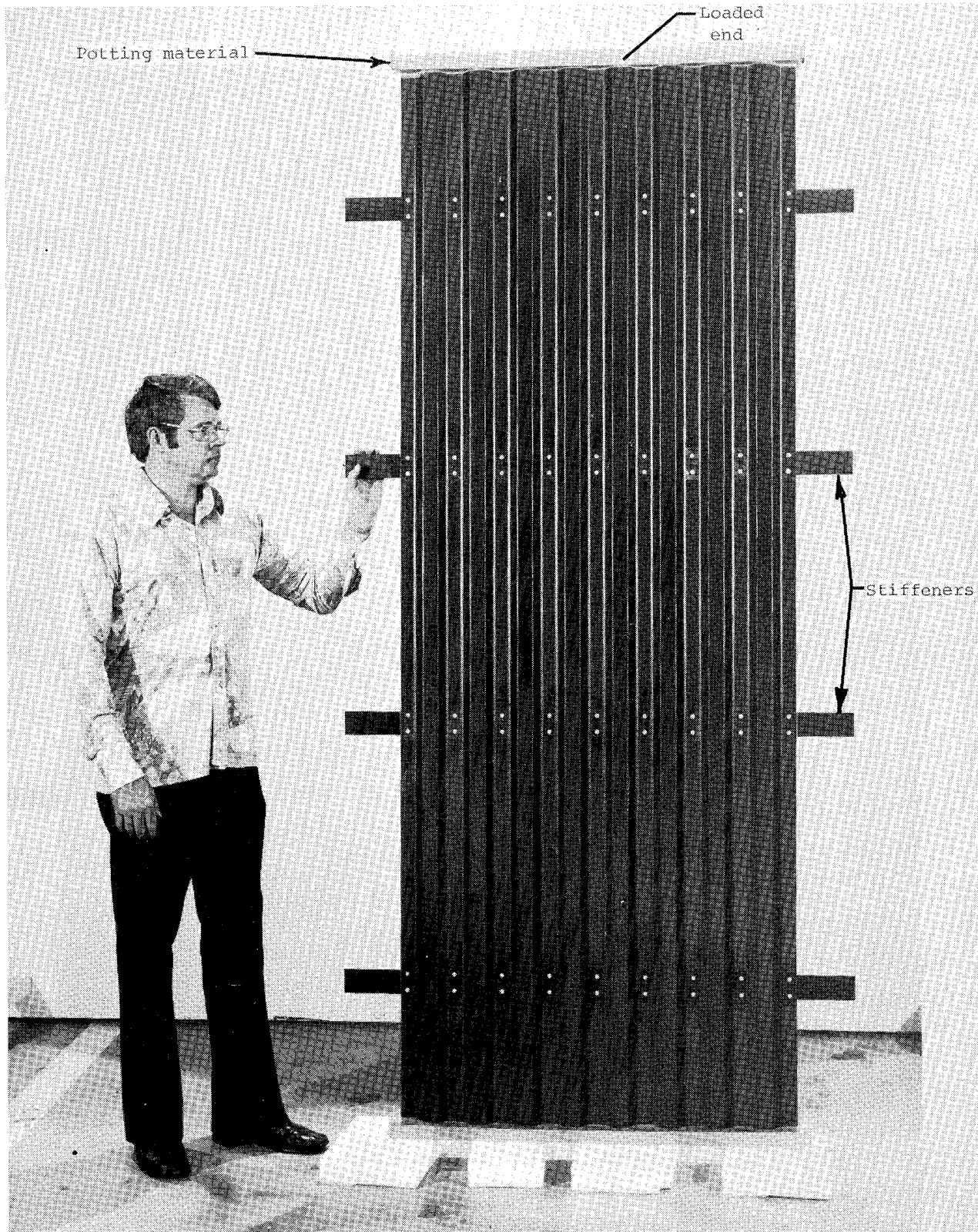
Figure 6.- Typical 254.0-cm-long graphite-epoxy corrugated panel with stiffeners.
