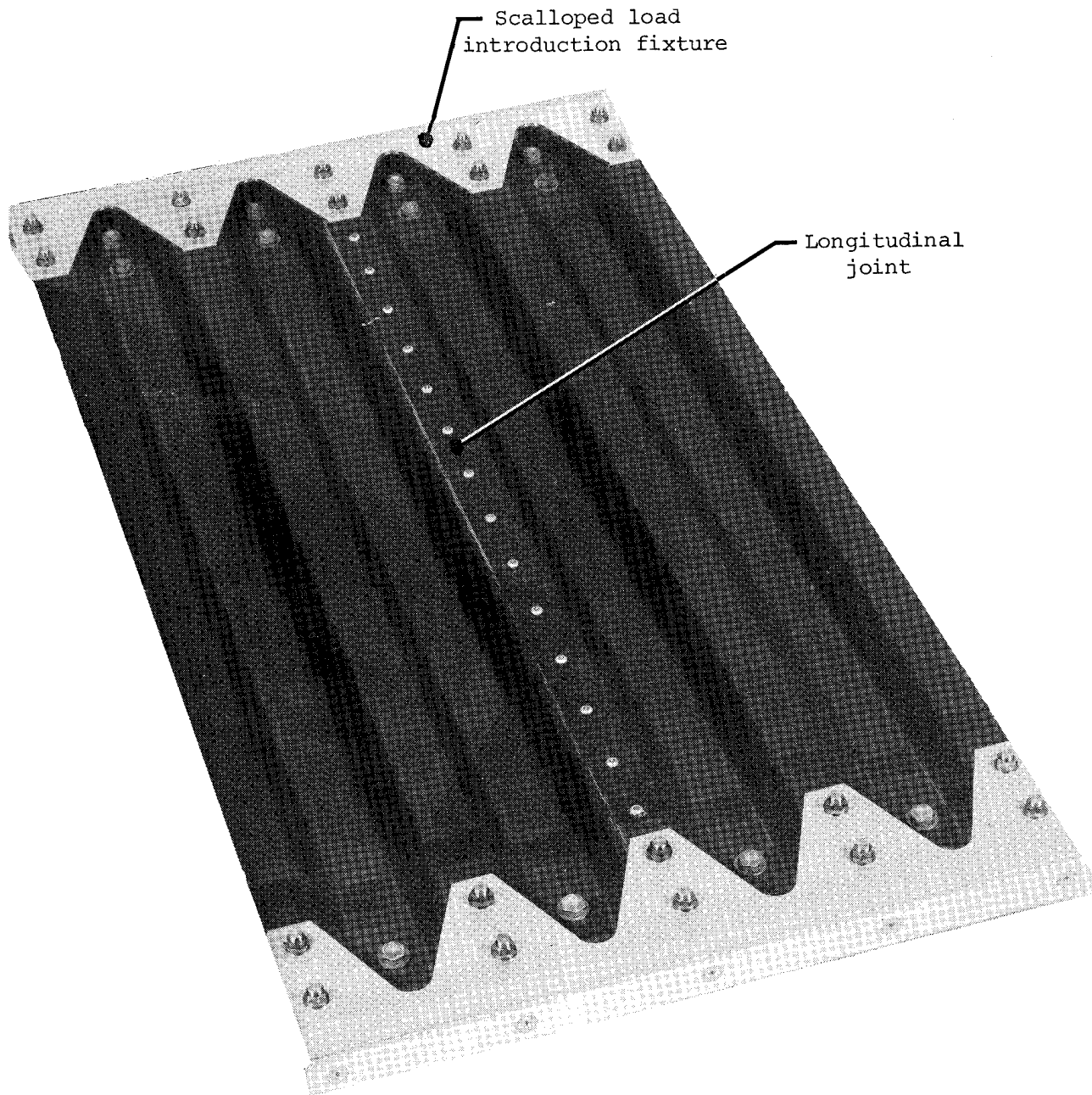
Figure 4.- Typical 91.44-cm-long test panel with longitudinal-joint and load-introduction fixtures.
