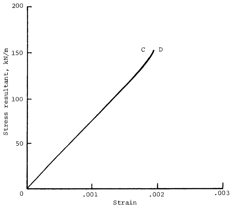
Figure 15.- Back-to-back strain-gage responses of adjacent corrugation crowns for panel 1-100.
