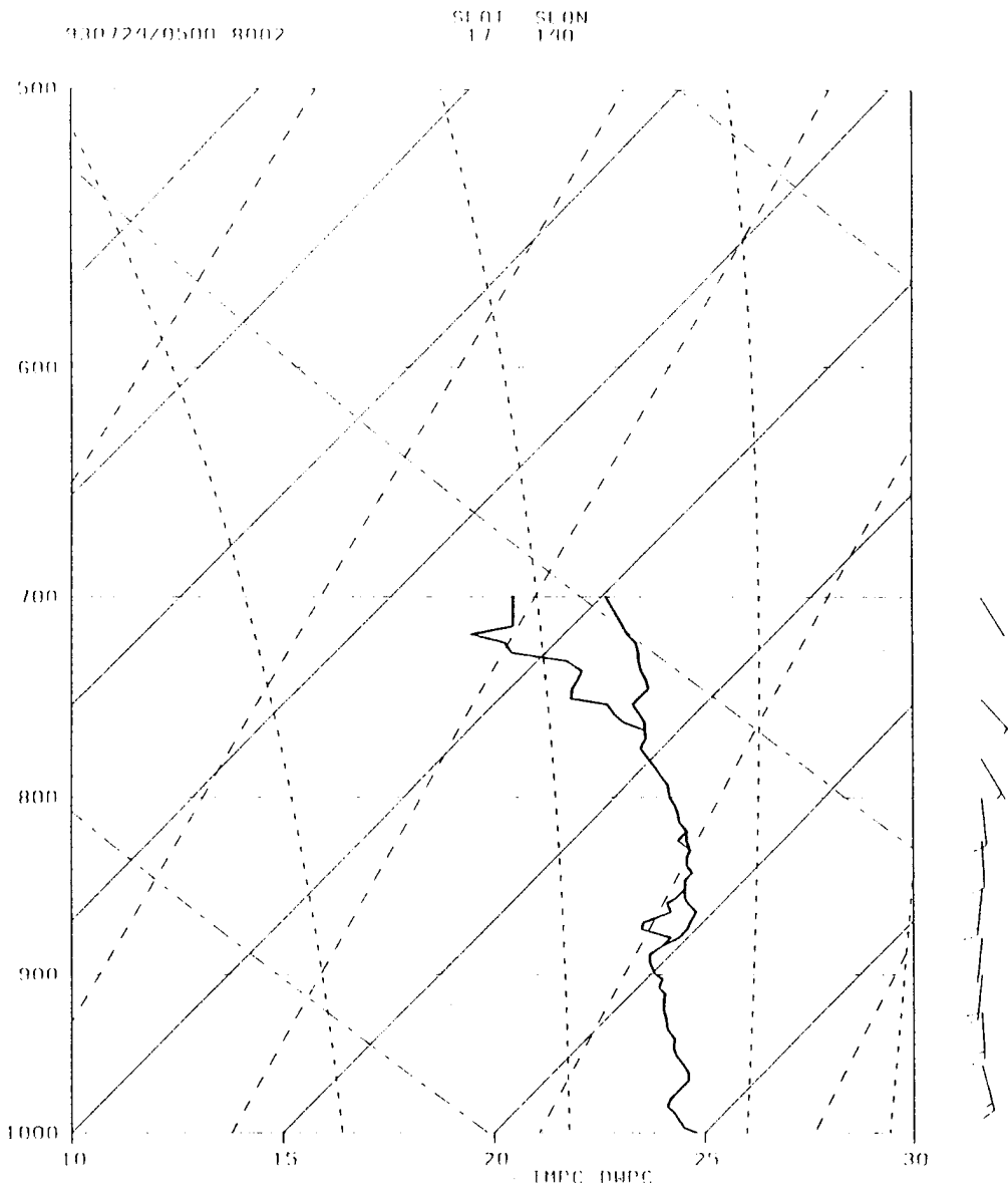
Figure 24b. ODW 2 sounding as in Fig. 15a, except deployed at 0502 UTC 24 July 1993 during AOP-1B. The complete flight track with all ODW locations is given in Fig. 2.
