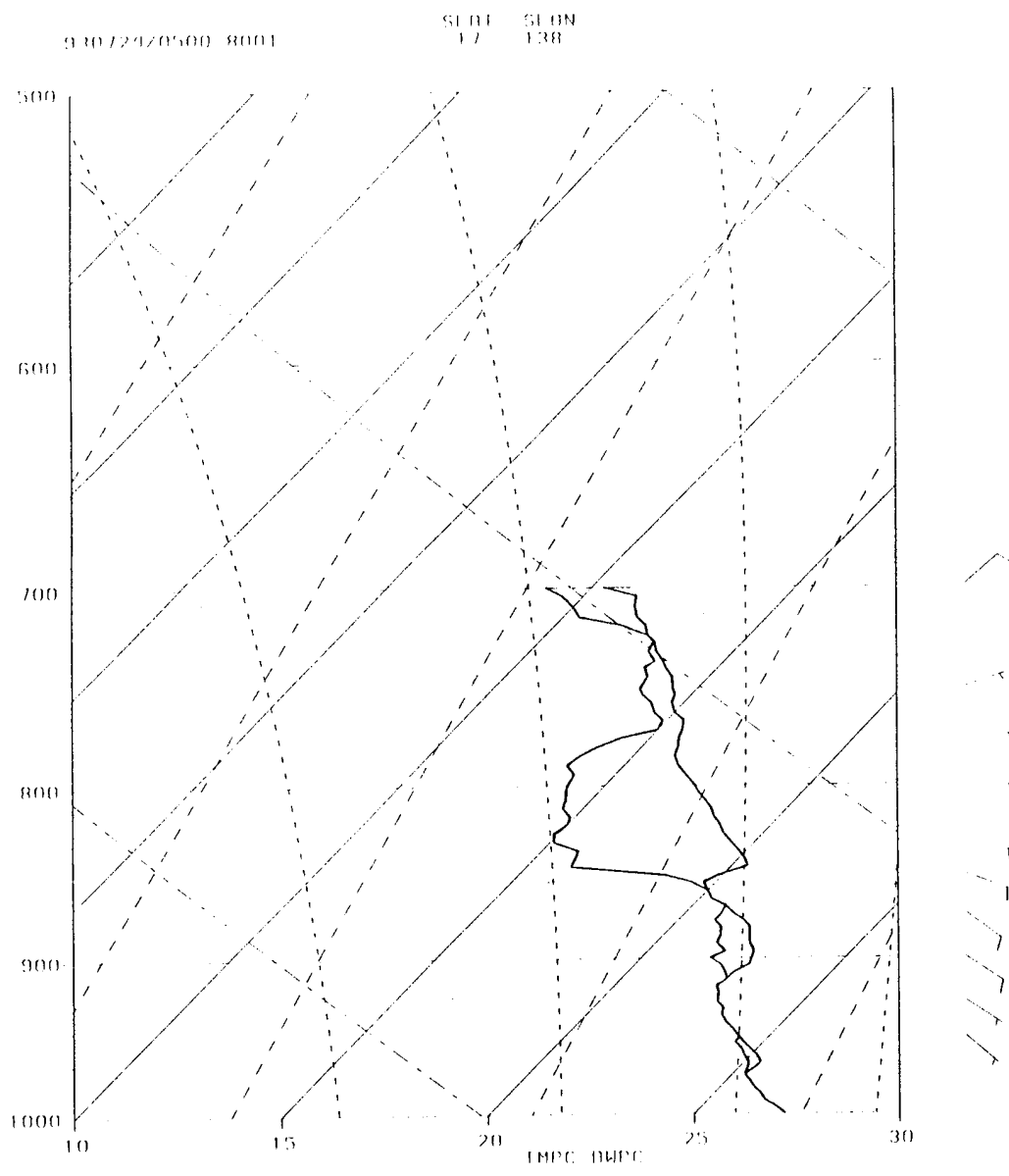
Figure 24a. ODW 1 sounding as in Fig. 15a, except deployed at 0442 UTC 24 July 1993.
