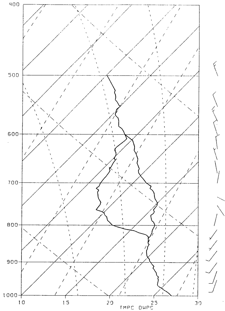
Figure 15b. ODW sounding as in Fig. 15a, except at location 4 deployed at 0409 UTC 23 July 1993.
