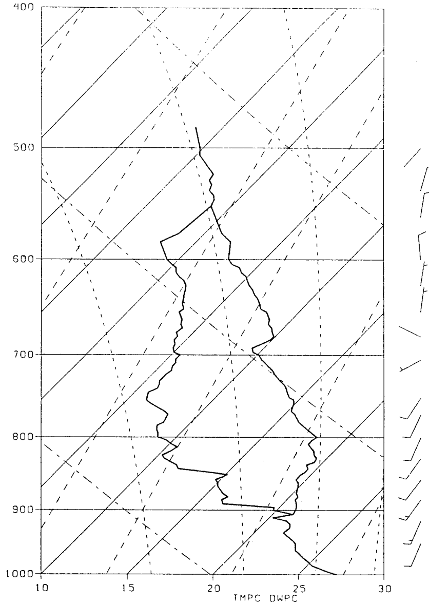
Figure 15a. ODW sounding at location 3 (see Table 1 and Fig. 1) deployed at 0354 UTC 23 July 1993. Temperatures and dew point temperatures are displayed on a skew-T-ln p diagram and wind barbs ( \text{m s}^{-1} ) are shown on the right.
