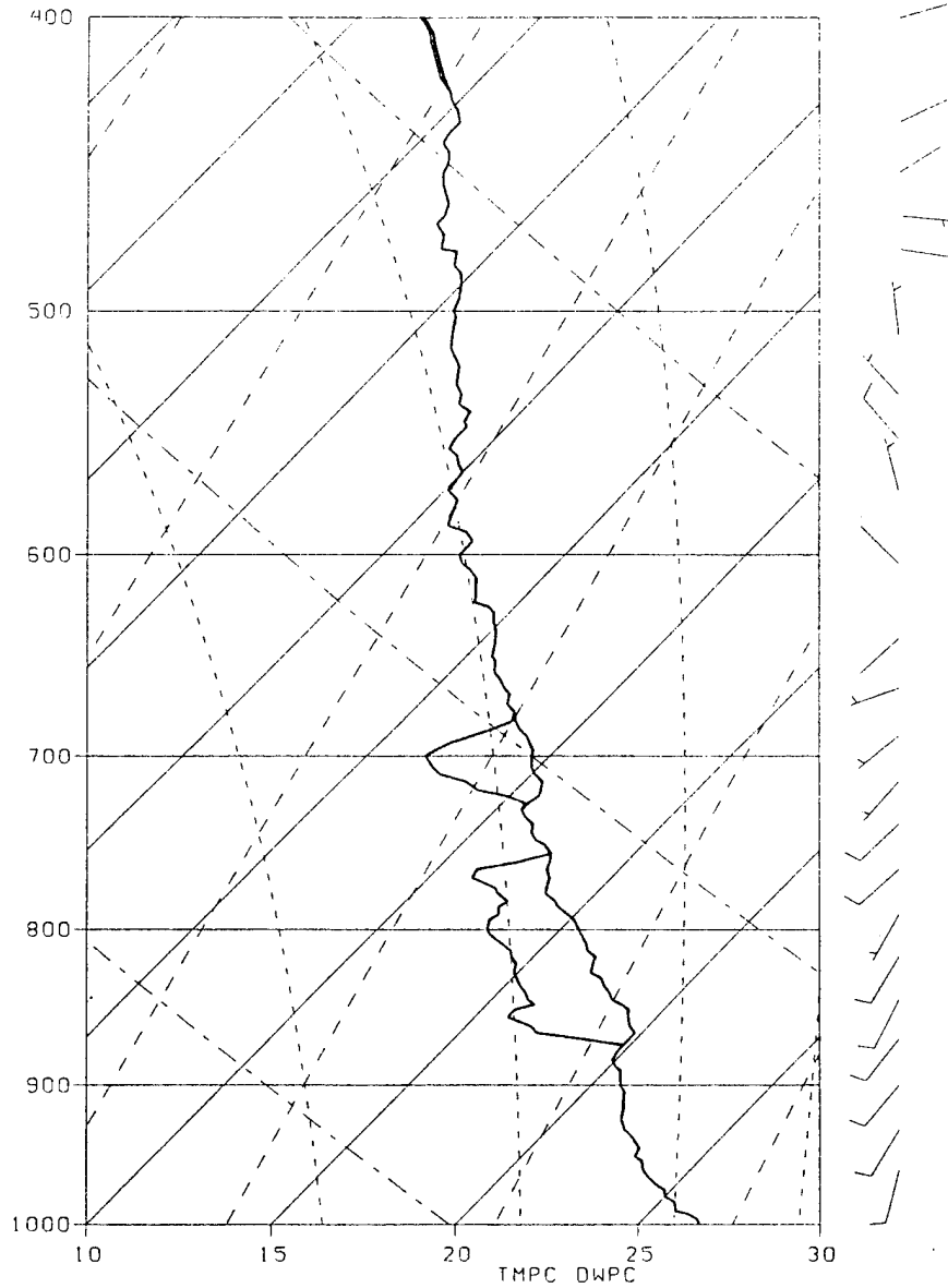
Figure 16b. ODW 16 sounding as in Fig. 15a, except deployed at 0818 UTC 23 July 1993.
