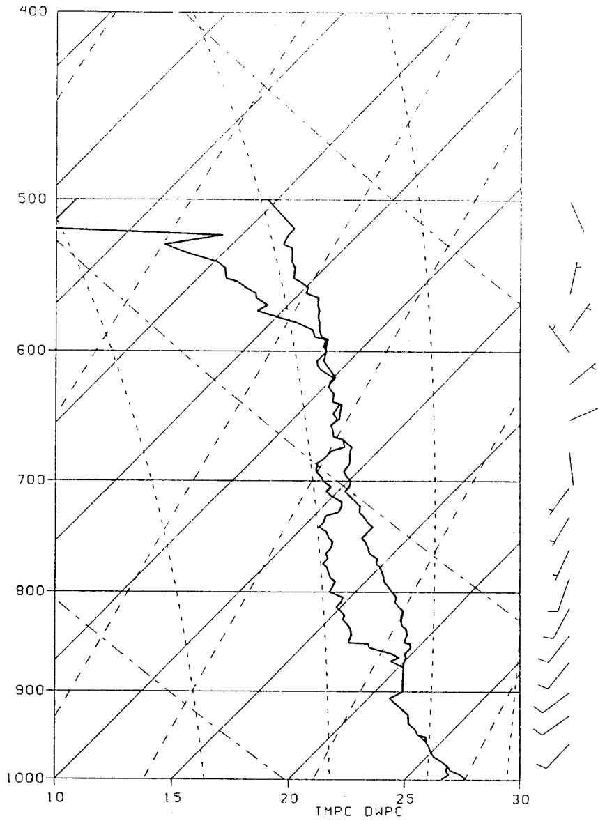
Figure 16a. ODW 8 sounding as in Fig. 15a, except deployed at 0522 UTC 23 July 1993.
