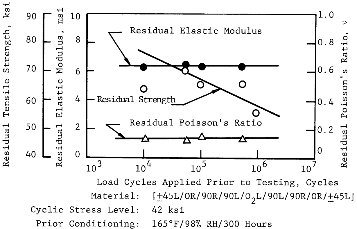
FIGURE 15 Residual Strength, Elastic Modulus and Poisson's Ratio for Composite Material ( \phi=1800 cpm, R=0.1 T=75°F, Orientation, Stress Level and Prior Conditioning as Noted), 33% Graphite by Plies.
