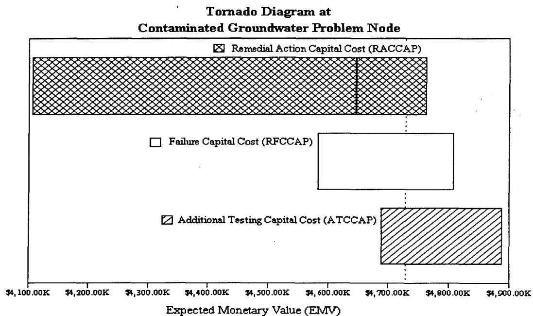
Figure 46. Tornado diagram illustrating sensitivity for the capital cost variables of the objective function.
