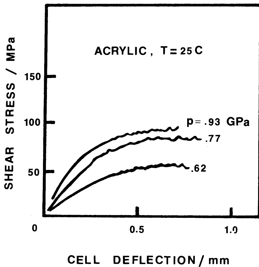
Figure 10. Shear Stress-Cell Deflection for Acrylic Plastic at Three Pressures and 25C
