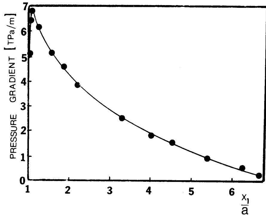
Figure 30. Pressure gradient distribution at the inlet zone for the conditions of point C of Figure 21
