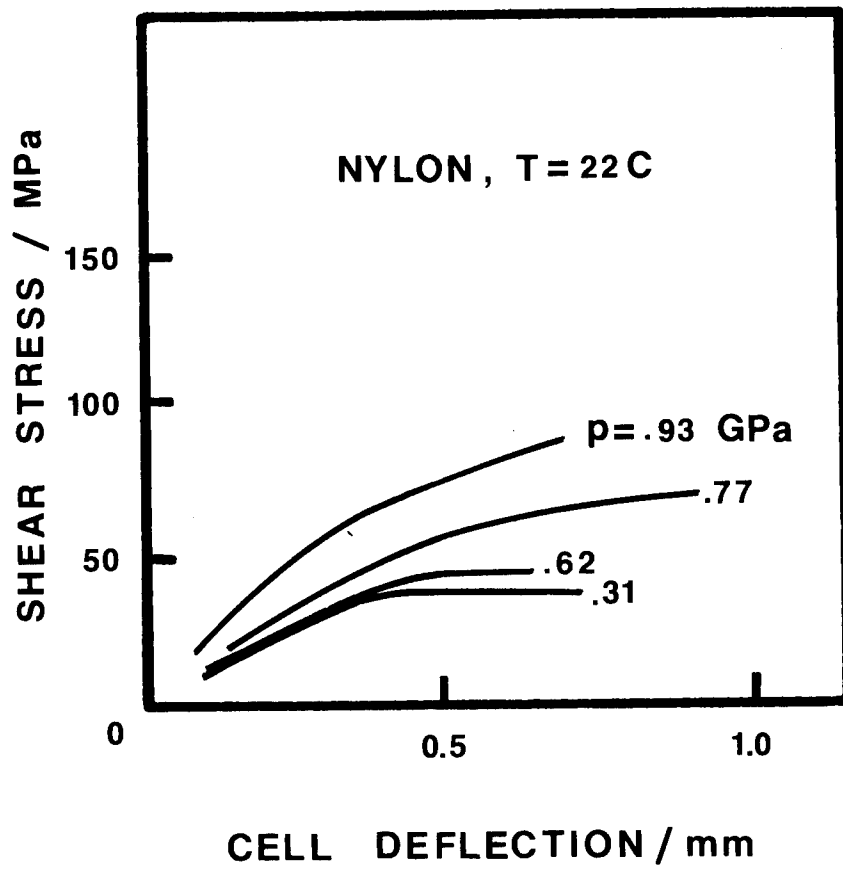
Figure 11. Shear Stress-Cell Deflection for Nylon at Four Pressures and 22C
