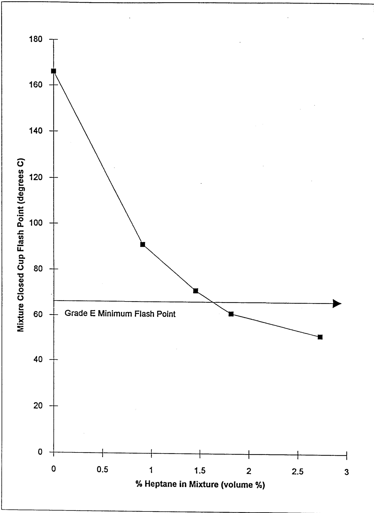
Figure 5-5. Effect of Heptane Contamination on Lubricating Oil
