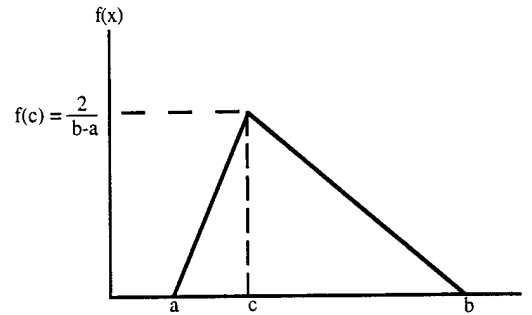
Figure 4.1 Triangular Probability Distribution
