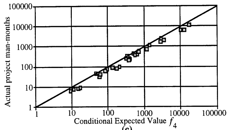
Figure 5.7 Intermediate COCOMO model results: (a) Original forecast versus actuals, (b) Unconditional expected values versus actuals, (c) Conditional expected values versus actuals.
