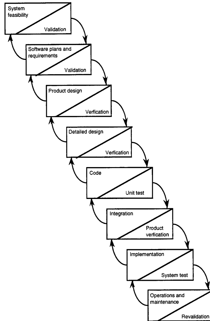
Figure 1.2 Waterfall model of the software process [Boehm 1981]
