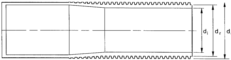
Figure 19. Horizontal integral-fin tube.
