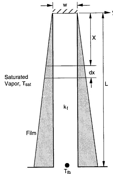
Figure 6. Condensation on a vertical fin of rectangular profile.
