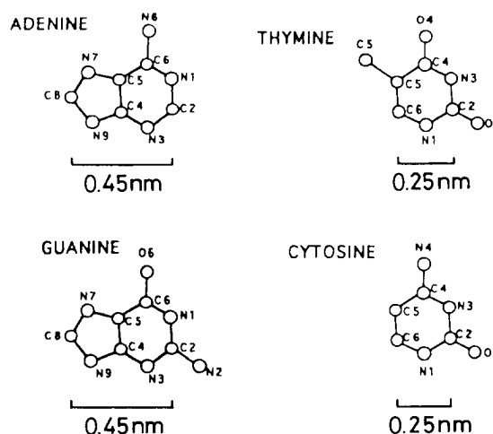
Fig. 1. Molecular structures of adenine, thymine, guanine and cytosine with atomic labelling convention and with scales.
