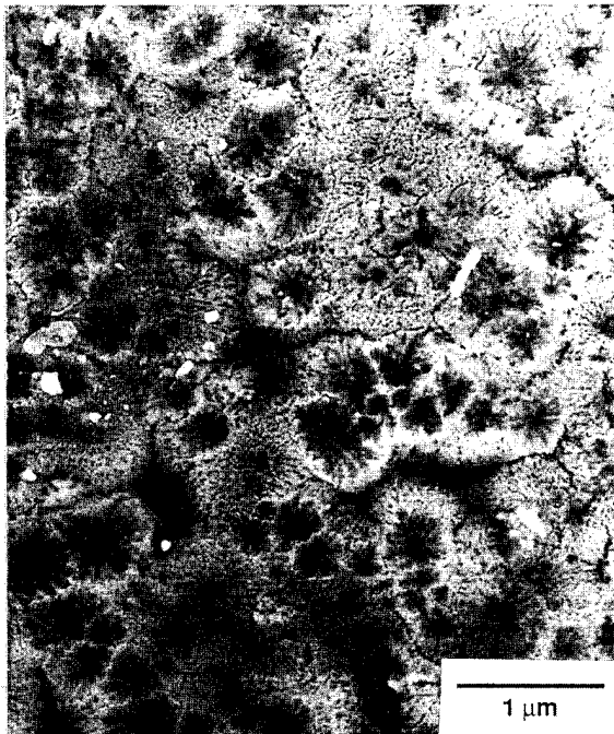
Fig. 9. Backscattered SEM micrograph of the top surface of the CAP glass-ceramic layer.
