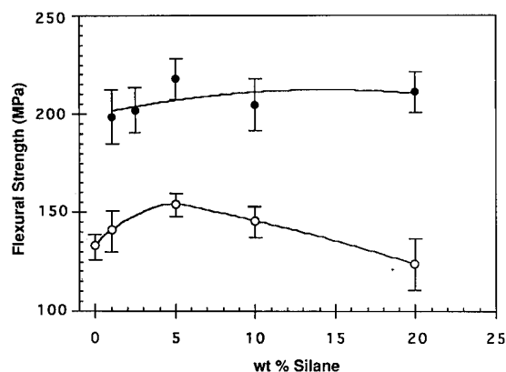
Fig. 7. Dependence of strength of alumina-epoxy composites on silane treatment: (○) silane added to the resin before infiltration and (●) alumina pretreated with a silane solution before infiltration with resin.
