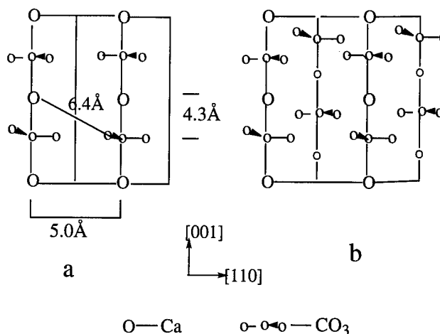
Fig. 11. Cell projections for calcite. (a) Parallel to the (110) axis with only coplanar atoms in the (110) face; (b) parallel to the (110) axis with additional non-coplanar atoms [5].
