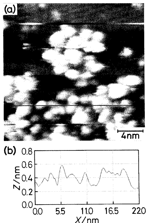
Fig. 8. (a) Constant current STM image ( 22 \text{ nm} \times 21 \text{ nm} \times 0.8 \text{ nm} ( x, y, z )) of guanidine on a reduced \text{SrTiO}_3(100) clean surface, taken at a sample bias of -3 \text{ V} and tunnelling current of 0.2 \text{ nA} . (b) A cross-section of (a). In this cross-section, guanidine adsorbates have a typical height of 0.24 \pm 0.05 \text{ nm} at a sample bias voltage of -3 \text{ V} .
