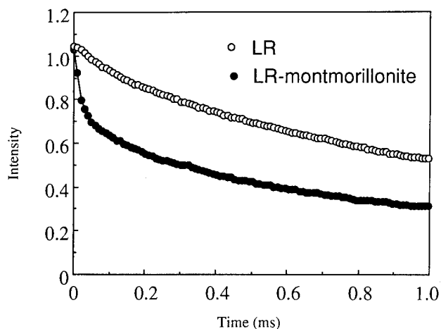
Fig. 9. T_2 signal for LR–montmorillonite.
