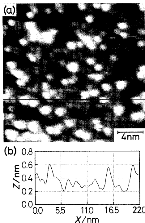
Fig. 9. (a) Constant current STM image ( 22 \text{ nm} \times 21 \text{ nm}^2 ) taken after the deposition of thymine on adenine. (b) Cross-section of (a). The image was acquired at a sample bias of -3 \text{ V} (tunnelling current of 20 \text{ pA} ) to differentiate between the adsorbed species.
