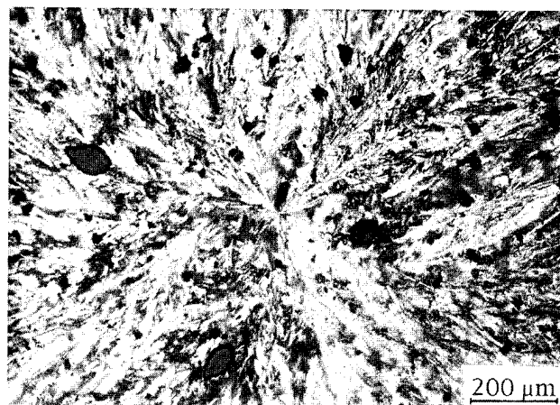
Fig. 1. A transmission optical micrograph of crystals grown from gallstone melt on a microscope slide. The recrystallization temperature was 84 °C. The resulting microstructure consists of radiating arrays of cholesterol crystals emerging from a unique nucleation center exhibiting spherulitic crystallization.
