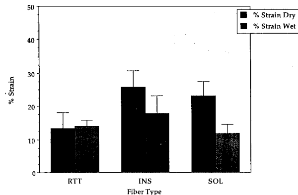
Fig. 3. Percent strain at failure of different dry native (RTT) fiber, insoluble (INS) fiber and soluble (SOL) fiber pulled to failure in uniaxial tension.
