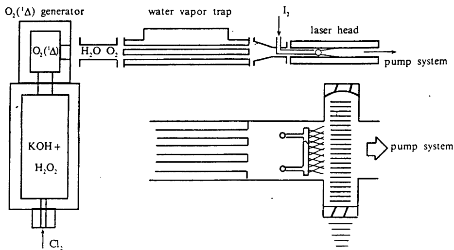
Fig.1 Schematic of CW chemical oxygen-iodine laser
