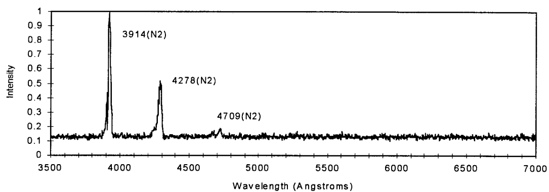
Figure 11a: Spectrum of a 4.5E-7 A, 0.5 MeV H 3 + excited air (P=1.2E-4 torr) observed 3 mm downstream from the foil wheel w/o the gel (Area A).
