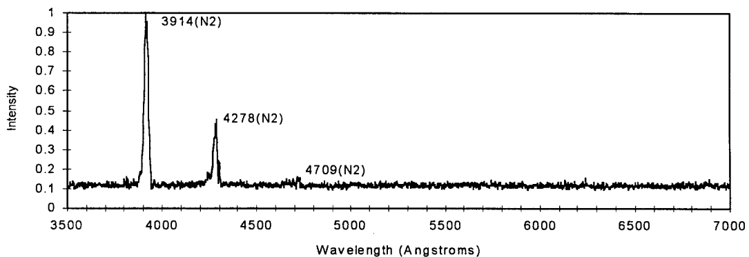
Figure 11c: Spectrum of a 4.5E-7 A, 0.5 MeV H 3 + excited air (P=1.2E-4 torr) observed 10 mm downstream from the foil wheel w/o the gel (Area C).
