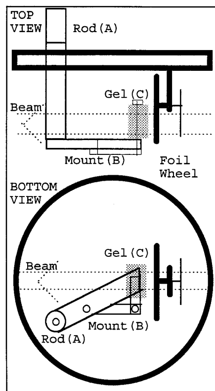
Figure 5: Target Chamber
