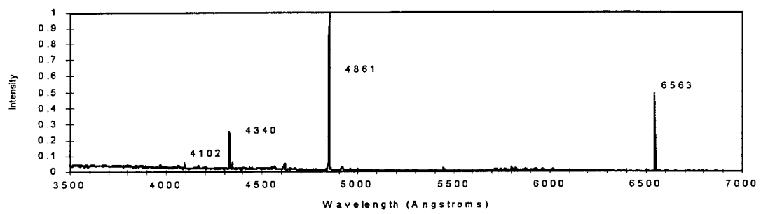
Figure 8a: Spectrum of a hydrogen Geissler tube at 55 VDC.
