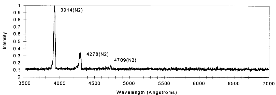
Figure 11b: Spectrum of a 4.5E-7 A, 0.5 MeV H 3 + excited air (P=1.2E-4 torr) observed 5 mm downstream from the foil wheel w/o the gel (Area B).
