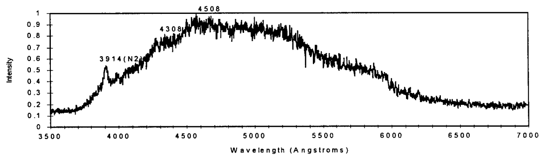
Figure 8d: Spectrum of a 5E-7 A, 0.5 MeV H3^+ excited gel ( P=1.2E-4 torr) observed 1 mm inside the gel (Area B).
