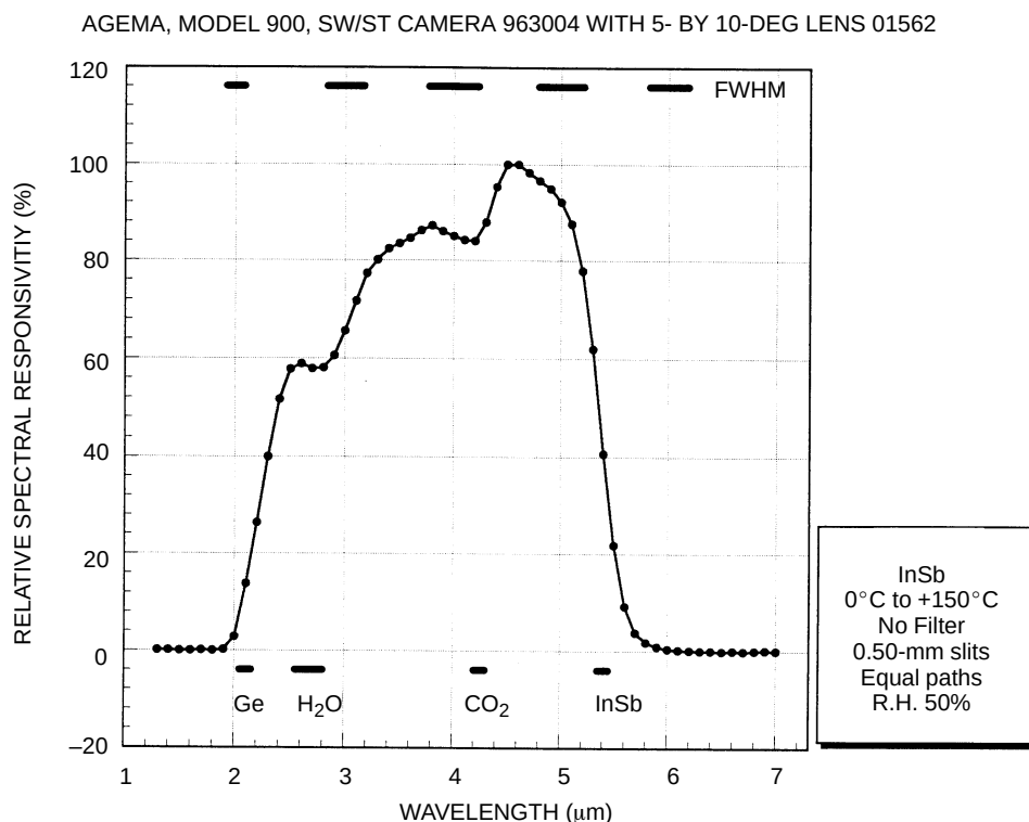
Figure 6. Responsivity of the AGEMA, Model 900, SW/ST camera system. The horizontal bars labeled “FWHM” show the full width at half maximum of the triangular monochromator bandpass for the 0.5-mm entrance and exit slits used in this measurement. The major spectral features of this curve are determined by those materials shown at the bottom of the figure.
