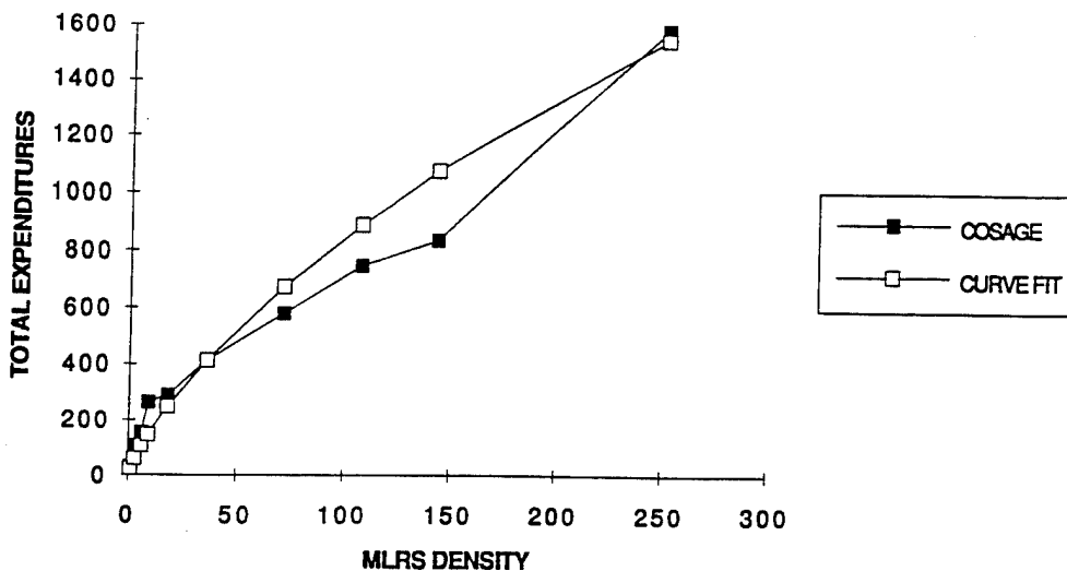
Figure 2-5. MLRS Rounds Expended in COSAGE and ATCAL Curve Fit Process
