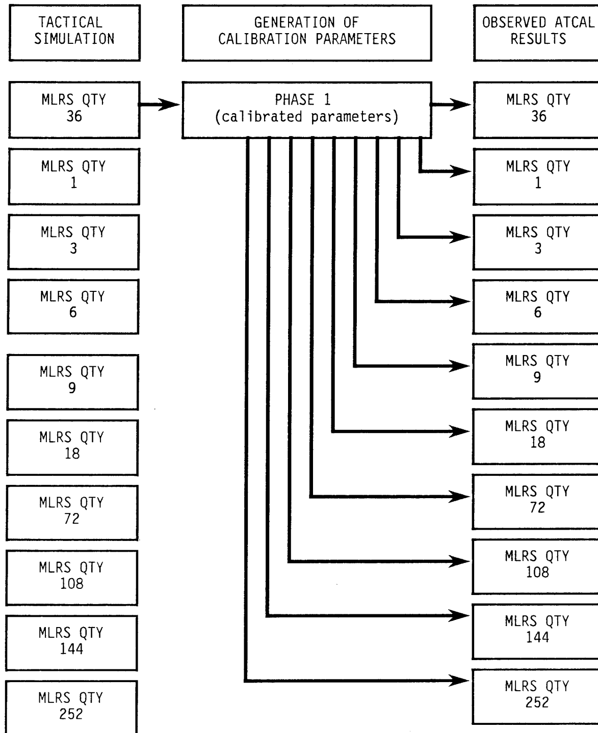
Figure 2-1. Experiment 2 Schematic
