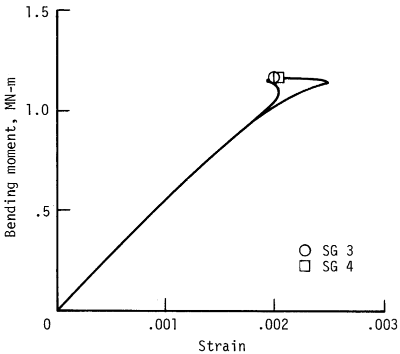
Figure 11.- Strain-gage (SG) responses in section between rings 1 and 2.
