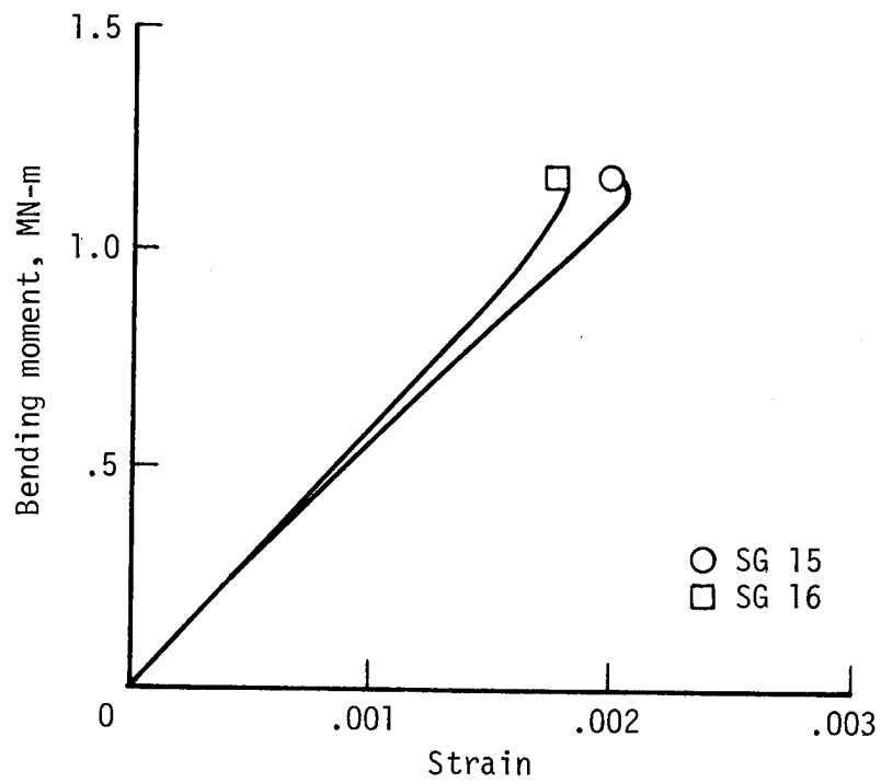
Figure 12.- Strain-gage (SG) responses in section between rings 2 and 3.
