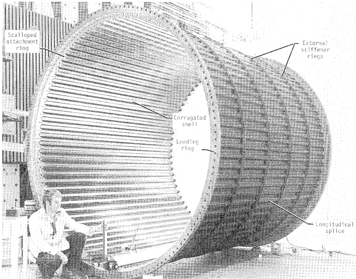
Figure 3.- Photograph of 3-m-diameter corrugated graphite-epoxy cylinder.
