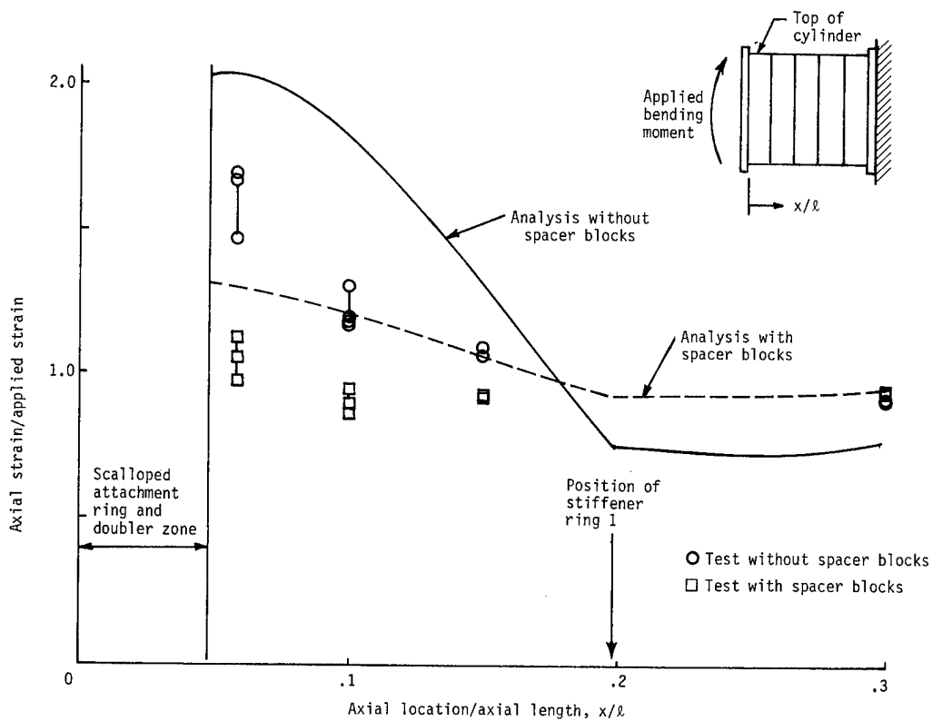
Figure 7.- Axial strain at top of cylinder from analysis and test at 30 percent of design load.
