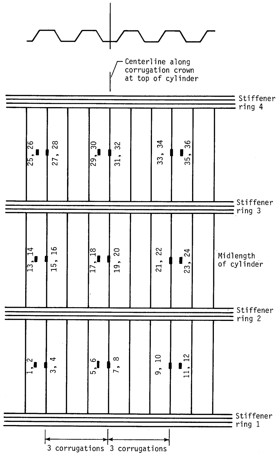
Figure 10.- Strain-gage locations on top of cylinder.
