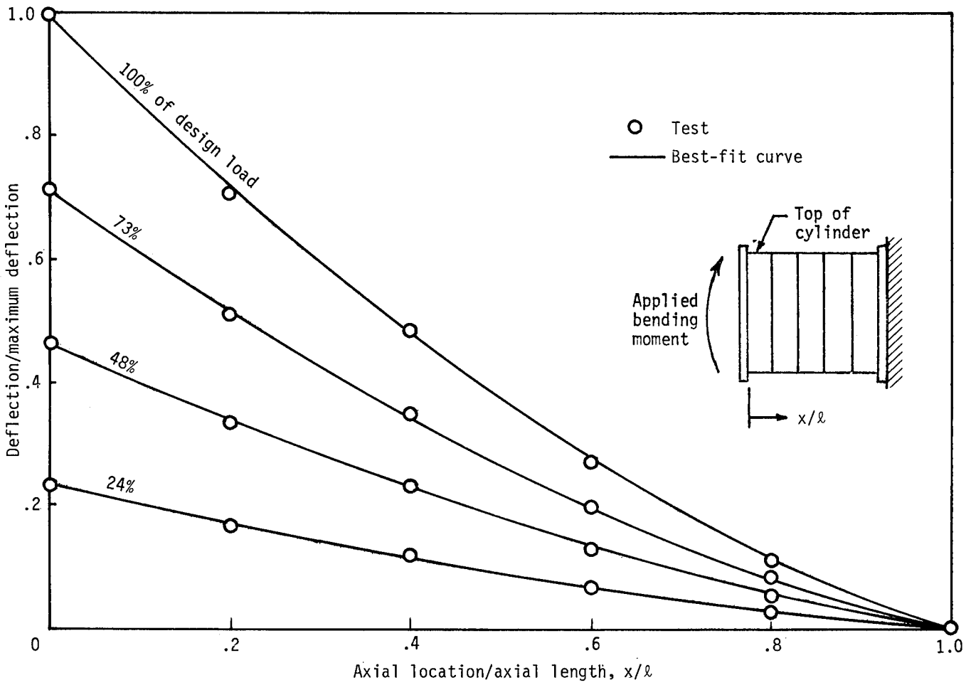
Figure 9.- Deflection of cylinder under bending moment.
