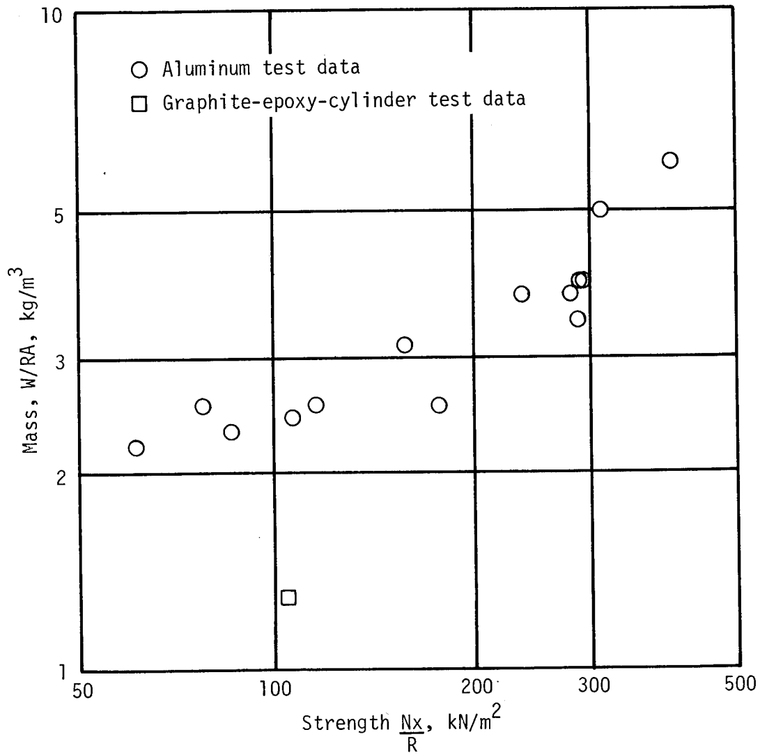
Figure 15.- Mass-strength plot showing mass-saving potential of graphite-epoxy cylinder.
