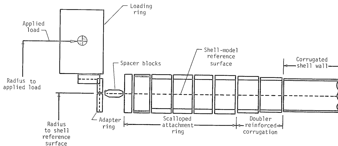
Figure 5.- Schematic of model used in shell analysis.
