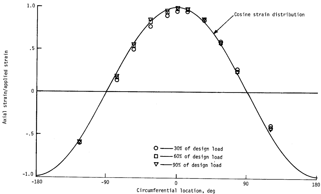
Figure 8.- Axial strain around circumference at midlength of cylinder with spacer blocks in place.
