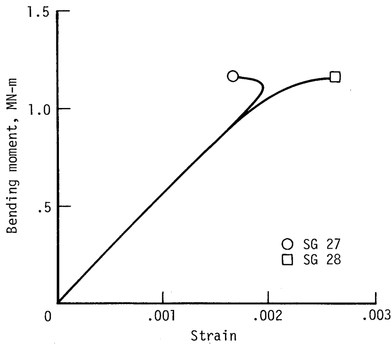
Figure 13.- Strain-gage (SG) responses in section between rings 3 and 4.
