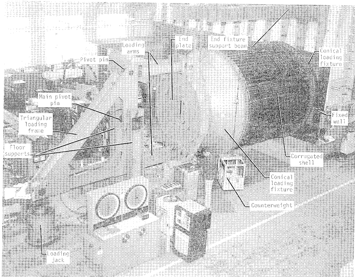
Figure 4.- Test fixture for applying bending moment to corrugated cylinder.
