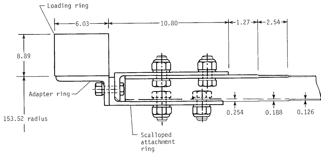
Figure 2.- Loading-ring and scalloped-attachment-ring details at end of cylinder. Dimensions are in centimeters.
