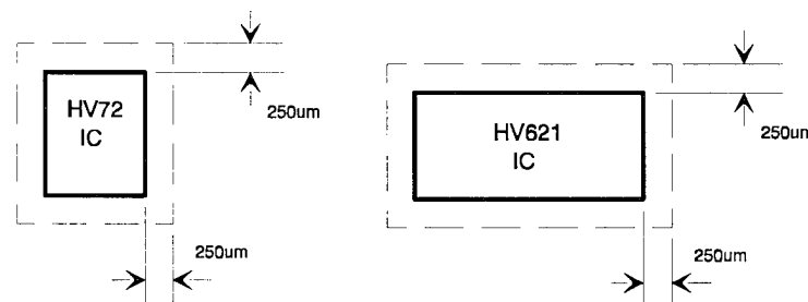
Figure 10. Clear Area Around IC's.
