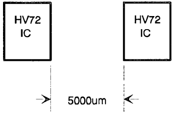
Mimimum Spacing with wire bonds
