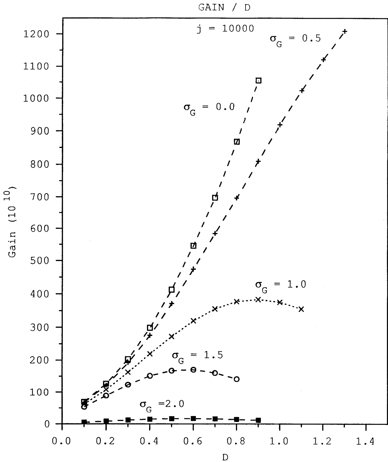
Figure 3-10a. Gain vs. D plots for dimensionless current j = 10000 .
