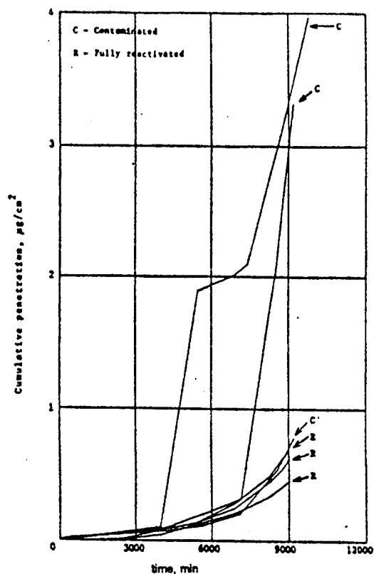
Figure 8. Cumulative HD penetration of simulated human sweat contaminated and iodine-reactivated carbon fabric.
