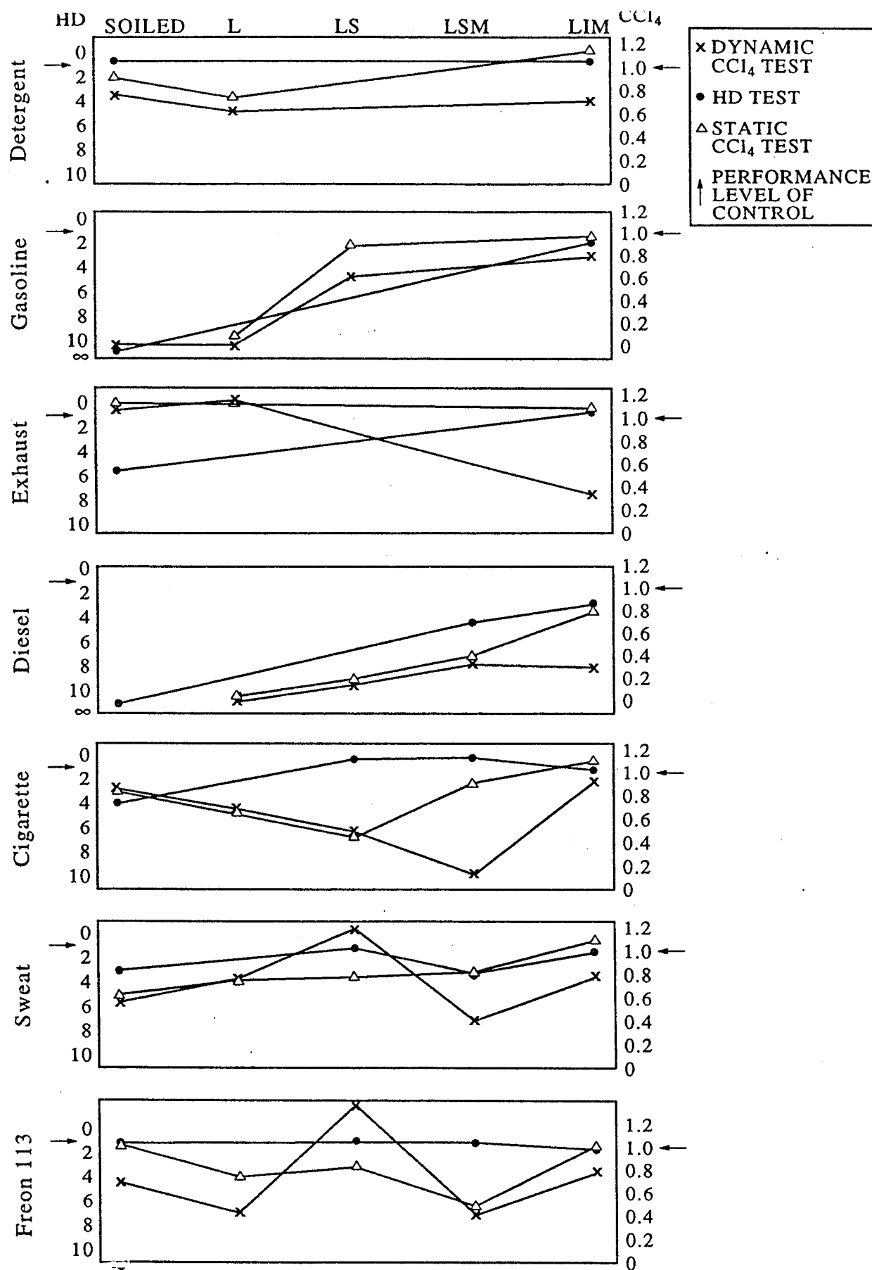
Figure 11. Summary graphs of HD and \text{CCl}_4 tests on Toyobo samples contaminated and reactivated to various extents
