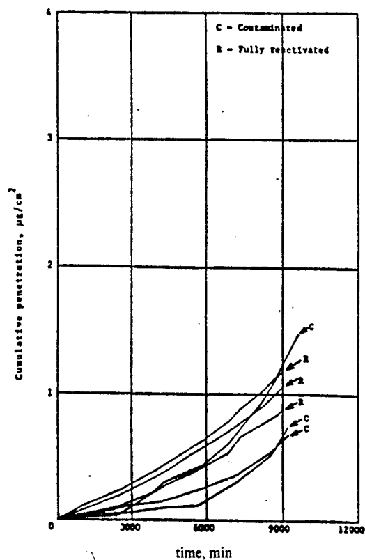
Figure 10. HD penetration Freon 113-contaminated and iodine-reactivated carbon fabric.
