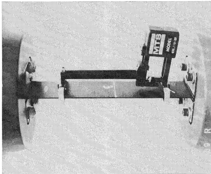
Extensometer (clip gage) with extender arm
