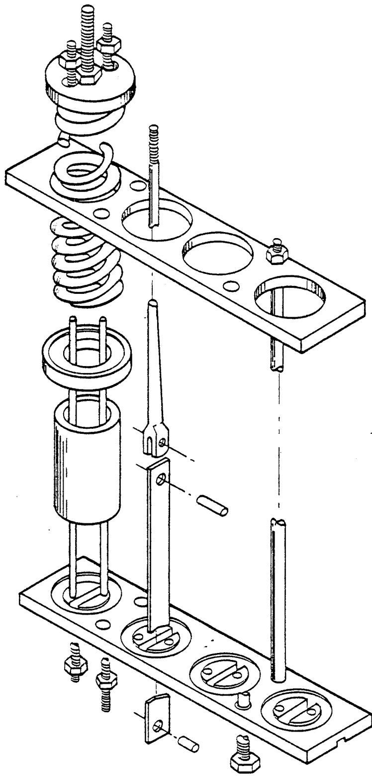
Figure 5. Sustained Stress Fixture
