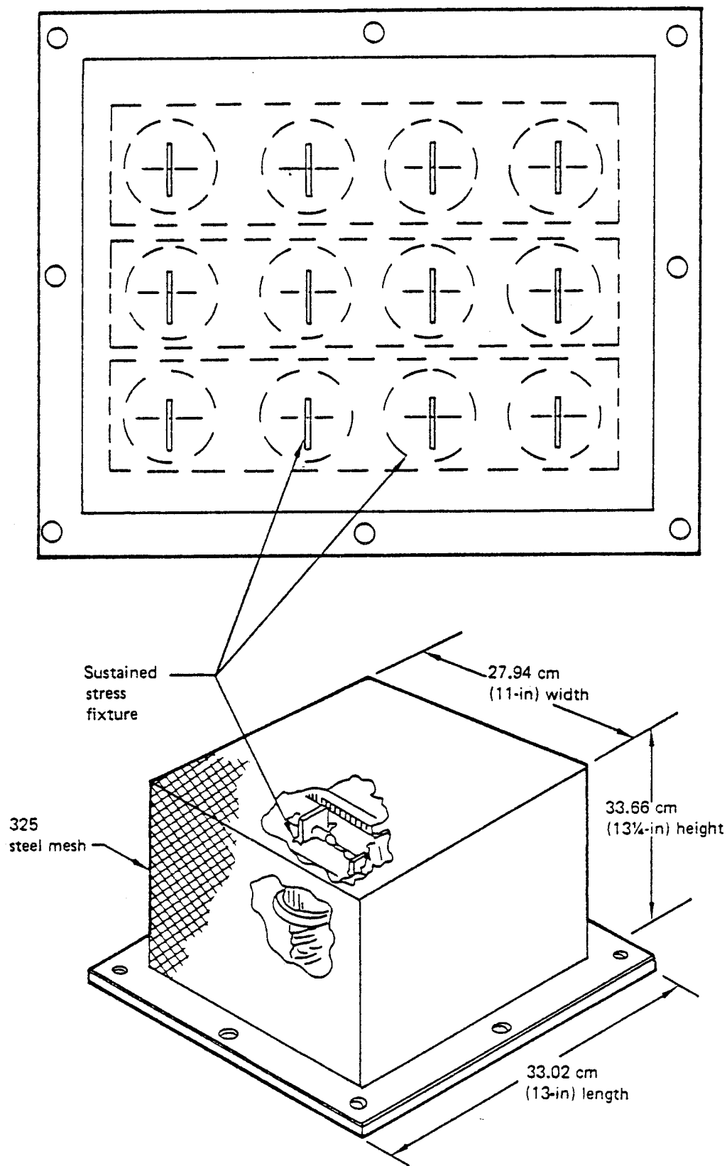
Figure 4. Fixture for Sustained Tension Loads
