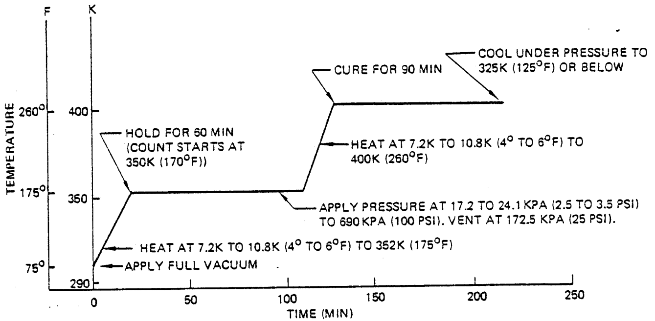
394K (250°F) Cure Cycle.
