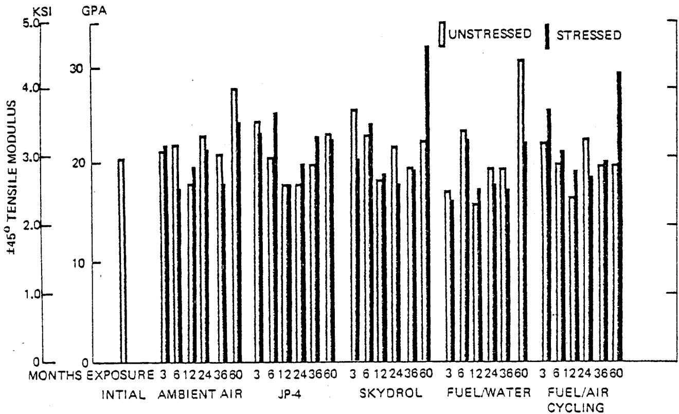
Figure 10. Environmental Exposure of T300/5209 ( \pm 45^\circ Tensile Modulus, V_F = 66.8\% )
