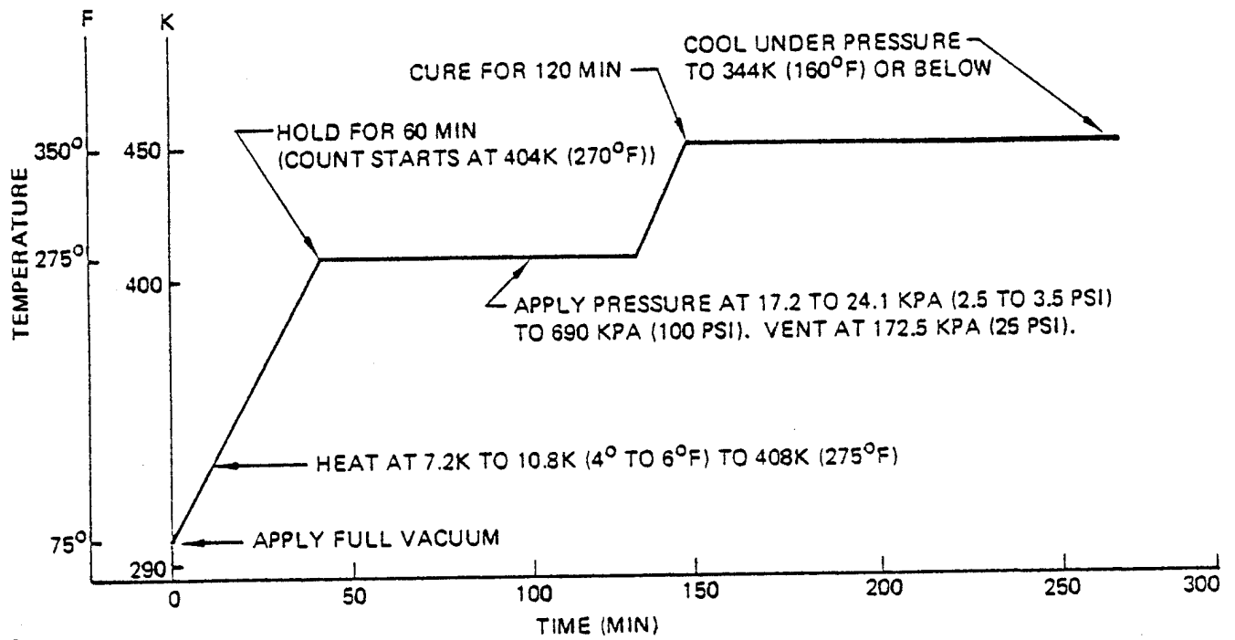
450K (350°F) Cure Cycle
