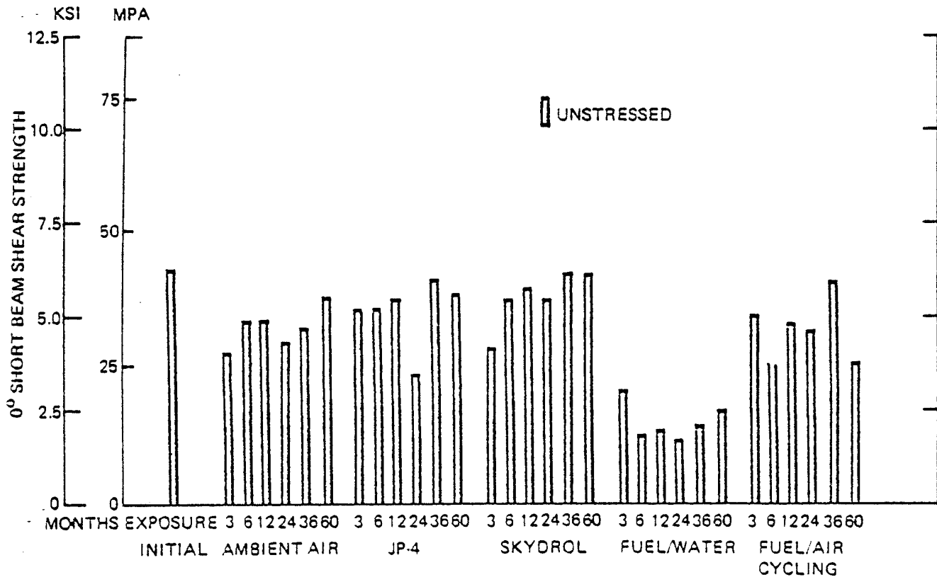
Figure 14. Environmental Exposure of Kevlar 49/2544 ( 0^\circ Short Beam Shear, V_F = 64.2\% )
