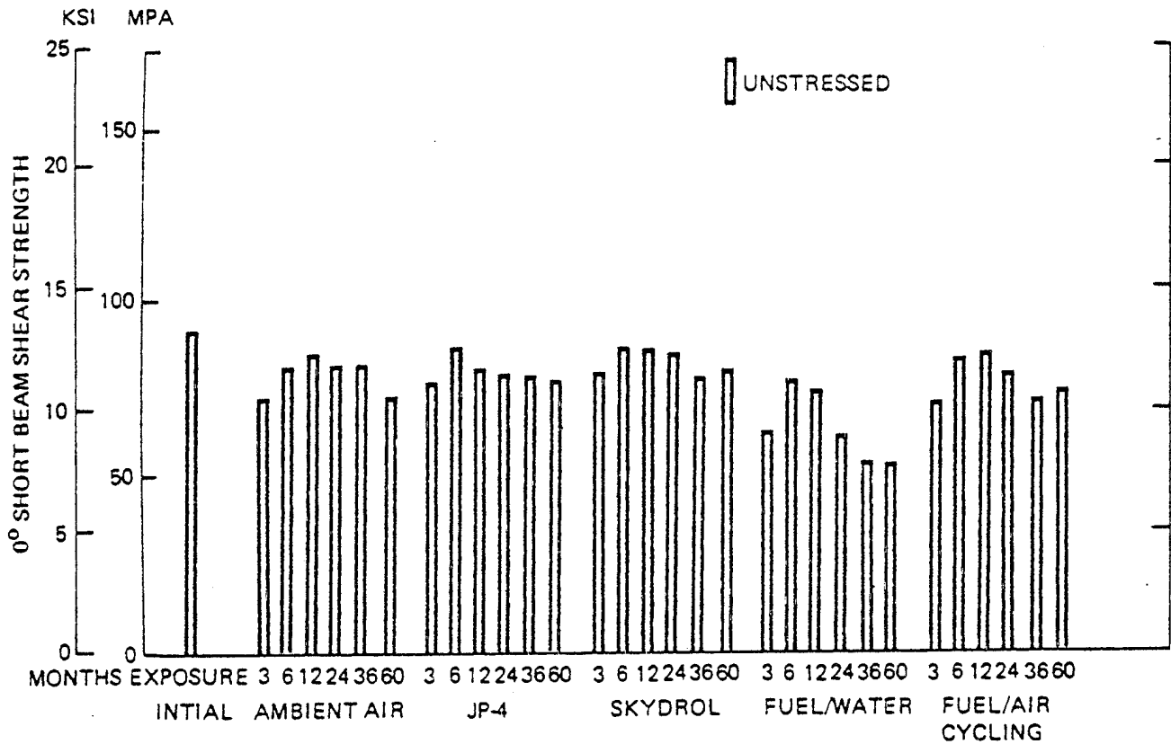
Figure 11. Environmental Exposure of T300/5209 (0° Short Beam Shear, V_F = 66.8\% )
