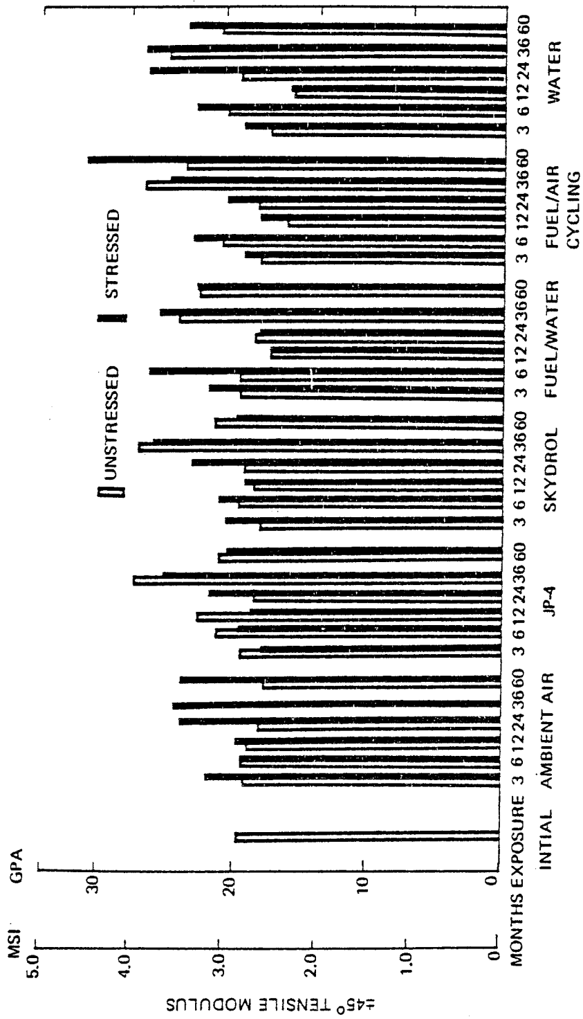
Figure 7. Environmental Exposure of T300/5208 ( \pm 45^\circ Tensile Modulus, V_F = 64.6 )
