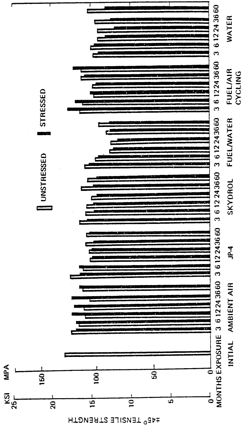
Figure 15. Environmental Exposure of Woven Kevlar (281)/5209 ( \pm 45^\circ Tensile Strength, V_F = 64.4\% )
