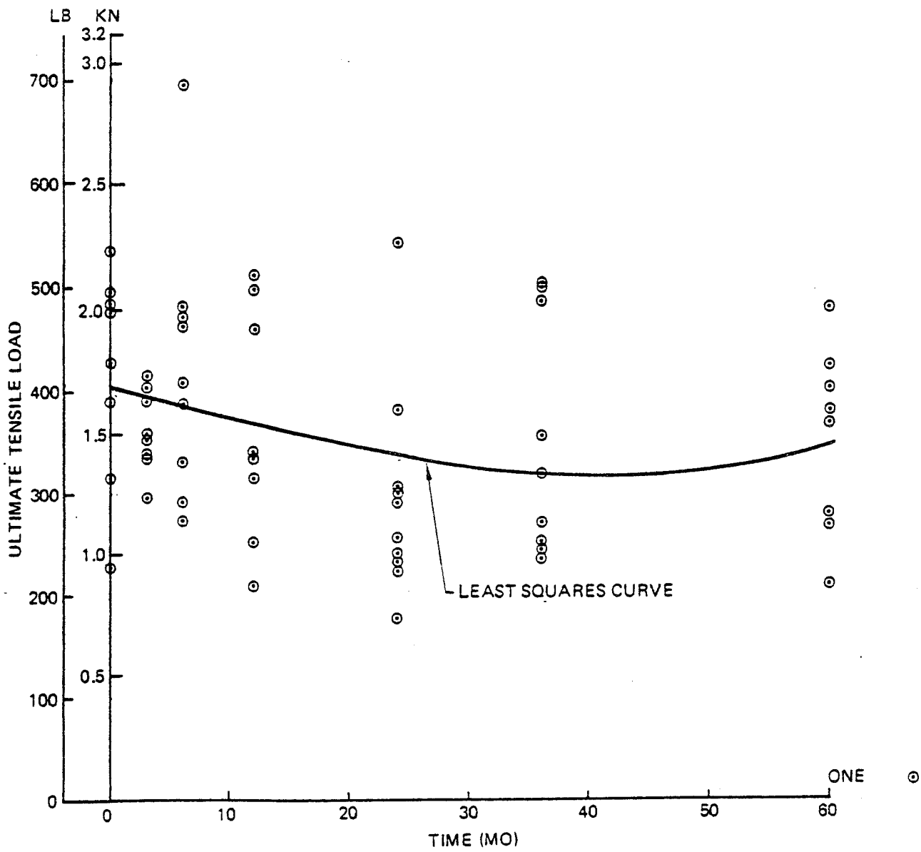
Figure 18. Tensile Results of (Unstressed) Kevlar Strands Immersed in Water
