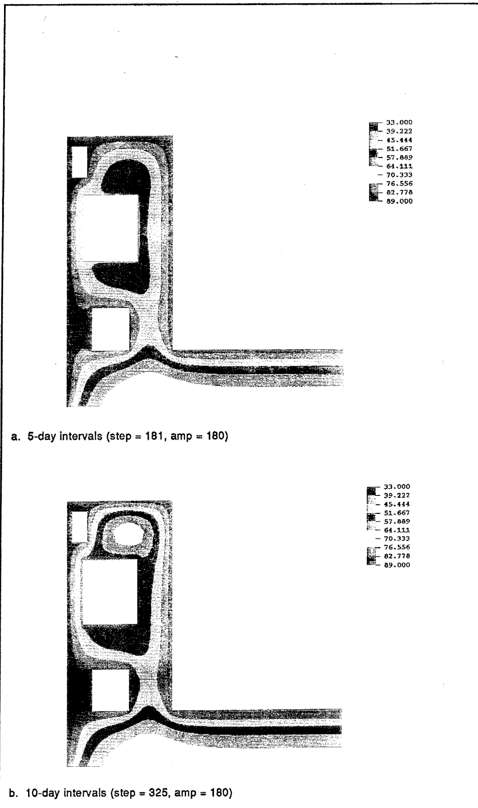
Figure 65. Temperature contours at 180 days after start of construction (Continued)
