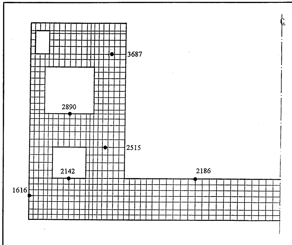
Figure 14. Nodes used to describe the thermal behavior of the monolith
