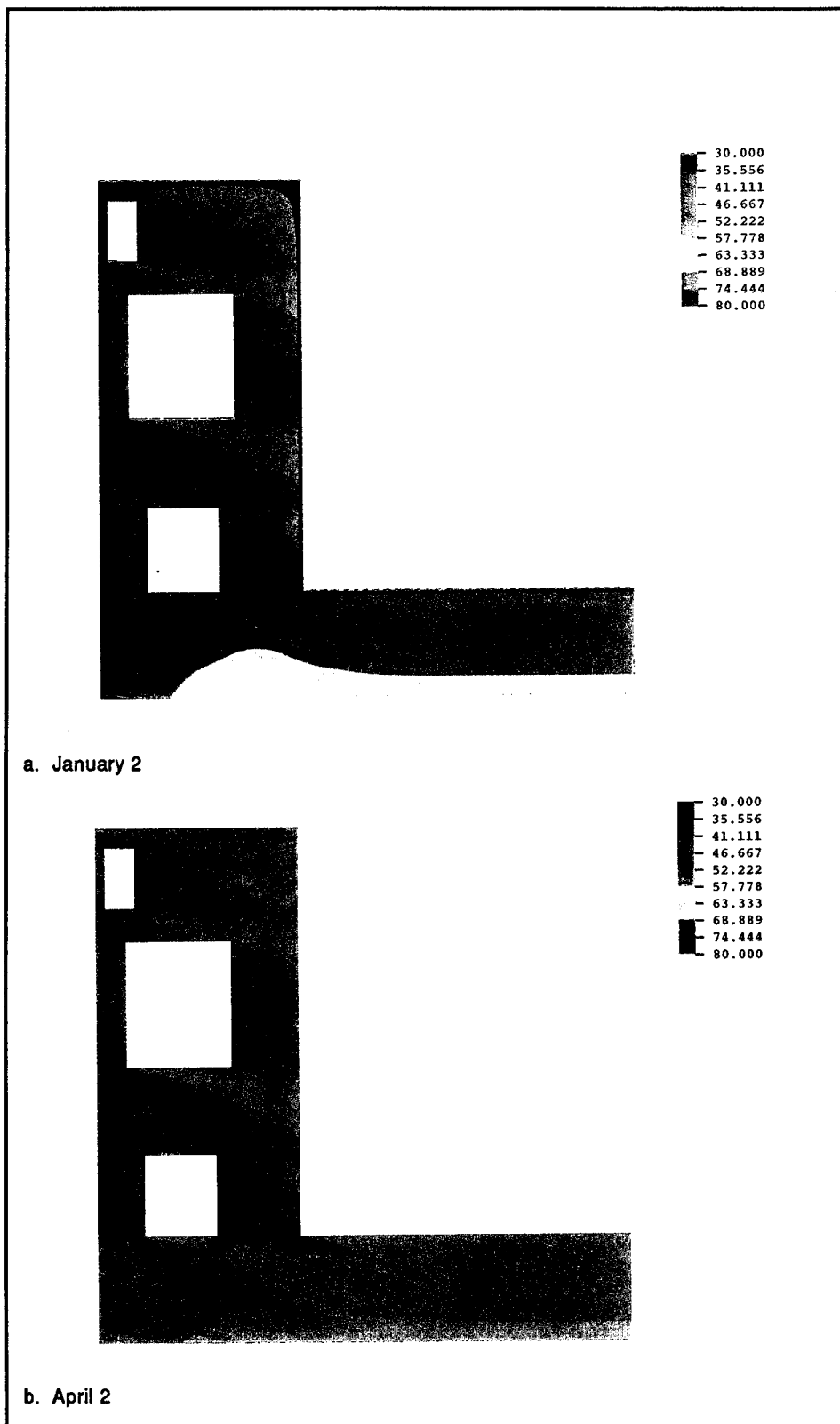
Figure 13. Temperature contours for 360 days after start of construction (step = 217, amp = 360) (Continued)
