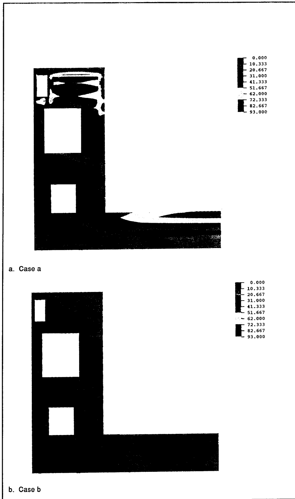
Figure 112. Cracking potential contours at 540 days after start of construction (step = 227, amp = 540) (Continued)
