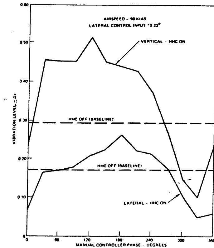
Figure 11. Variation of 4P vibration with input phase at 90 KIAS (From Ref. 1)
