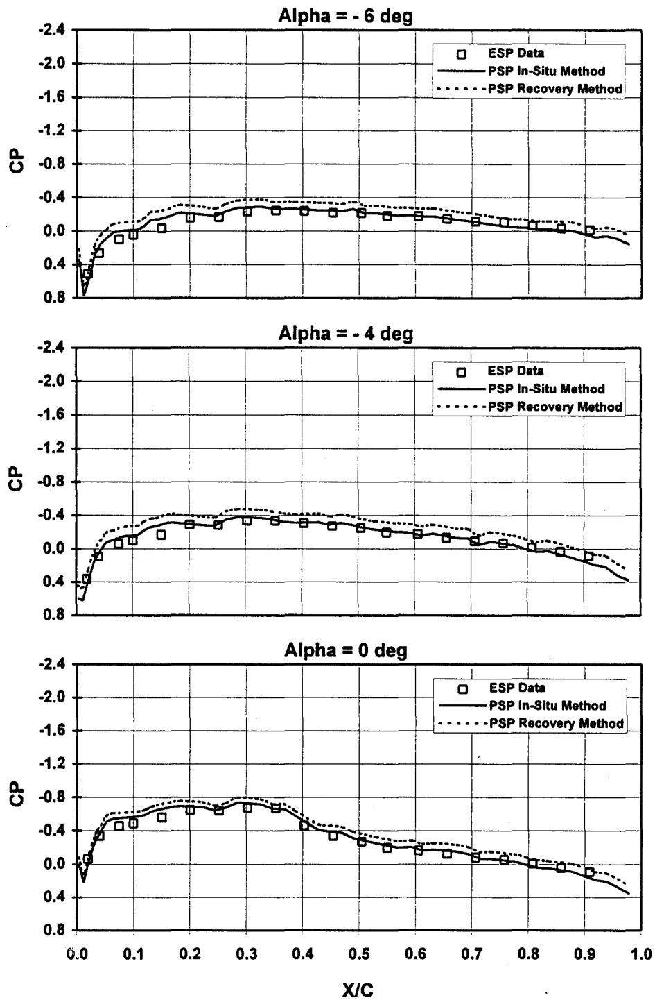
e. Mach = 0.85, P_T = 2,000 psfa, T_T \approx 120^\circ\text{F} Figure 11. Continued.
