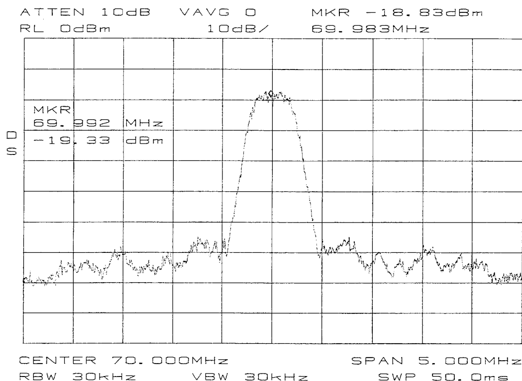
Figure 5. Output Spectrum from CM701 modem with 384-kbps, unencoded BPSK.
