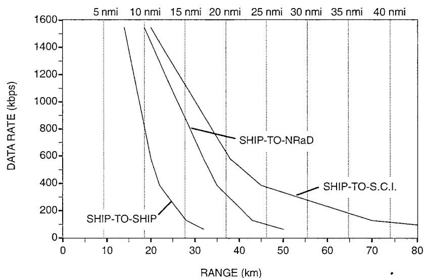
Figure 18. Estimated range for an uncoded QPSK signal with a fade margin of 15 dB, carrier frequency of 300 MHz, and standard propagation conditions (i.e., K=4/3 ). Estimates based on a minimum RSL = –82 dBm for BER = 10 –6 .
