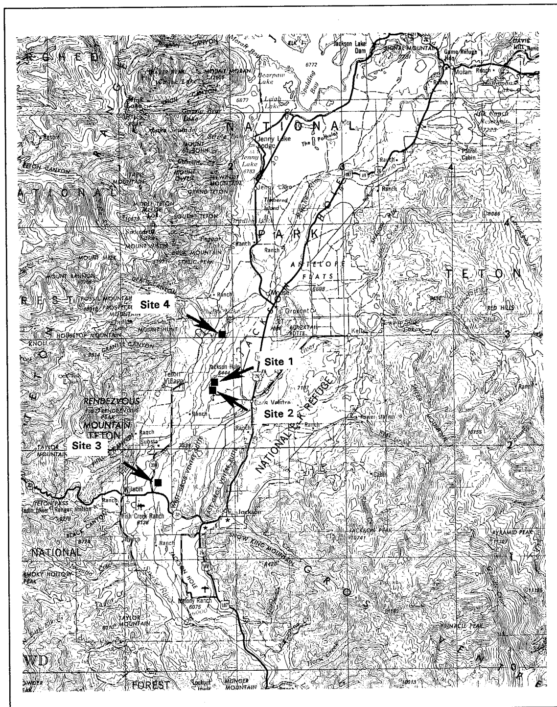
Figure 1. Location of Snake River dendrochronology study areas in Jackson Hole (Continued)
