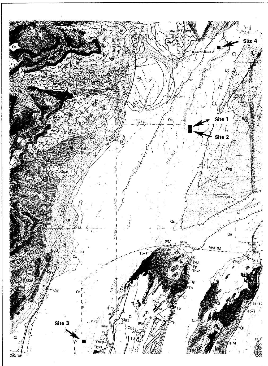
Figure 3. Geology of Snake River dendrochronology study areas (Sheet 1 of 3)
