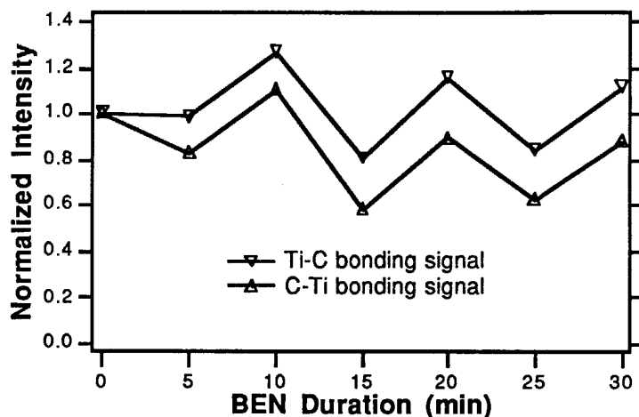
Figure 2. The normalized photoelectron intensity for the C-Ti and Ti-C bonding as a function of BEN duration.
