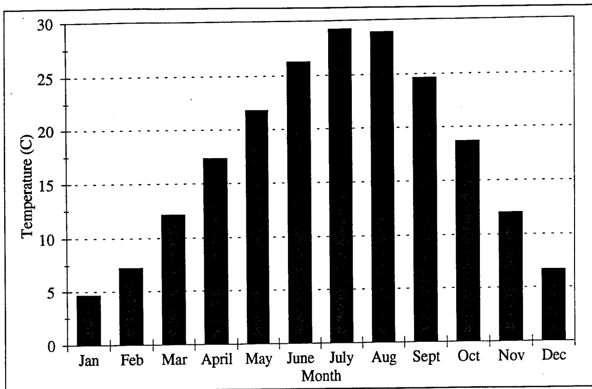
Figure 4. Average monthly temperatures at Pilot Point, TX
