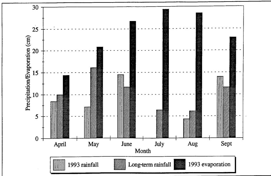
Figure 7. Total monthly precipitation and evaporation for study period, as measured at Pilot Point
