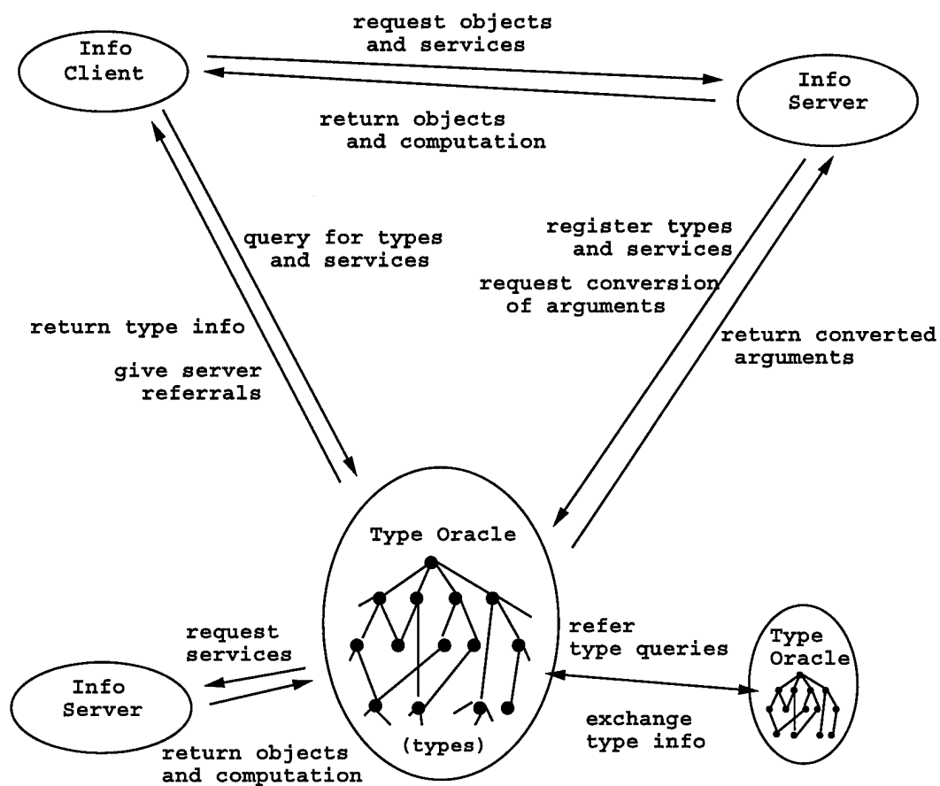
Figure 1: Agent interaction in TOM
