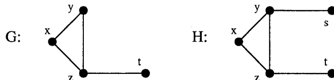
Figure 10. In G x is simple; In H x is not simple.
