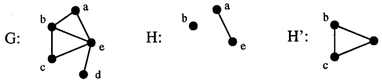
Figure 3. A graph G , subgraph H , and induced subgraph H' .
