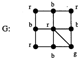
Figure 5. A 3-coloring of G ; \chi(G) = 3 .
