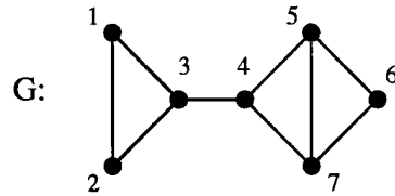
Figure 8. \alpha = (1, 2, 3, 4, 5, 6, 7) is a perfect elimination ordering.
