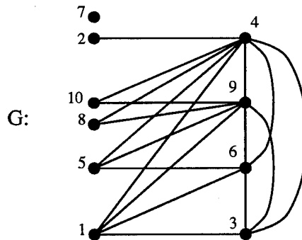
Figure 14. A threshold graph G and a threshold elimination ordering.
