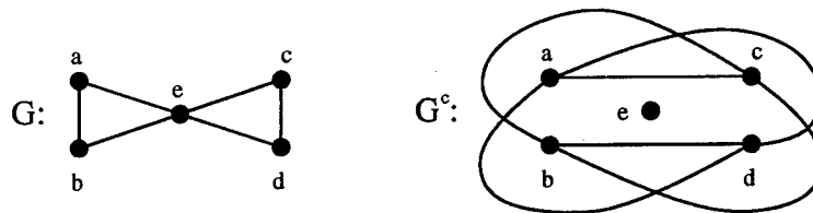
Figure 4. A graph G and its complement G^c .
