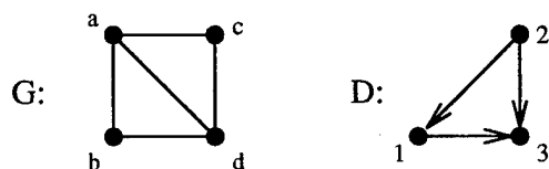
Figure 1. A graph G and a digraph D .
