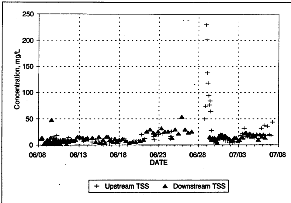
Figure 21. 1993 TSS concentrations
