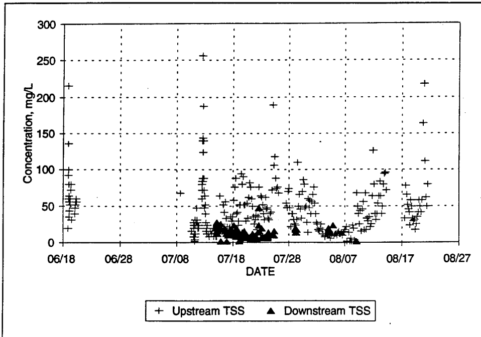
Figure 20. 1992 TSS concentrations
