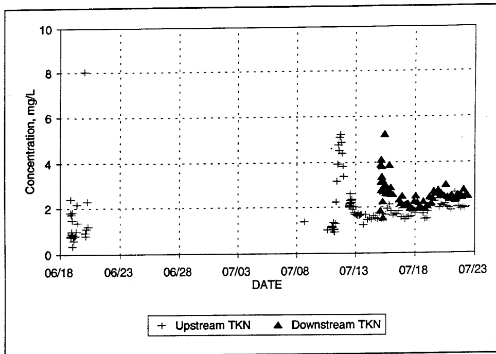
Figure 24. 1992 TKN concentrations
