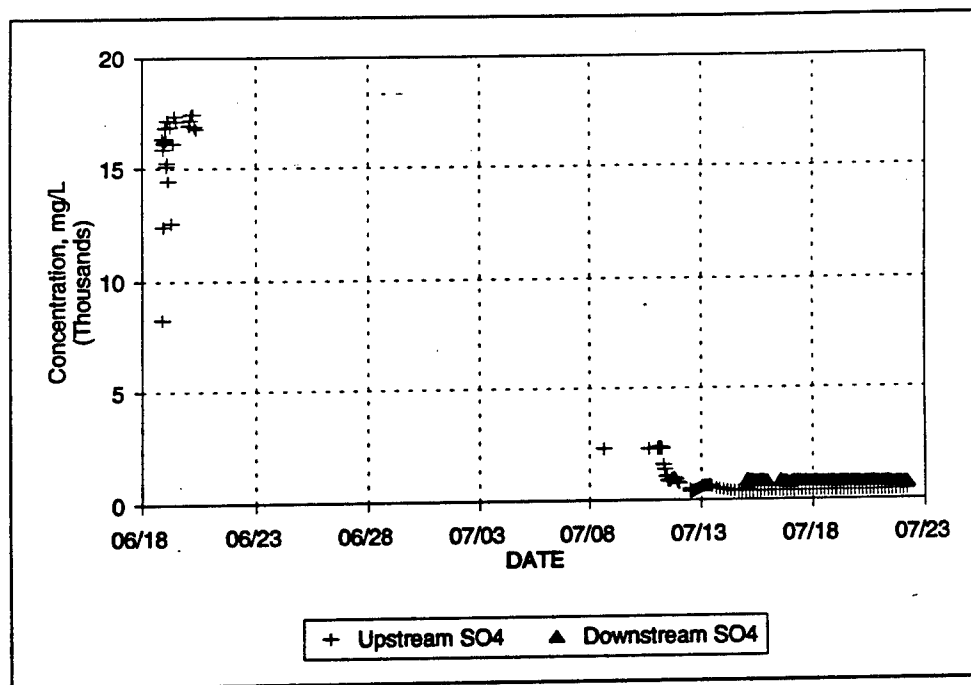
Figure 27. 1992 SO 4 concentrations
