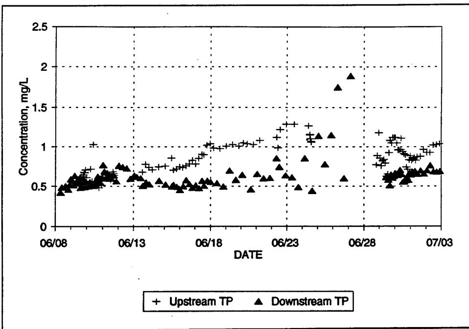
Figure 23. 1993 TP concentrations
