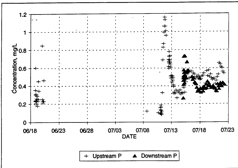
Figure 22. 1992 TP concentrations
