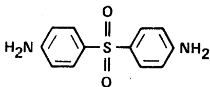
4, 4' DIAMINODIPHENYL SULFONE (19.4%)
