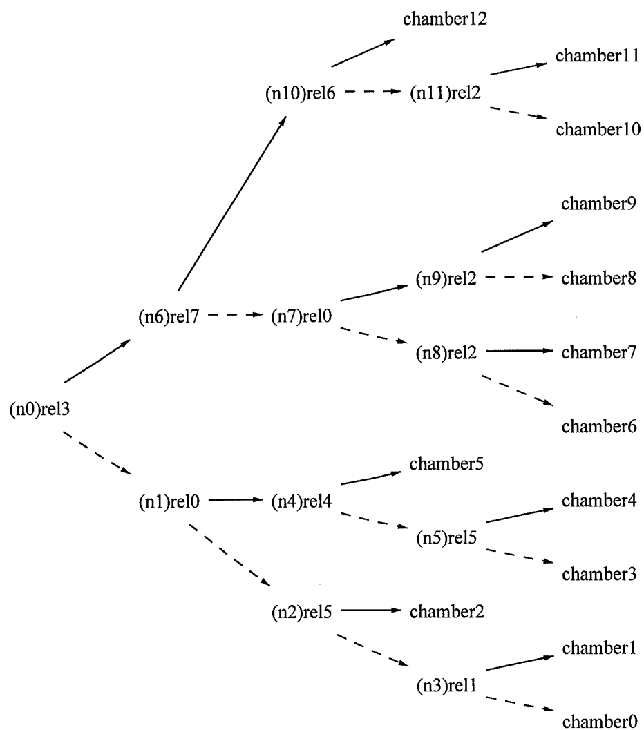
Figure B.1: Decision tree for 3 by 3 contingency tables.
