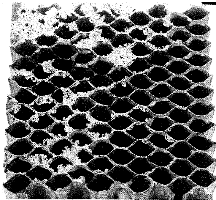
Figure 12. Failed Flatwise Tension Test Specimen (NR 150 Graphite Laminates/HRH Polyimide Honeycomb Core)
