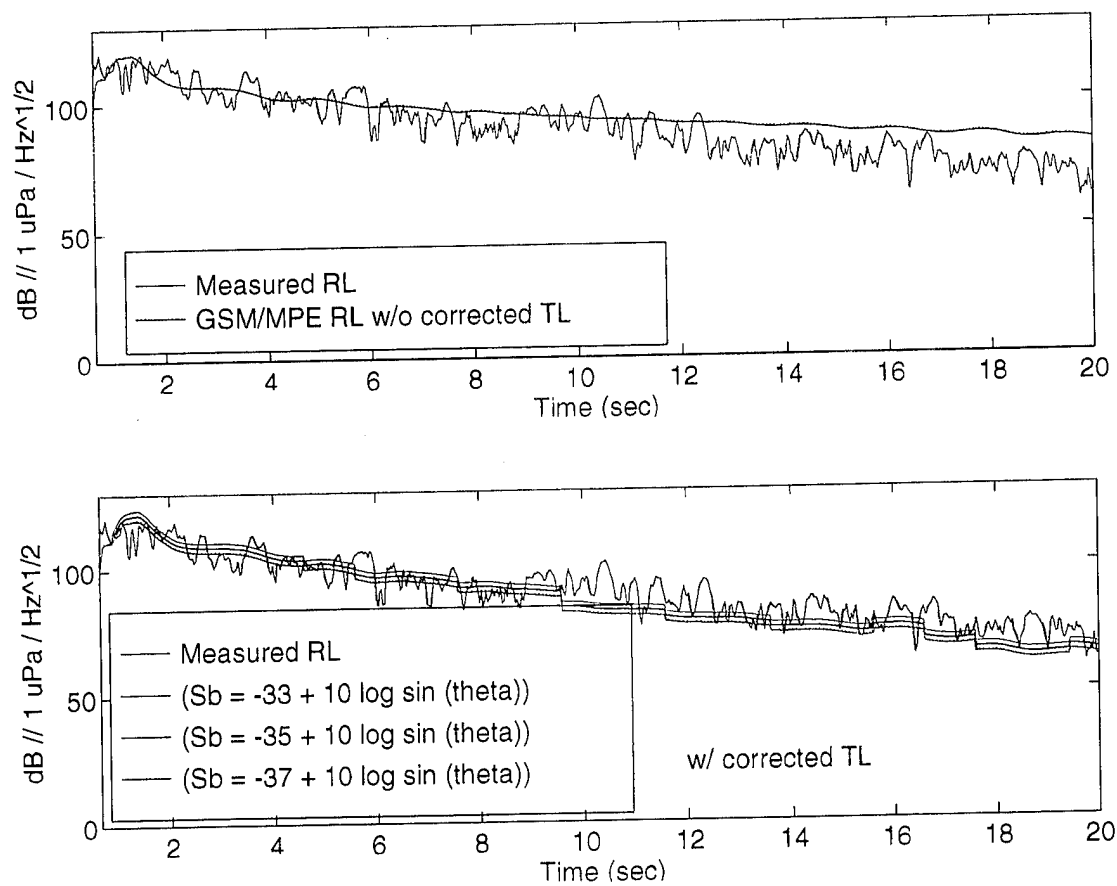
Figure 40d. Same as Figure 40a except for ping 60, beam 24.
