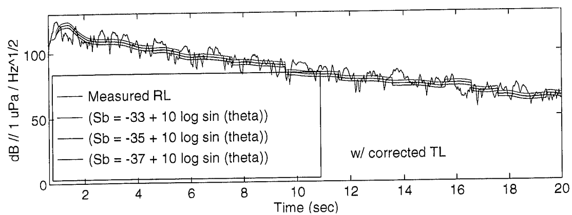
Figure 38c. Same as Figure 38a except for ping 40, beam 1.
