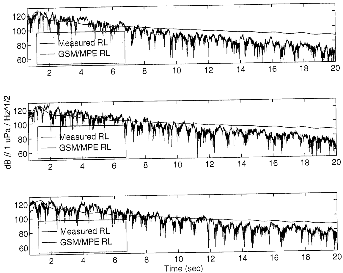
Figure 30a. Measured RL and GSM/MPE RL using the NPS model for ping 30, beam 1 (top panel), ping 30, beam 3 (center panel), and ping 30, beam 5 (bottom panel).
