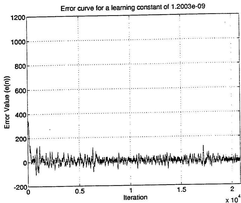
Figure 3: Error curve for a learning constant of 1.2003e-9
