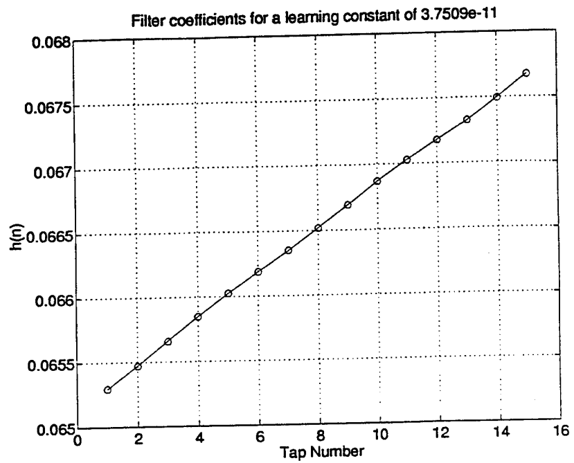
Figure 2: Coefficient vector for a learning constant of 3.7509e-11.
