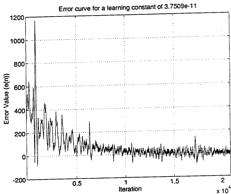
Figure 1: Error curve for a learning constant of 3.7509\text{e-}11
