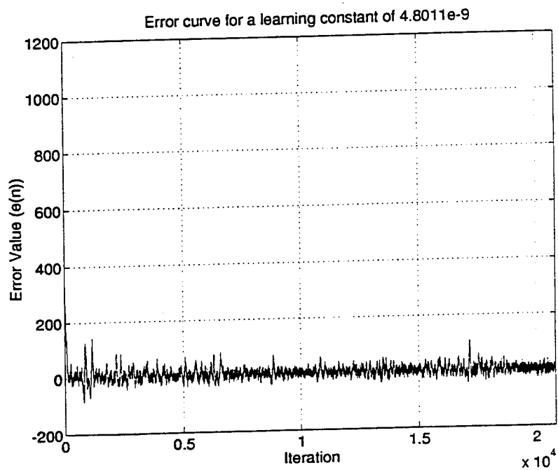
Figure 5: Error curve for a learning constant of 4.8011e-9
