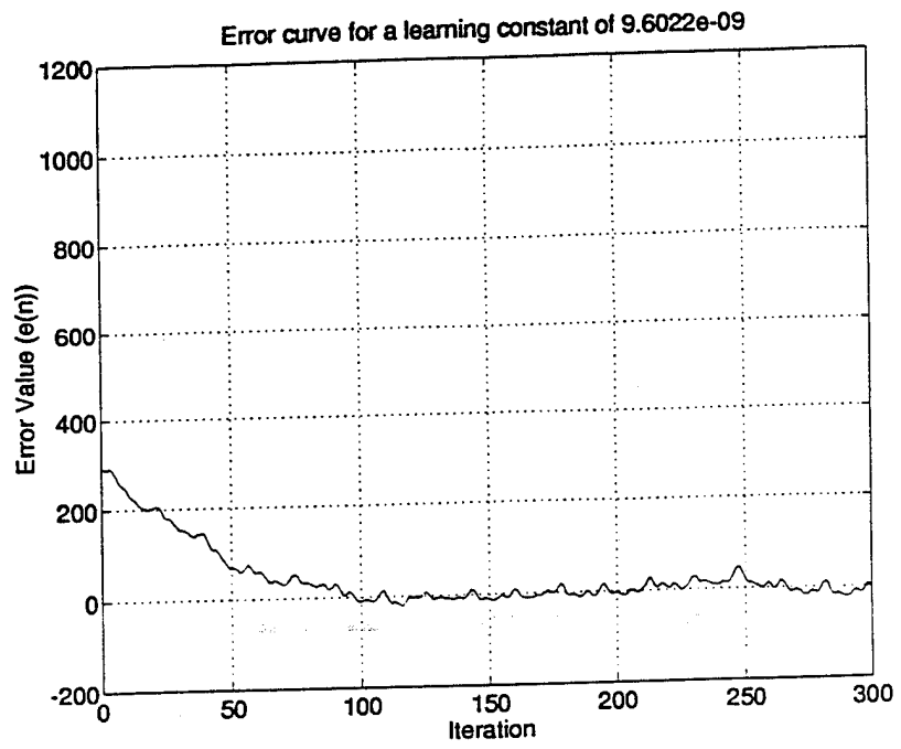
Figure 8: Error curve for a learning constant of 9.6022e-9
