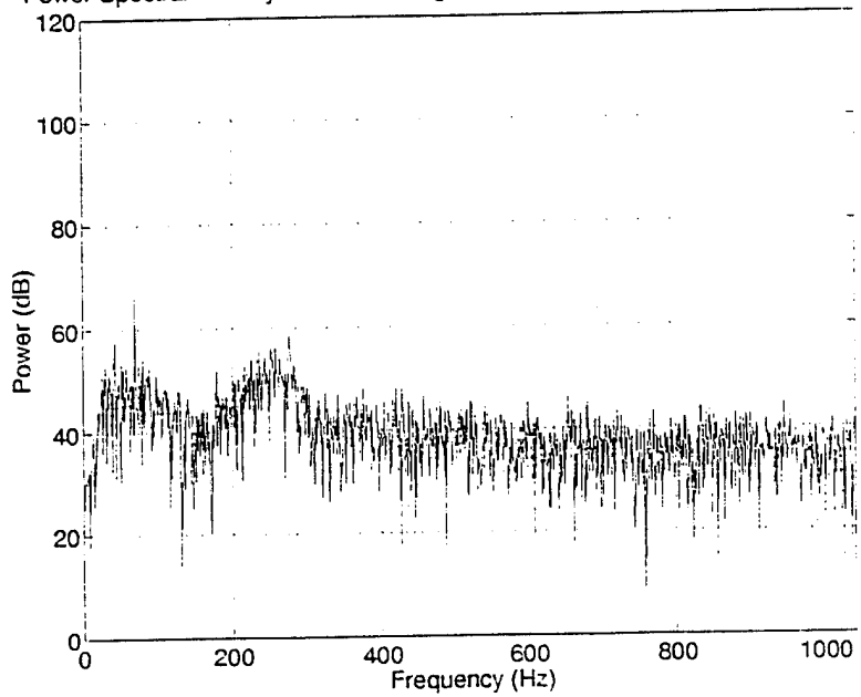
Figure 38: Power spectral density of processed signal 25
