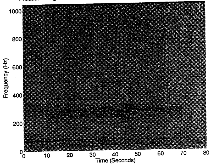
Figure 37: Spectrogram of processed signal 25
