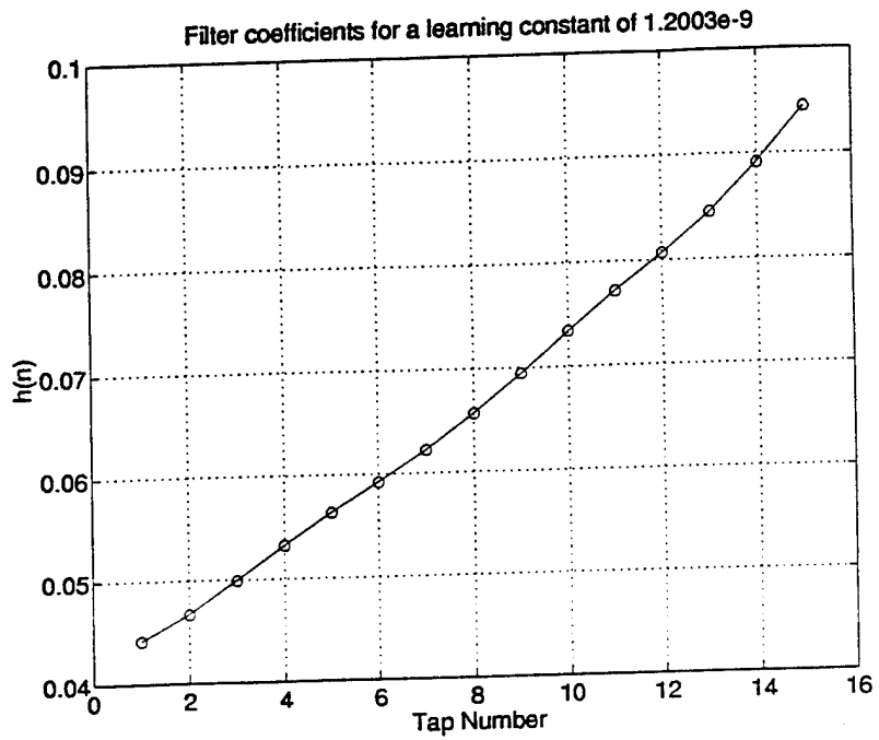
Figure 4: Coefficient vector for a learning constant of 1.2003e-9
