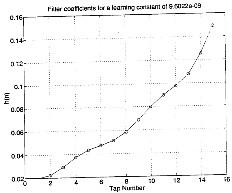
Figure 9: Coefficient vector for a learning constant of 9.6022e-9
